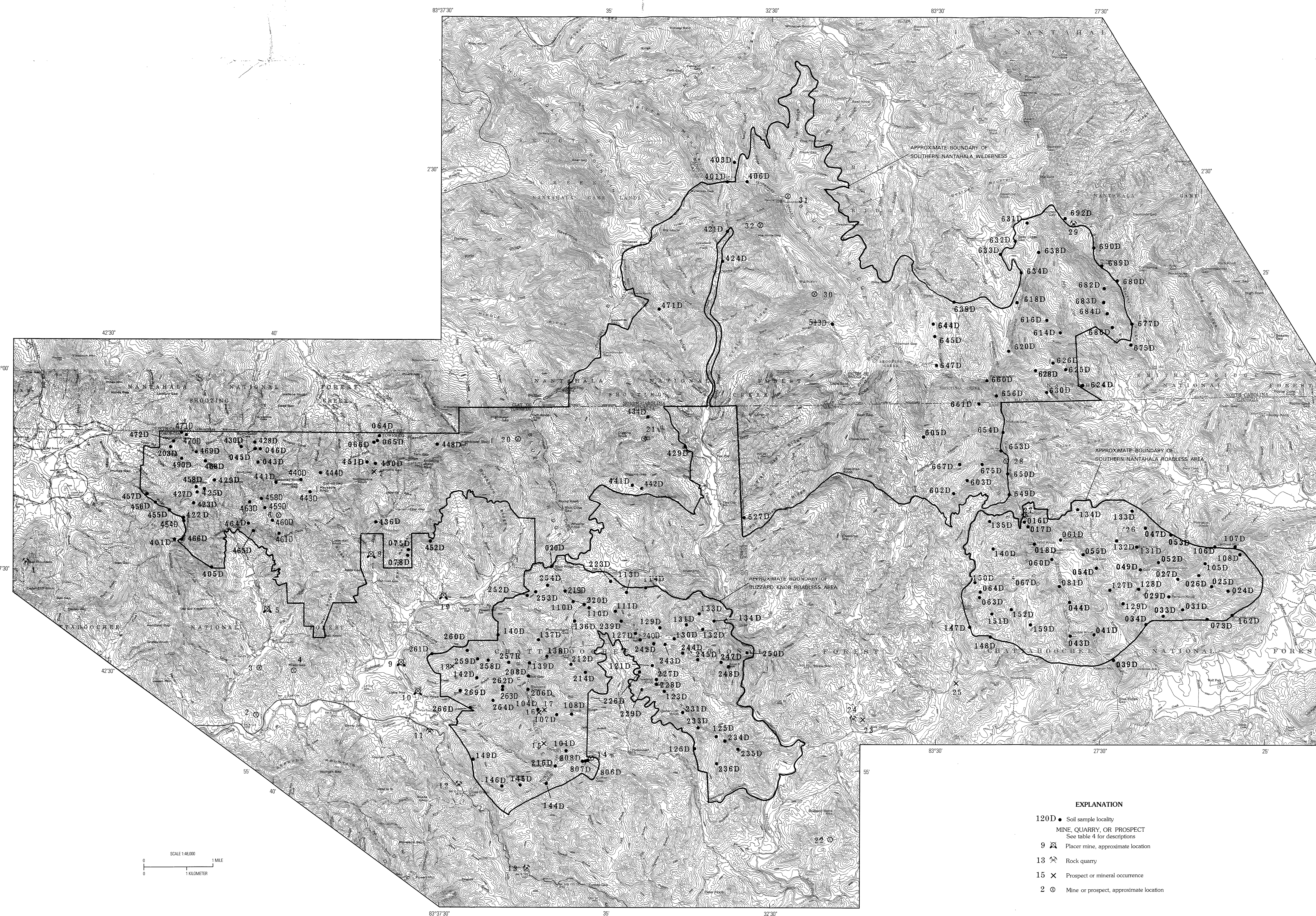
C. SOIL SAMPLE LOCALITY, MINE, PROSPECT, AND MINERAL OCCURRENCE MAP OF THE SOUTHERN NANTAHALA WILDERNESS AND ADJACENT ROADLESS AREAS
