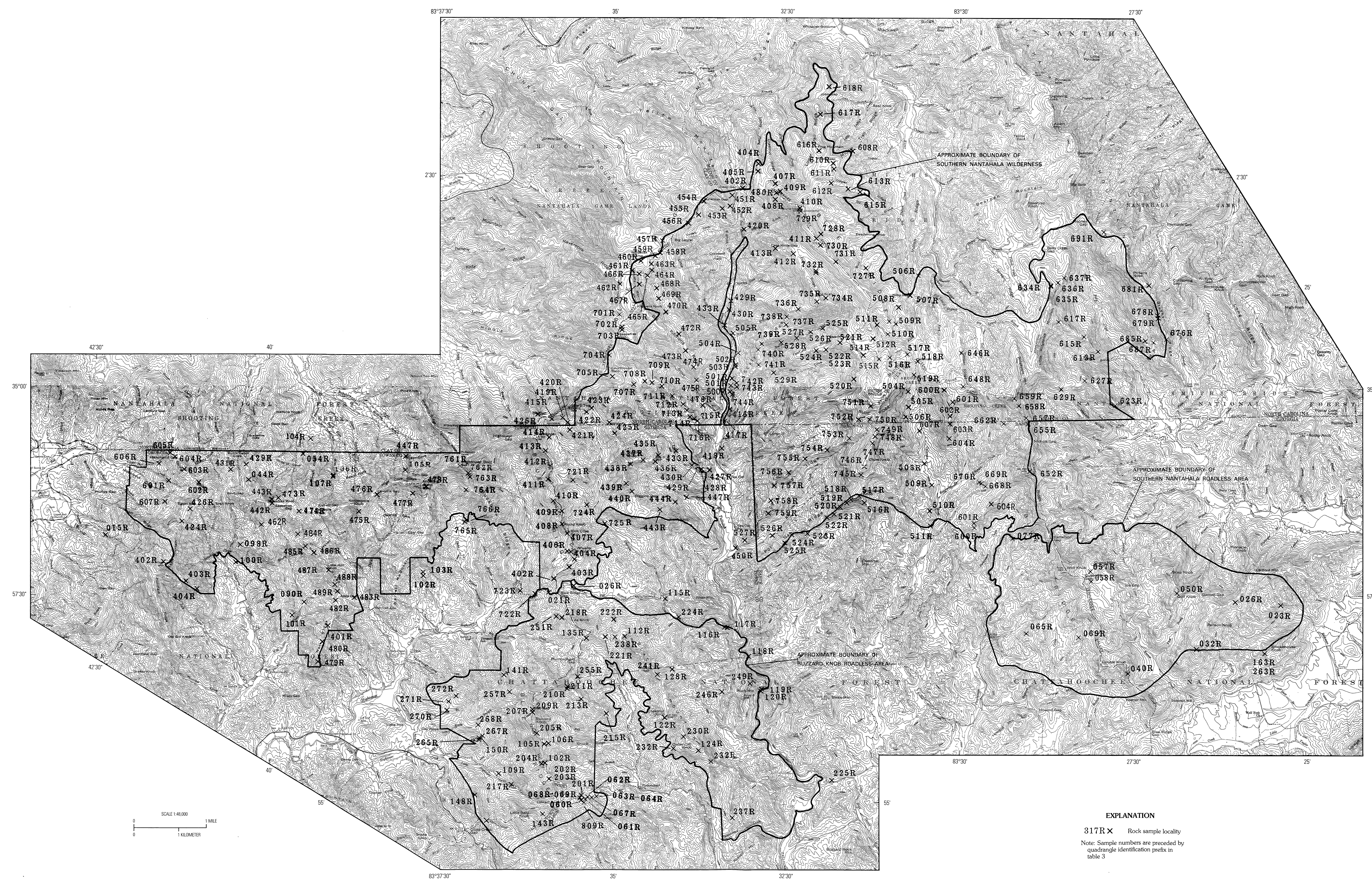
B. ROCK SAMPLE LOCALITY MAP OF THE SOUTHERN NANTAHALA WILDERNESS AND ADJACENT ROADLESS AREAS
