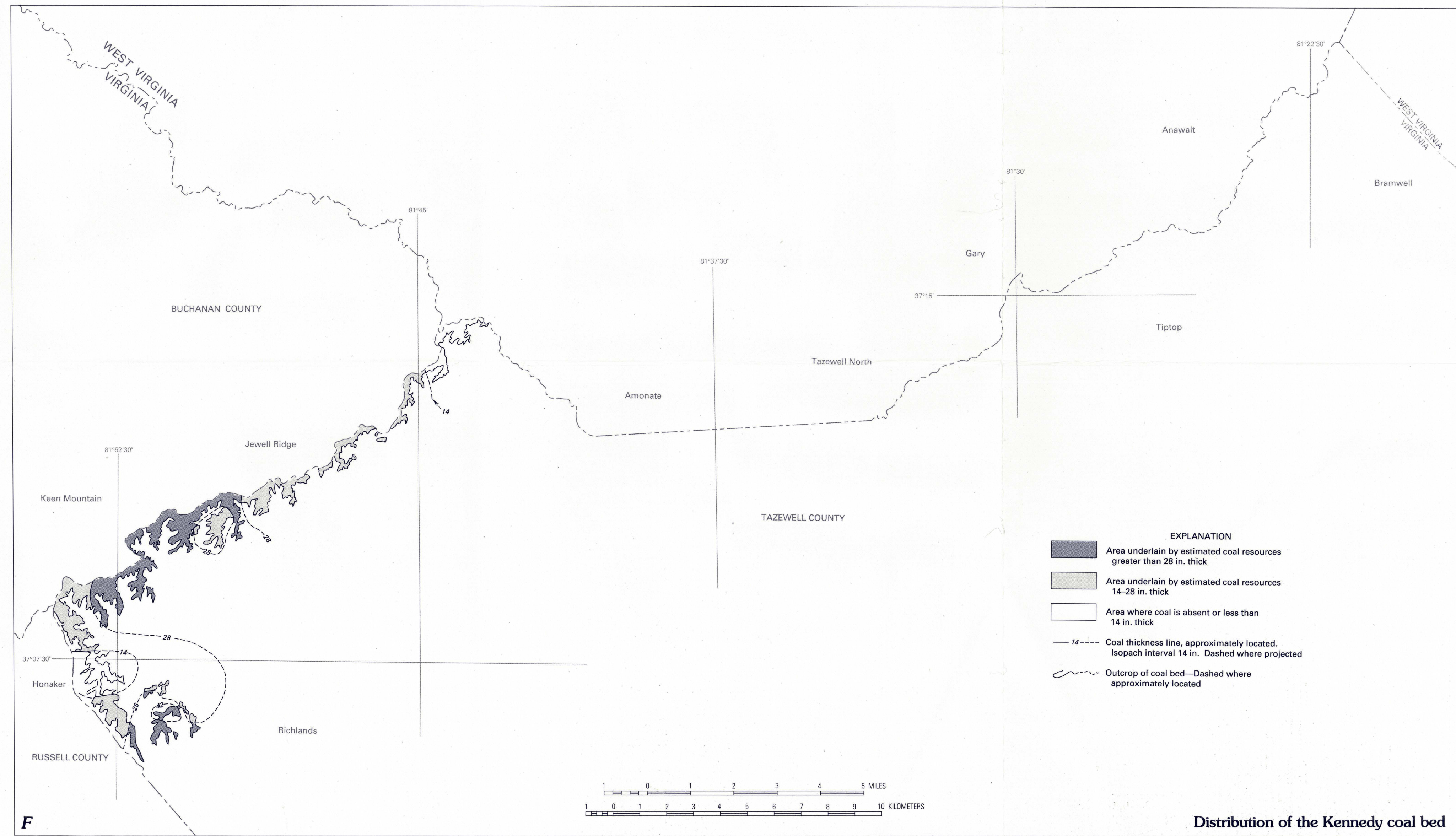
DISTRIBUTION OF THE MIDDLE SEABOARD, UPPER SEABOARD, TILLER, JAWBONE, JEWELL, AND KENNEDY COAL BEDS
