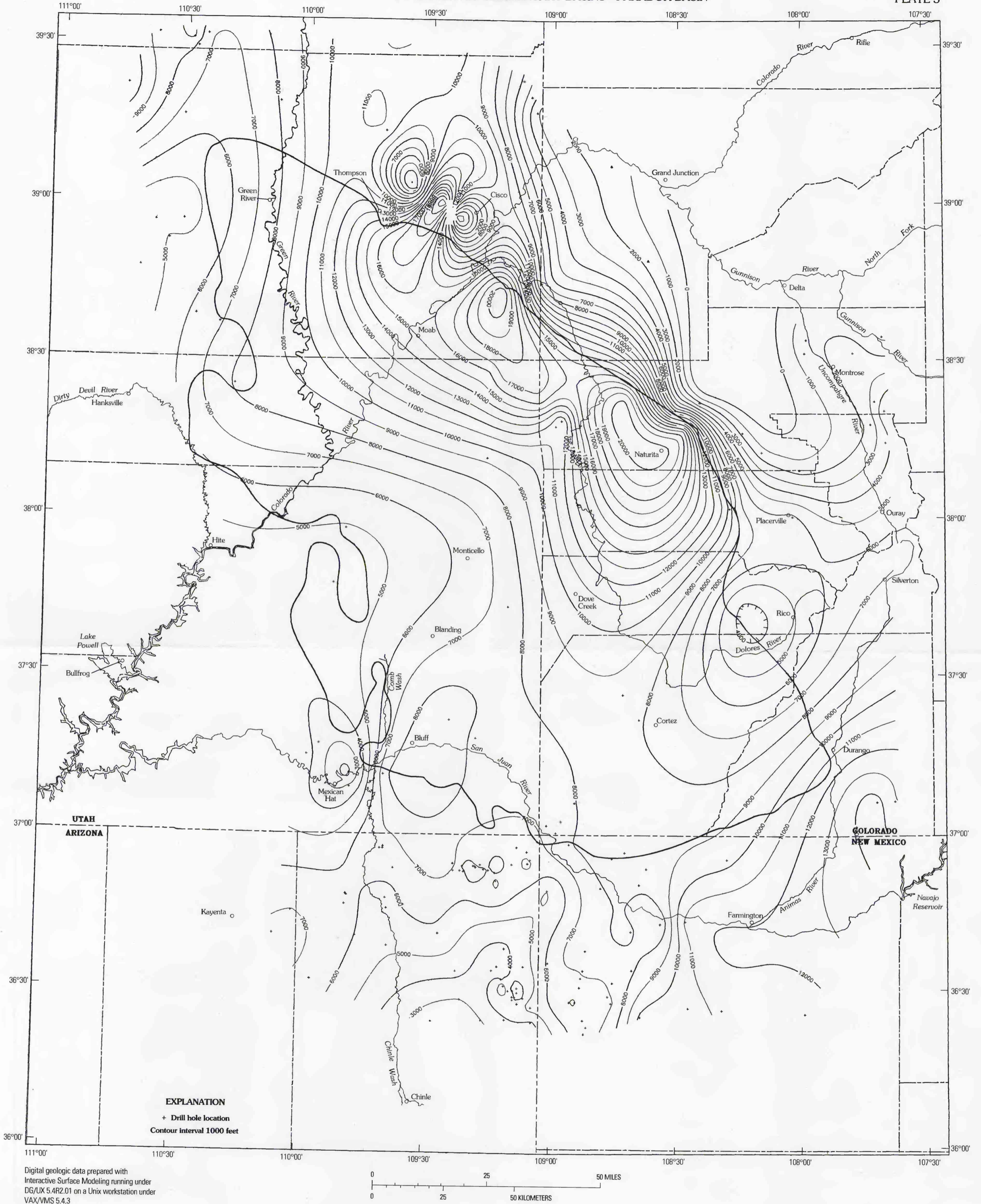
MAP SHOWING THICKNESS OF SEDIMENTARY ROCKS, PARADOX BASIN AND ADJACENT AREAS, UTAH, COLORADO, ARIZONA, AND NEW MEXICO
