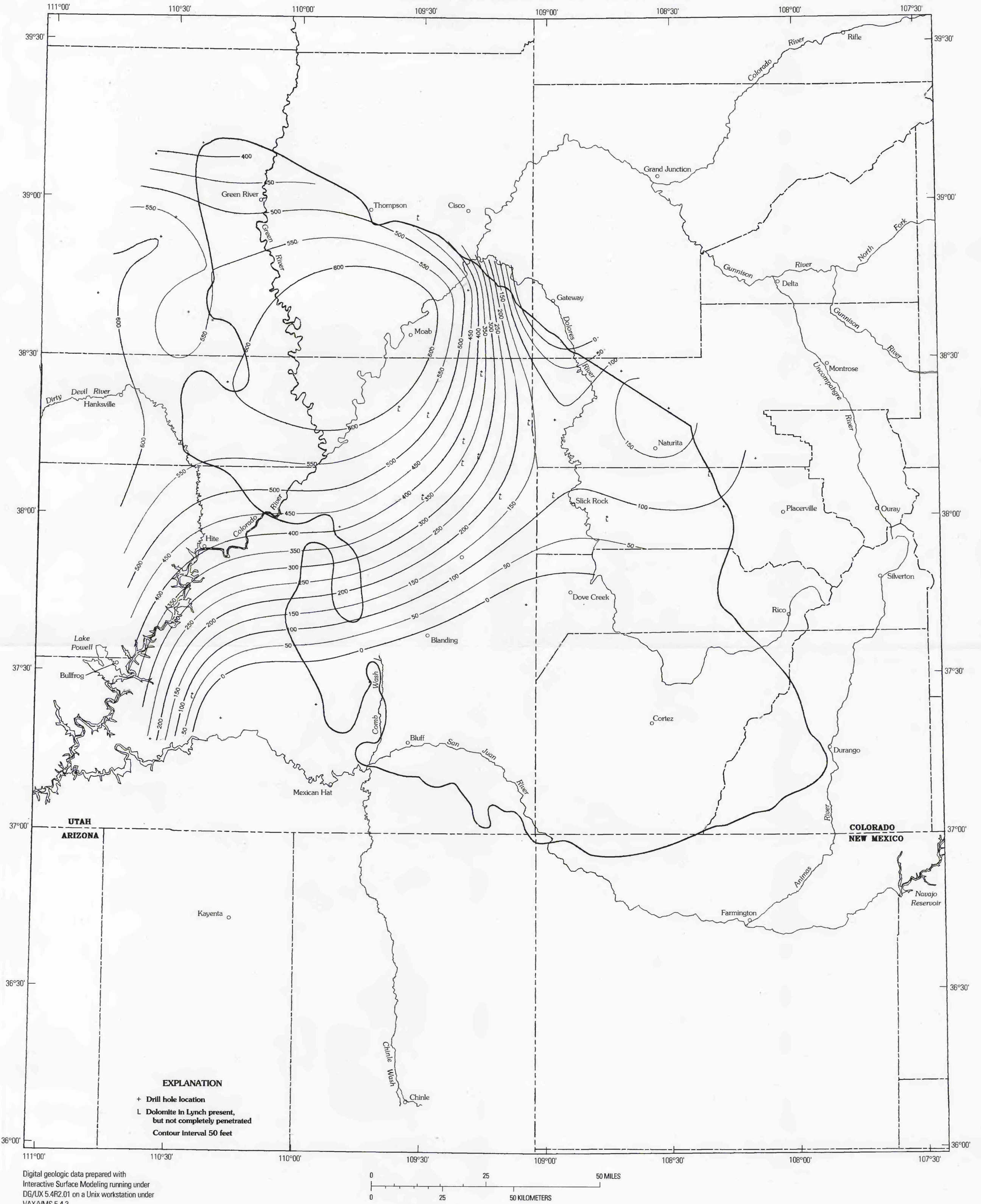
MAP SHOWING THICKNESS OF THE CAMBRIAN LYNCH DOLOMITE, PARADOX BASIN AND ADJACENT AREAS, UTAH, COLORADO, ARIZONA, AND NEW MEXICO
