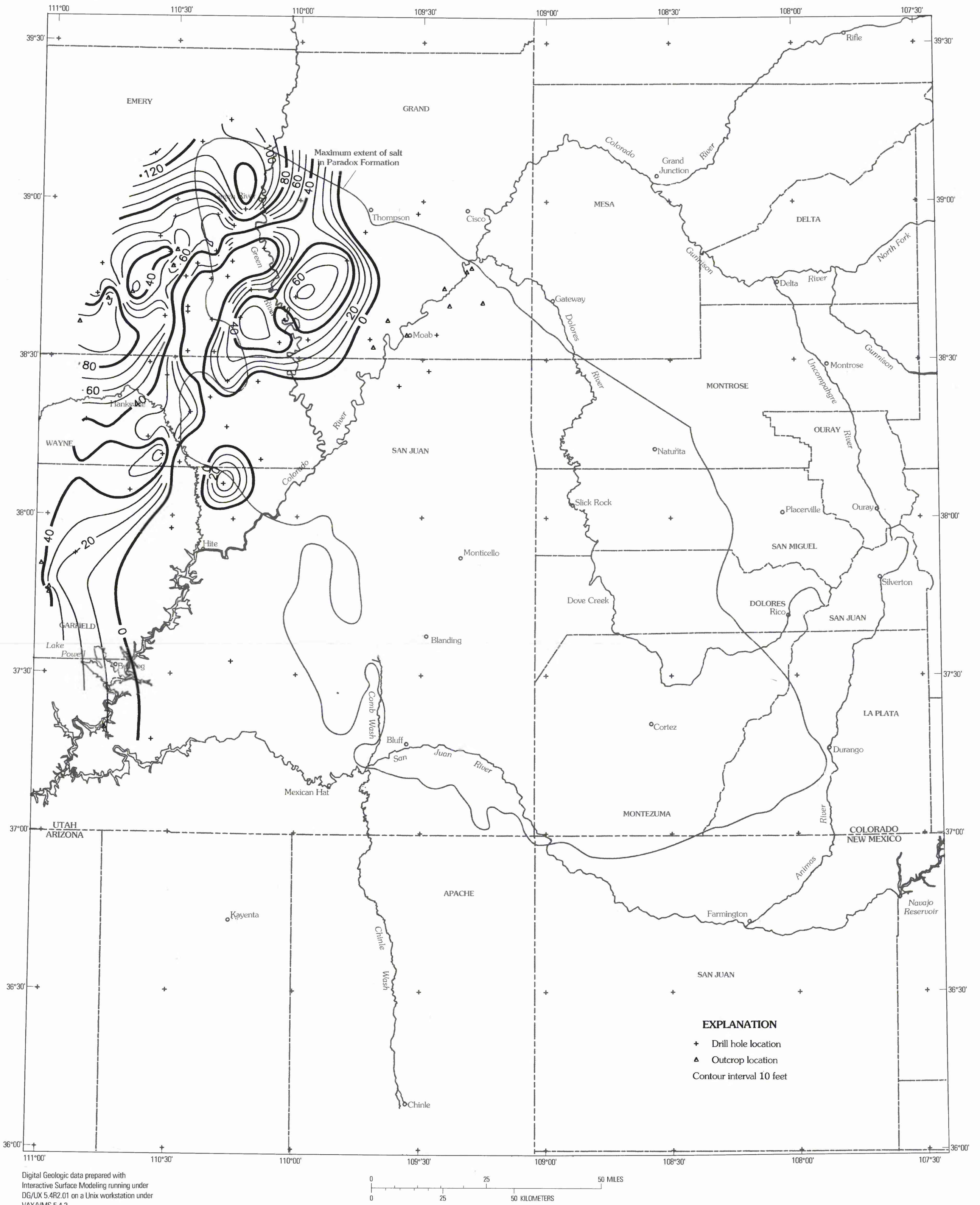
MAP OF THE PARADOX BASIN AND ADJACENT AREAS SHOWING THICKNESS OF THE PERMIAN KAIBAB LIMESTONE
