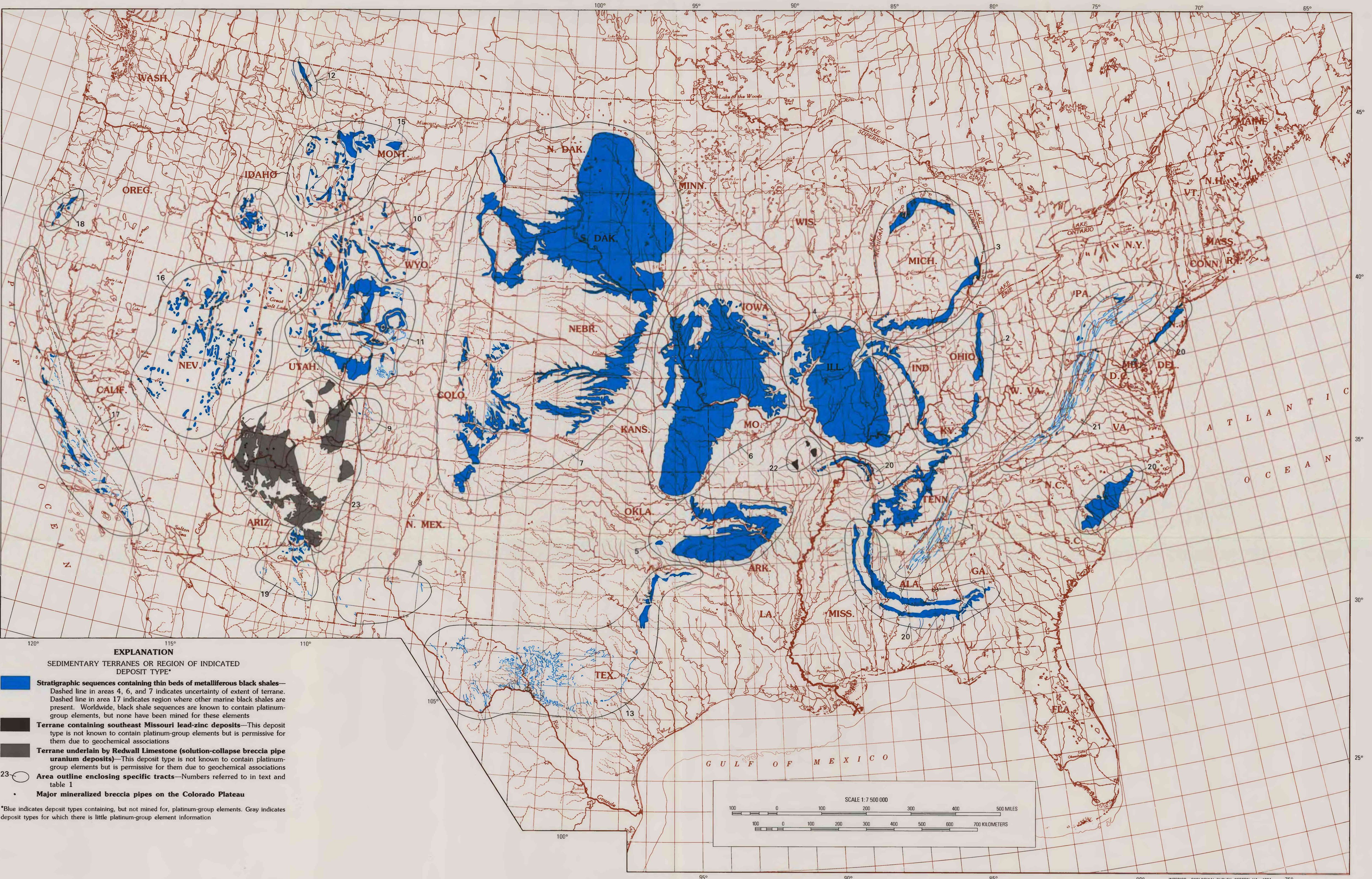
MAP 2. PERMISSIVE TRACTS FOR ORGANIC-CARBON-RICH METALLIFEROUS BLACK SHALES AND SOUTHEAST MISSOURI LEAD-ZINC AND SOLUTION-COLLAPSE BRECCIA PIPE URANIUM DEPOSITS IN THE CONTERMINOUS UNITED STATES
