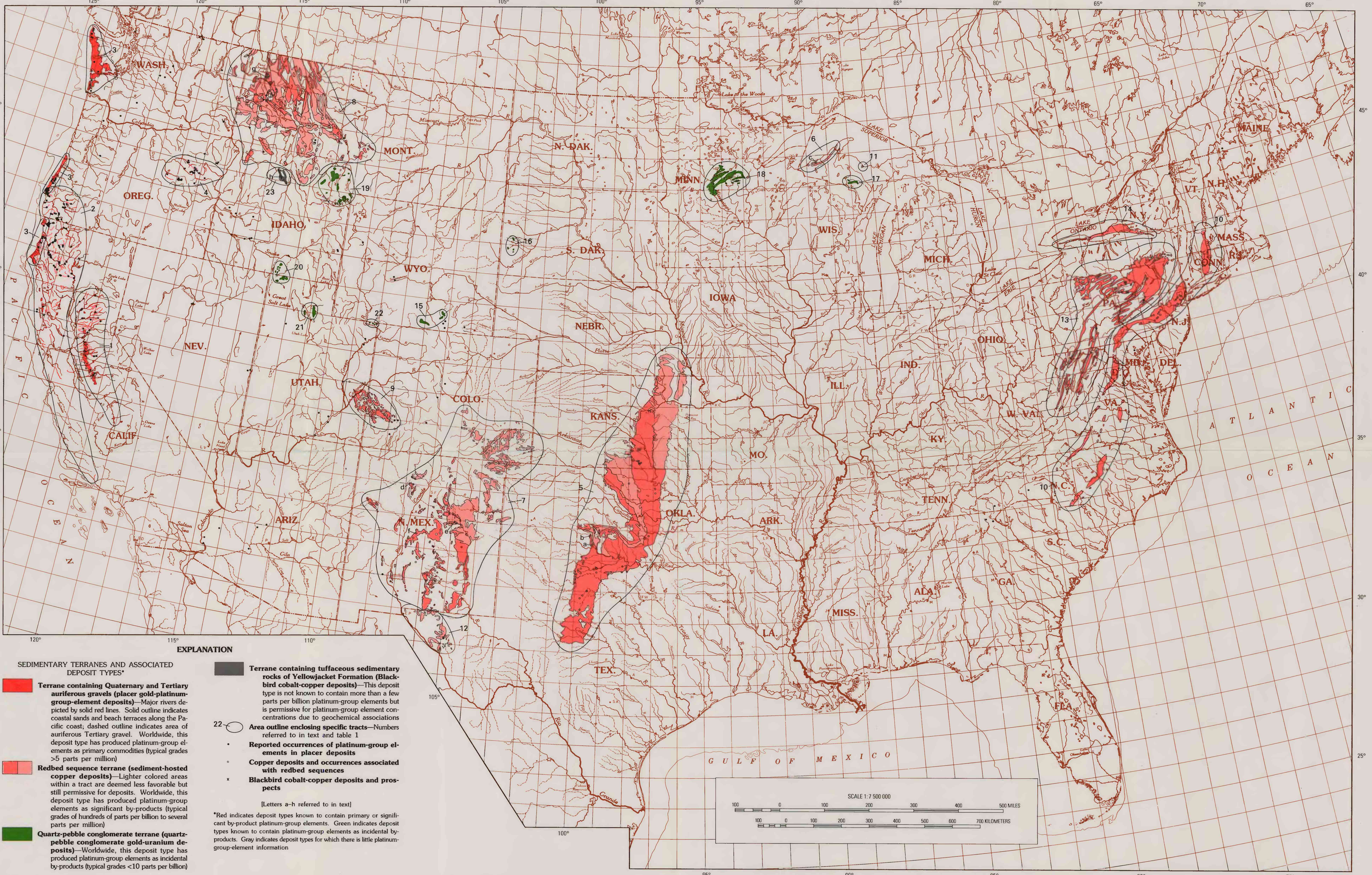
MAP 1. PERMISSIVE TRACTS FOR PLACER; SEDIMENT-HOSTED COPPER, QUARTZ-PEBBLE CONGLOMERATE GOLD-URANIUM, AND BLACKBIRD COBALT-COPPER DEPOSITS AND KNOWN PLATINUM-GROUP-ELEMENT-BEARING PLACER DEPOSITS IN THE CONTERMINOUS UNITED STATES
