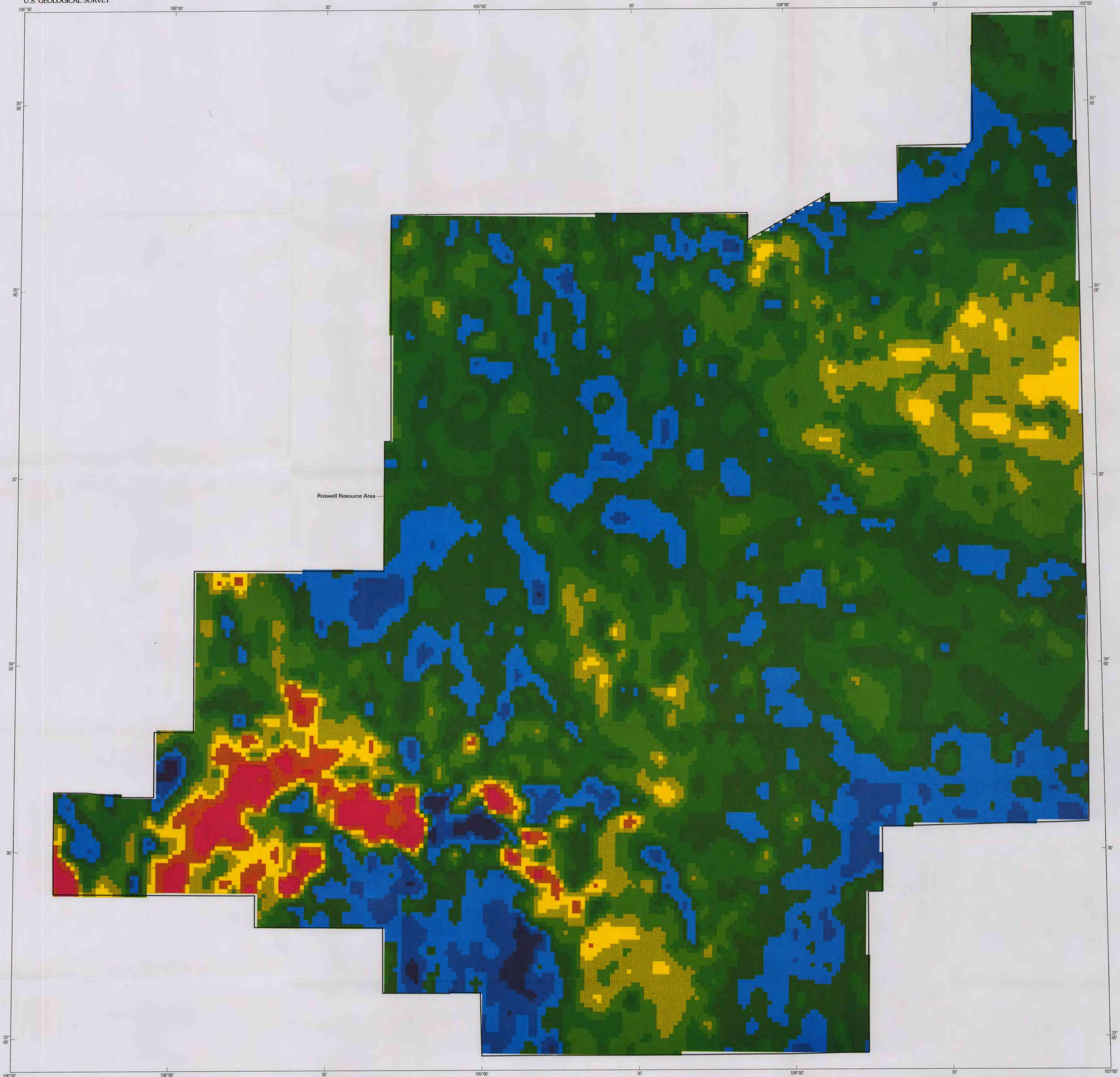
MAP SHOWING APPARENT SURFACE CONCENTRATIONS OF POTASSIUM, ROSWELL RESOURCE AREA, NEW MEXICO
