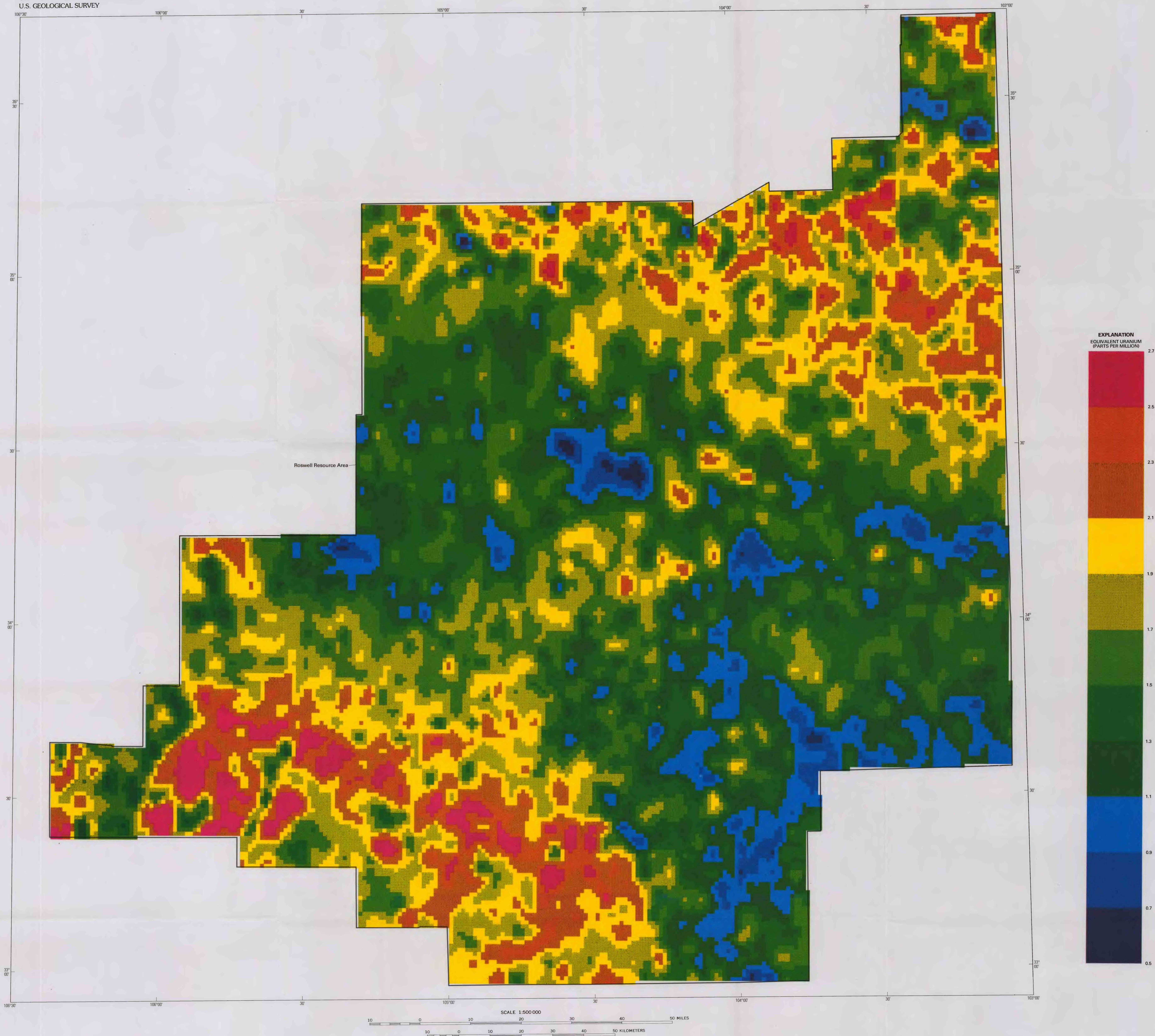
MAP SHOWING APPARENT SURFACE CONCENTRATIONS OF EQUIVALENT URANIUM, ROSWELL RESOURCE AREA, NEW MEXICO
