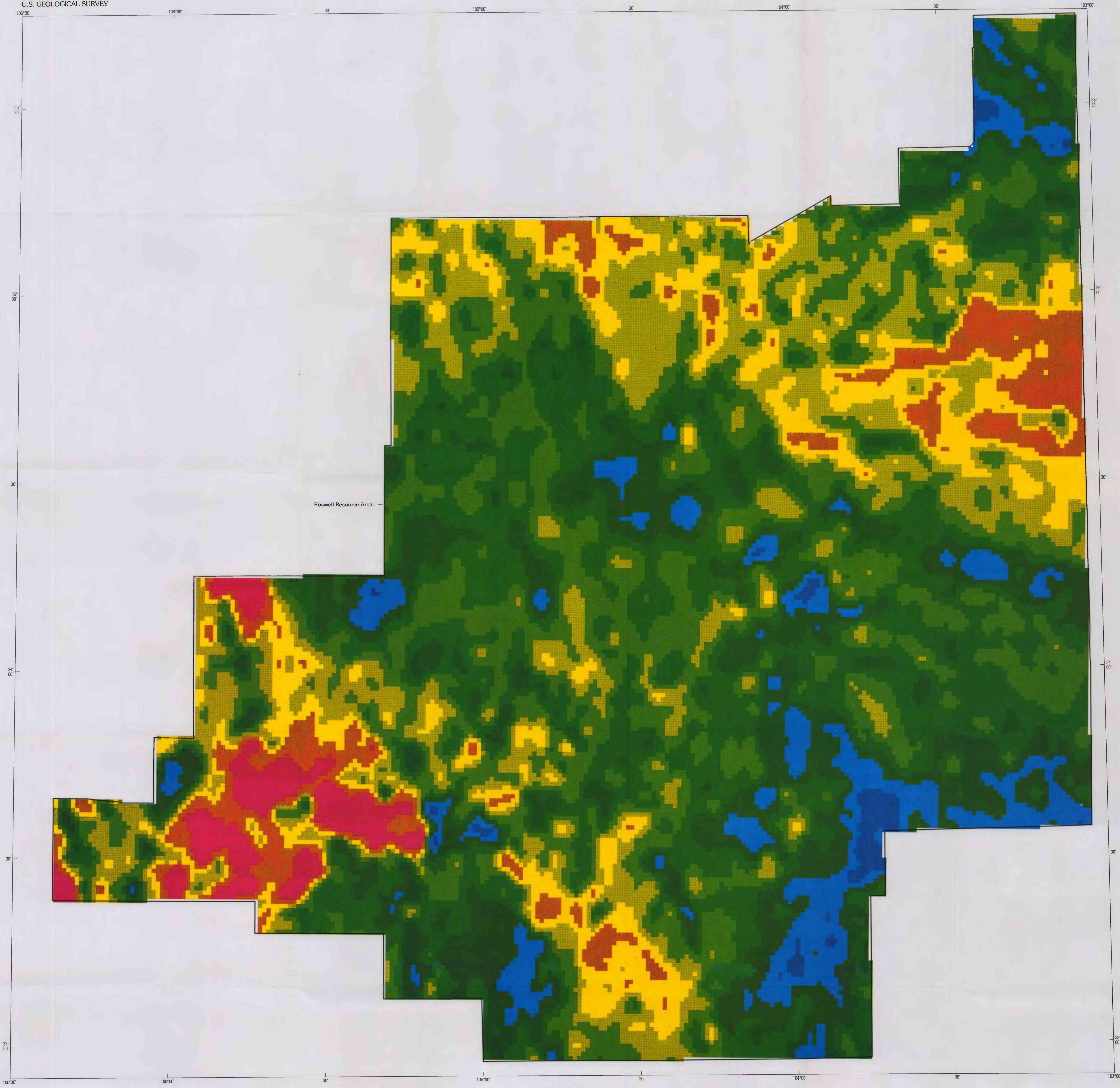
MAP SHOWING APPARENT SURFACE CONCENTRATIONS OF EQUIVALENT THORIUM , ROSWELL RESOURCE AREA, NEW MEXICO
