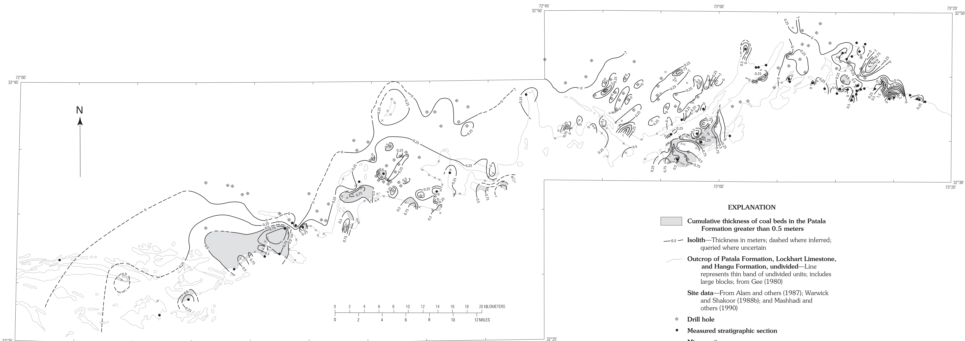
MAP C.—ISOLITH MAP OF CUMULATIVE COAL BED THICKNESS IN THE PATALA FORMATION
