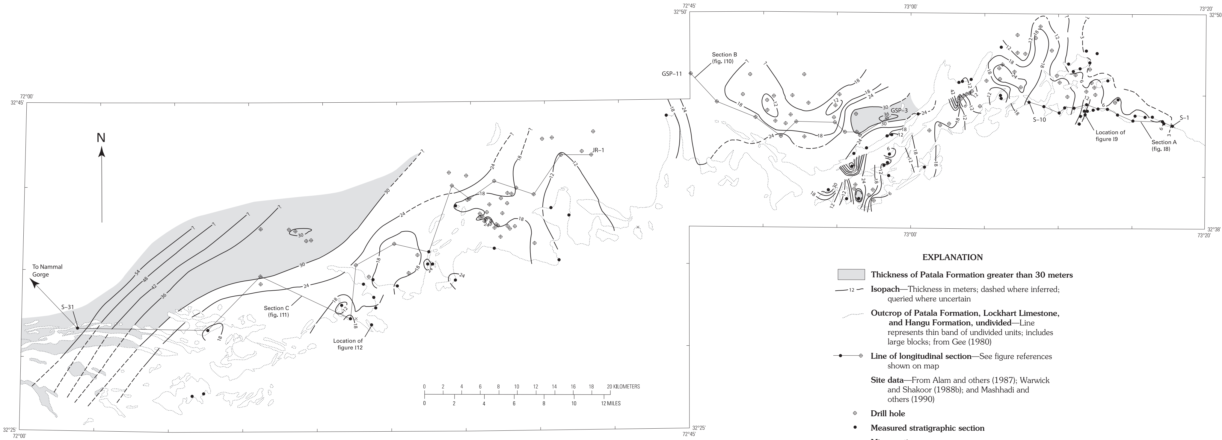
MAP A.—ISOPACH MAP OF THE PATALA FORMATION
