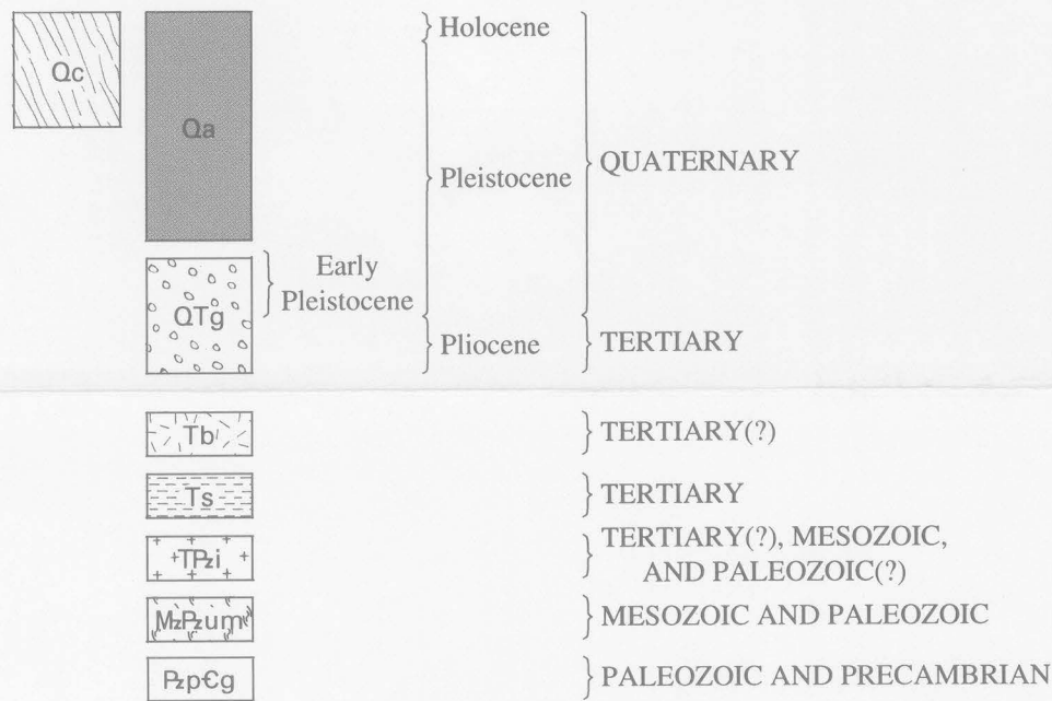
GEOLOGIC MAP SHOWING GOLD PLACERS, FORTY-MILE RIVER AREA, EAGLE QUADRANGLE, ALASKA
