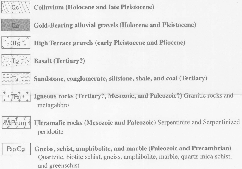
GEOLOGIC MAP SHOWING GOLD PLACERS, FORTY-MILE RIVER AREA, EAGLE QUADRANGLE, ALASKA
