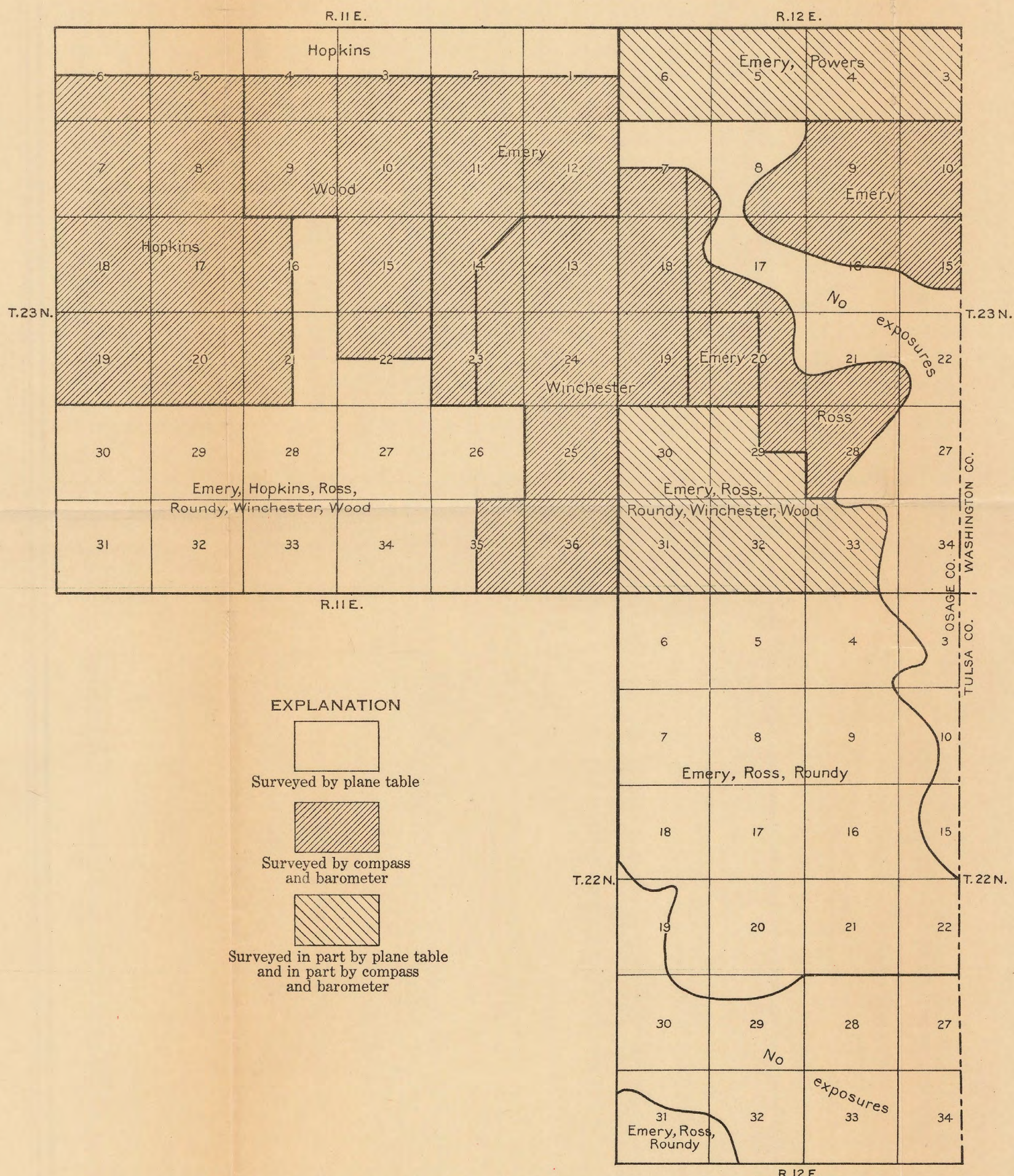
INDEX MAP SHOWING AREAS WORKED BY DIFFERENT GEOLOGISTS AND METHODS USED
