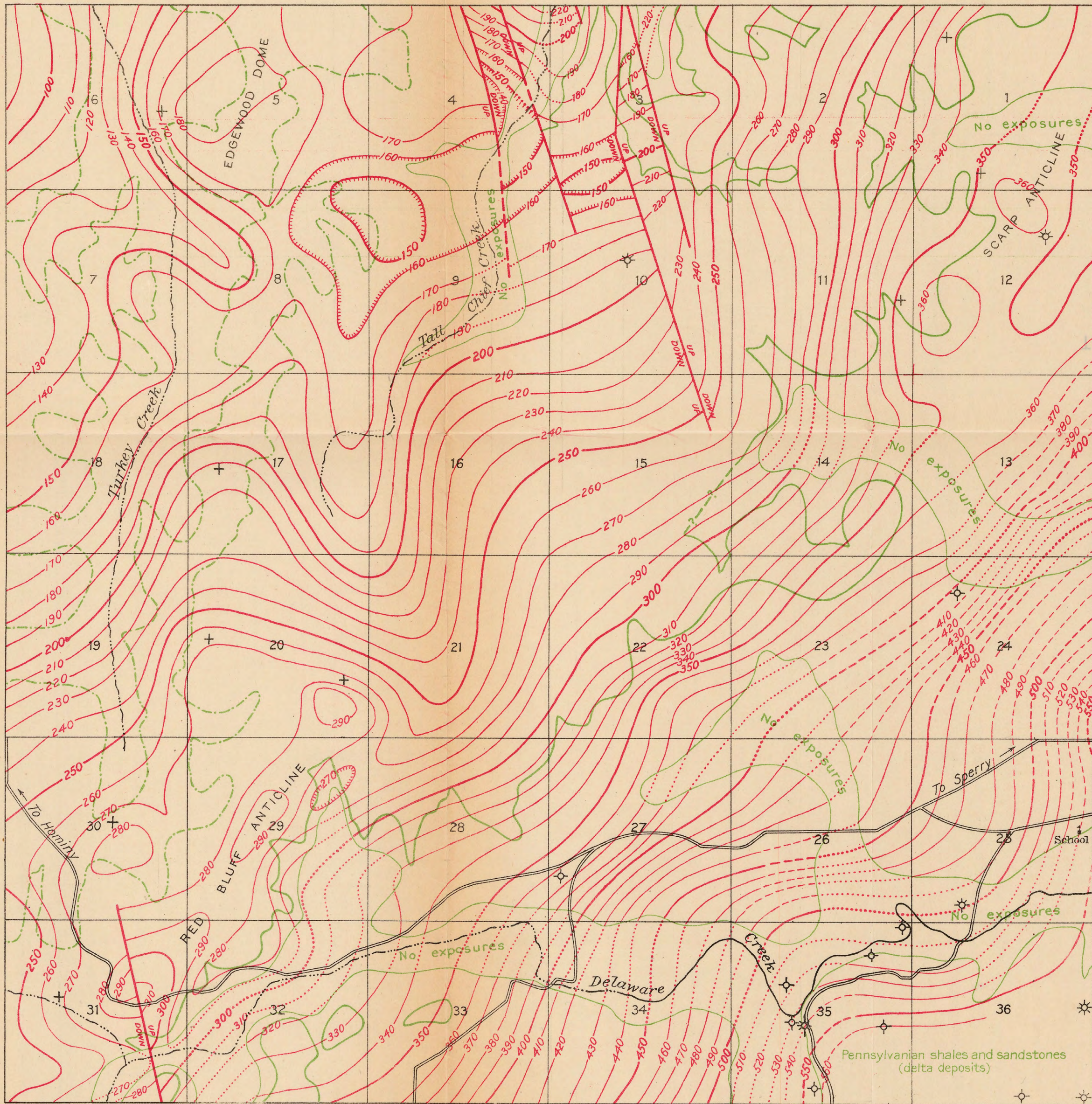
MAP SHOWING GEOLOGIC STRUCTURE OF T. 21 N., R. 11 E., OKLAHOMA
