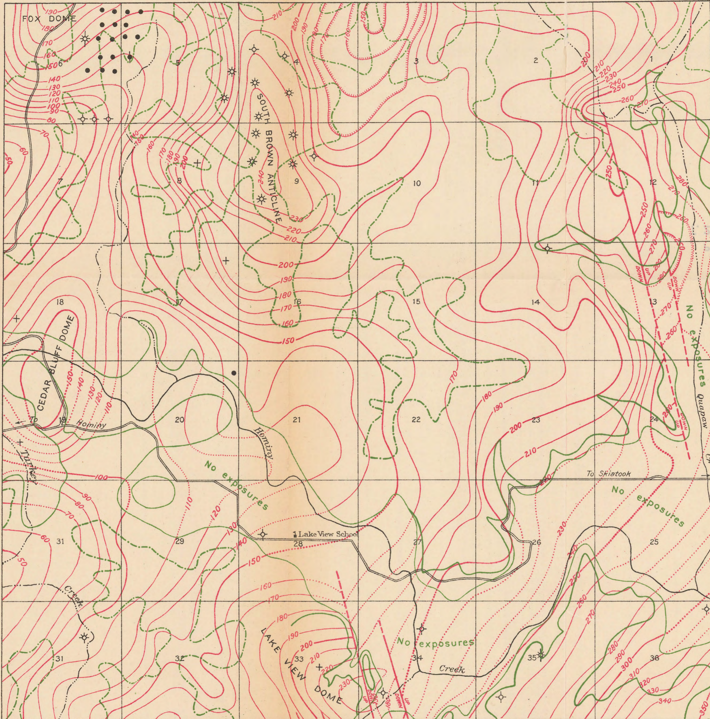
MAP SHOWING GEOLOGIC STRUCTURE OF T. 22 N., R. 11 E., OKLAHOMA
