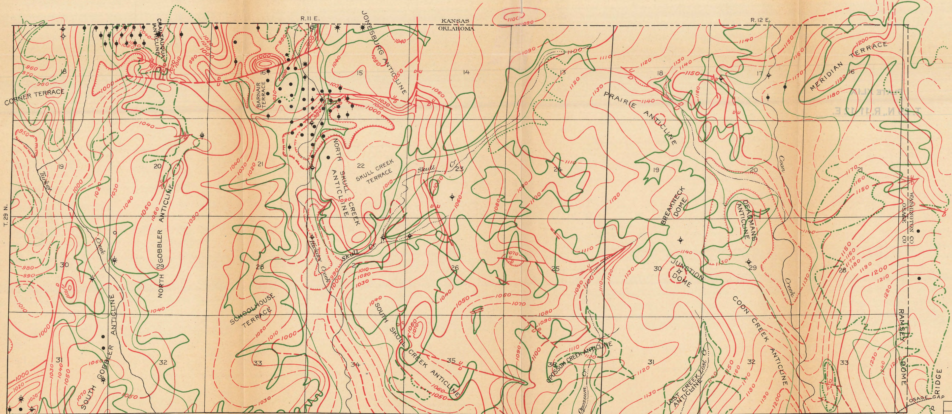
MAP SHOWING GEOLOGIC STRUCTURE OF T. 29 N., RS. 11 AND 12 E., OKLAHOMA
