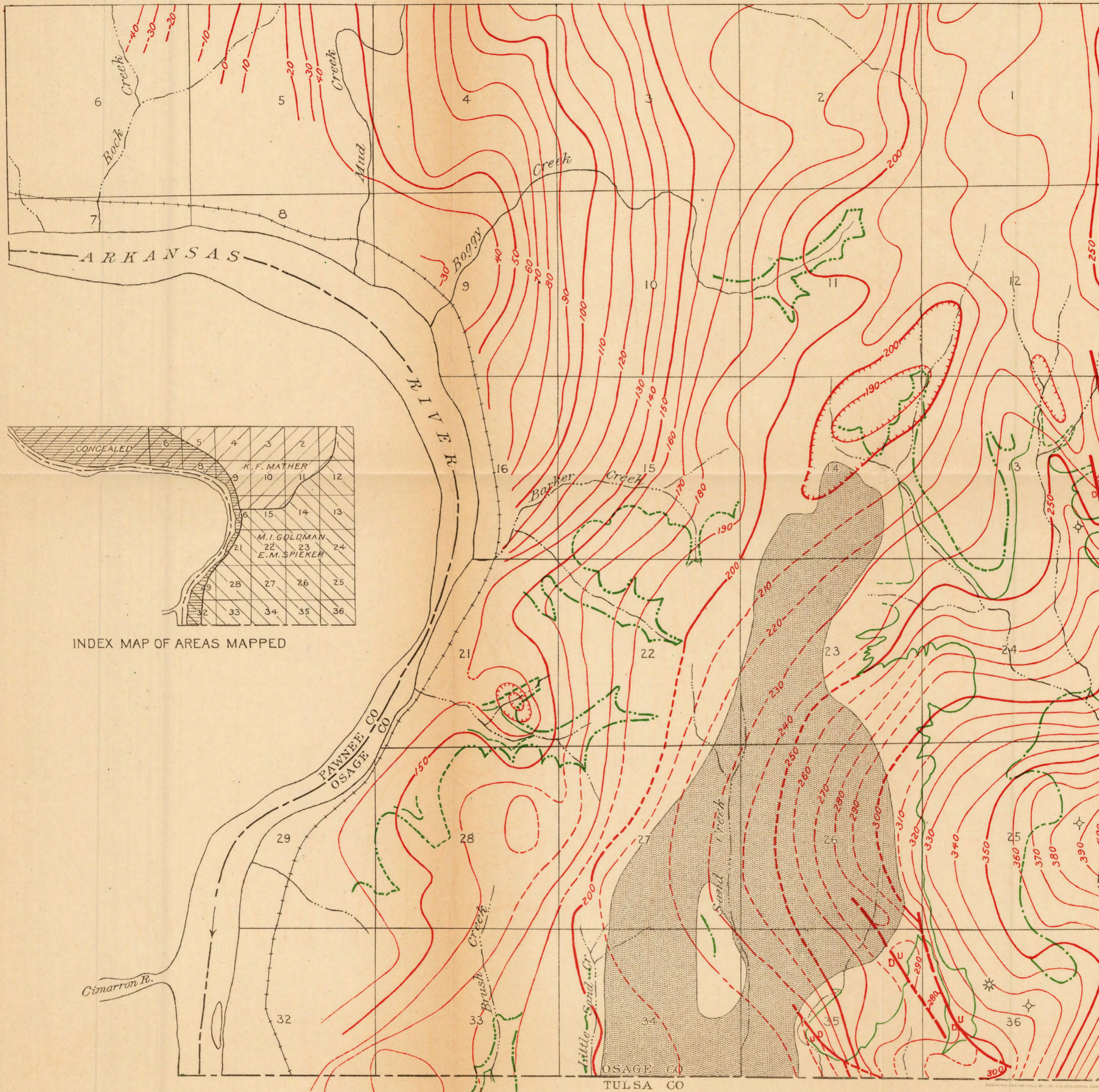
MAP SHOWING GEOLOGIC STRUCTURE IN T. 20 N., R. 10 E., OKLAHOMA, AND OUTCROPS OF CERTAIN BEDS OF ROCK
