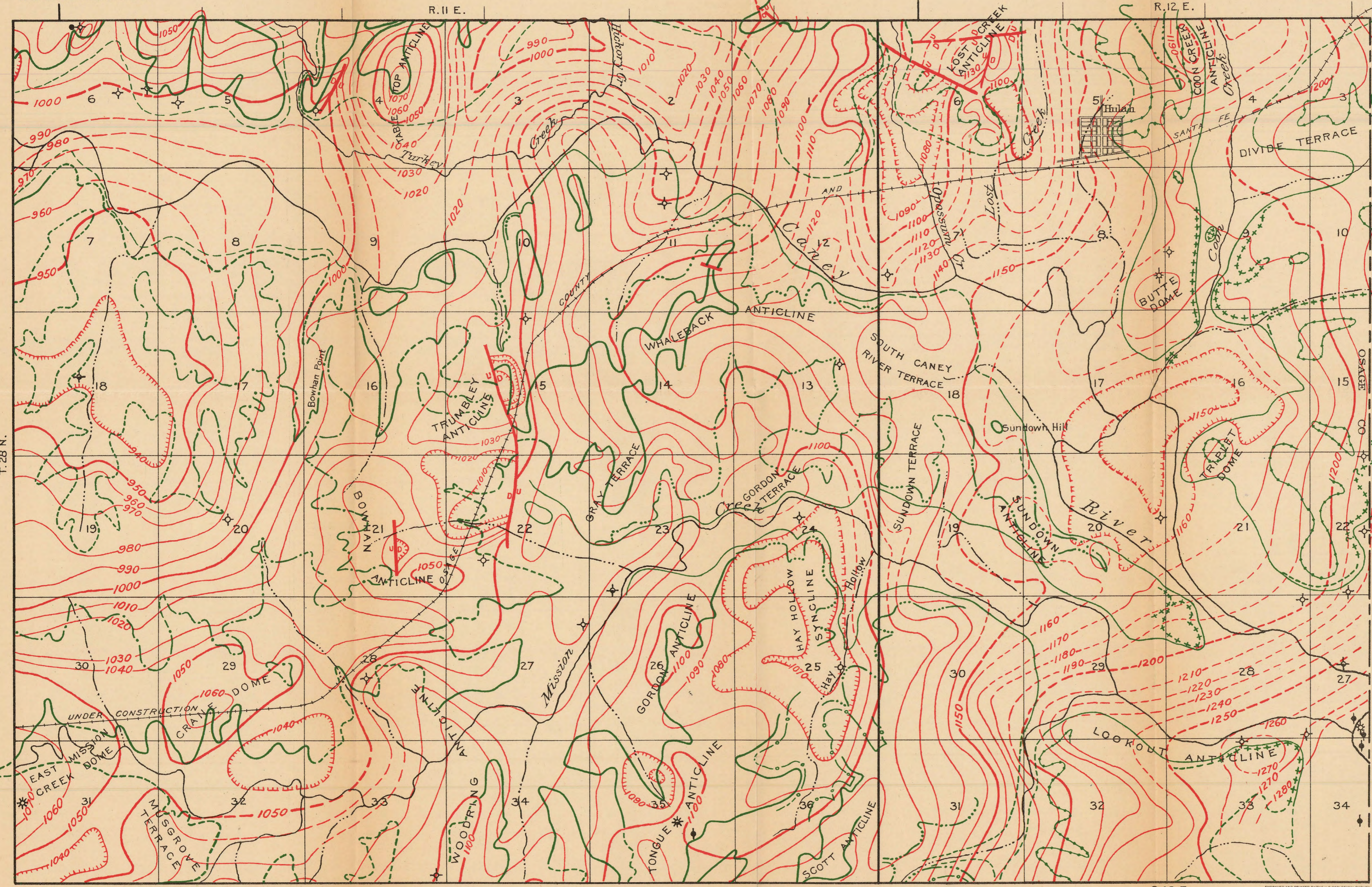
MAP SHOWING GEOLOGIC STRUCTURE, OUTCROPS OF CERTAIN BEDS, AND LOCATION OF WELLS IN T. 28 N., RS. 11 AND 12 E., OKLAHOMA
