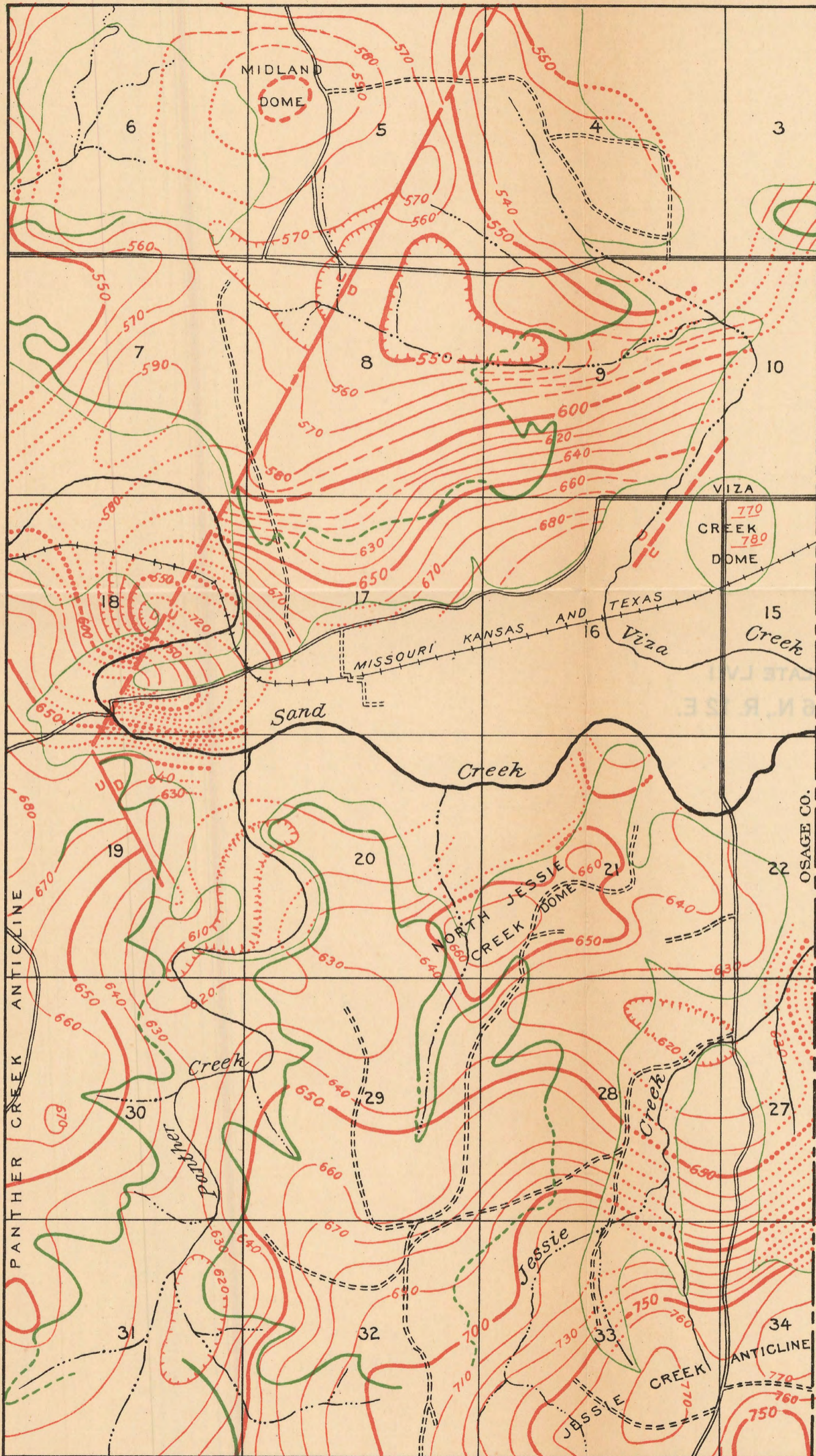
MAP SHOWING GEOLOGIC STRUCTURE OF T. 26 N., R. 12 E., OKLAHOMA AS DETERMINED FROM SURFACE ROCKS
