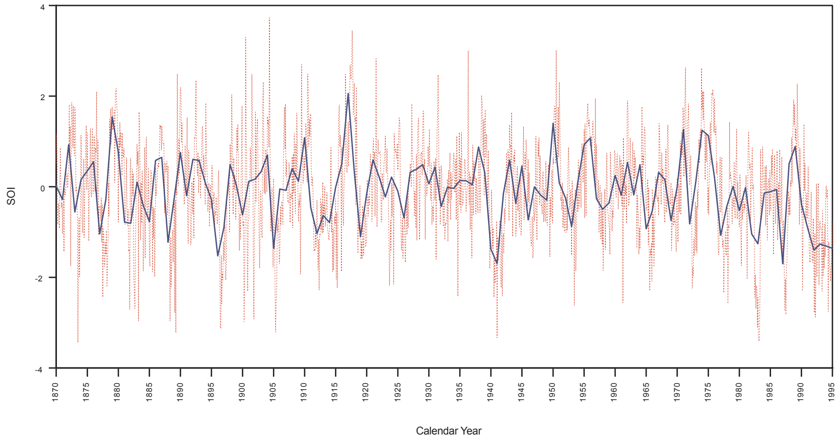
Figure 18. The mean annual Southern Oscillation Index (SOI) in blue and the monthly SOI in red, 1870-1995. See text section,
