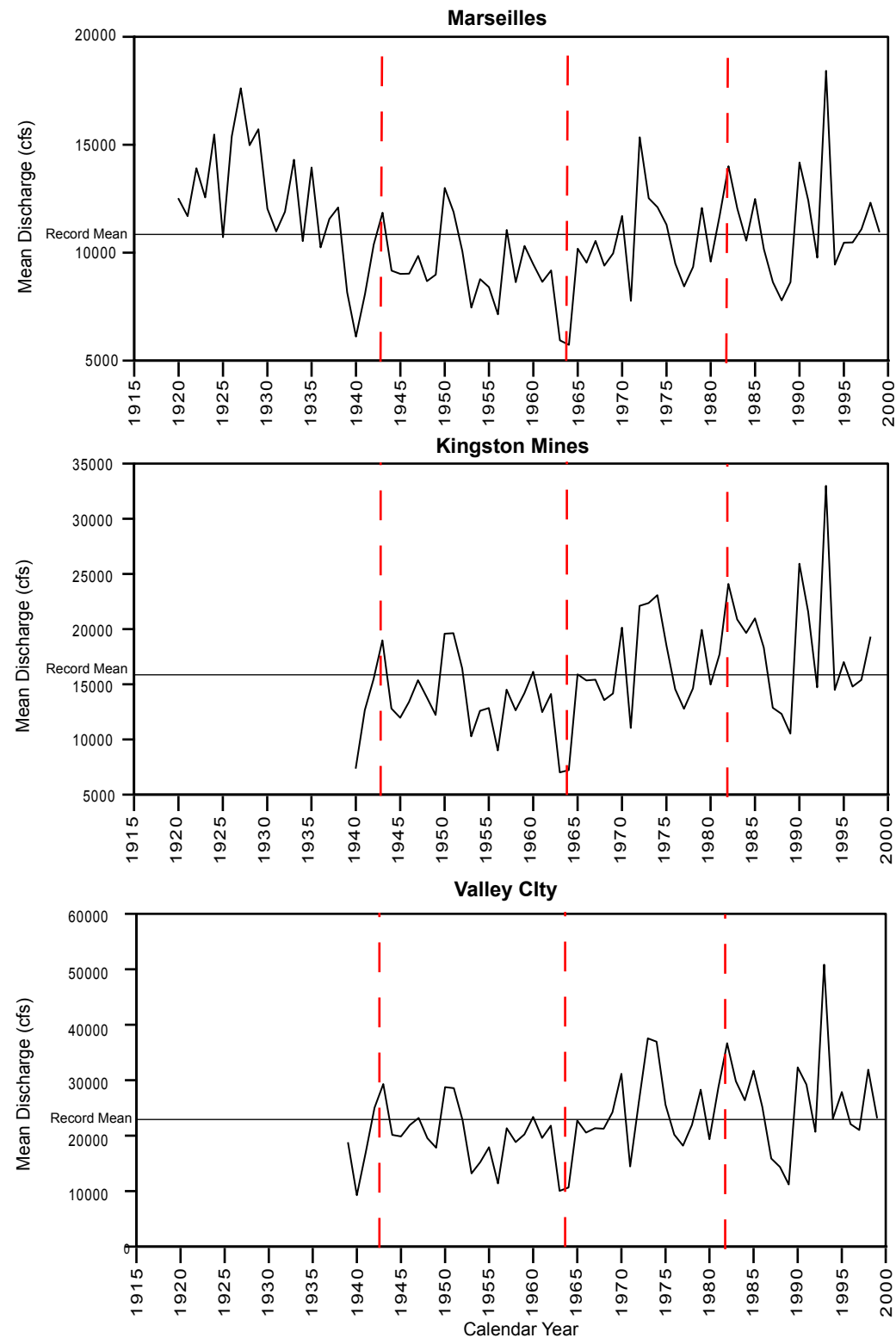
Figure 5. Illinois River gaging station locations and discharge records. Interstation comparisons indicate that mean annual discharge has not been significantly modified by manmade structures. The longest record from Marseilles was selected to represent the Illinois River flow. Dashed vertical lines track similarities between the records; the horizontal line in each record represents the mean discharge for the entire record. cfs, cubic feet per second.
