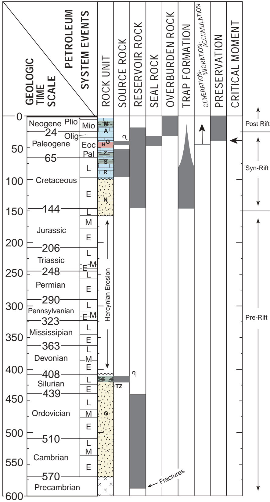
Figure 14. Sirte-Zelten Total Petroleum System events chart. Significant rock units noted on chart include GH, Gargaf/Hofra Formation—Cambrian-Ordovician sandstones; TZ, Tanezzuft Shale—Silurian; N, Nubian or Sarir Sandstone—Jurassic—Early Cretaceous; R, Rakk Group—Cretaceous, Turonian-Campanian; S, Sirte Shale Member of Rakk Group, primary source rock—Campanian; Z, Zelten Group carbonates—Paleocene; H, Hon Evaporite Member of Gir Formation—Eocene-Ypresian; G, Gialo Formation carbonates—middle Eocene-Lutetian; A, Arida Formation—Oligocene; M, Marada Formation—Miocene.
