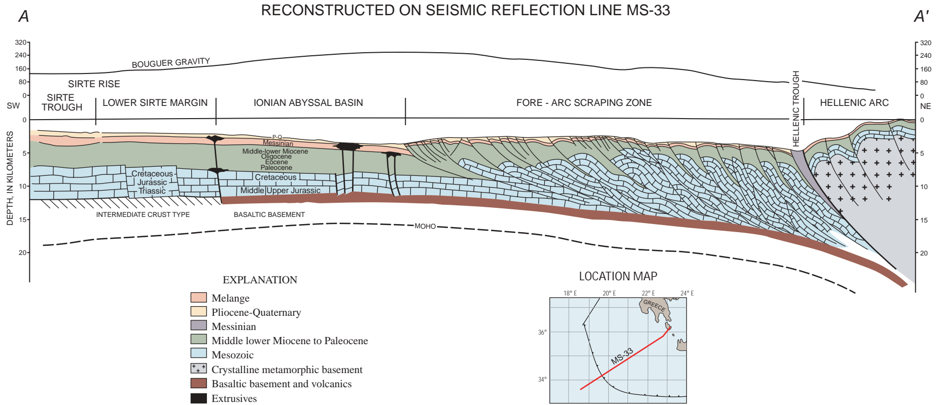
Figure 4. Northeast-southwest offshore regional cross section showing structural, tectonic, and crustal relationships in offshore Sirte Rise to Hellenic Arc (modified from Finetti, 1982).
