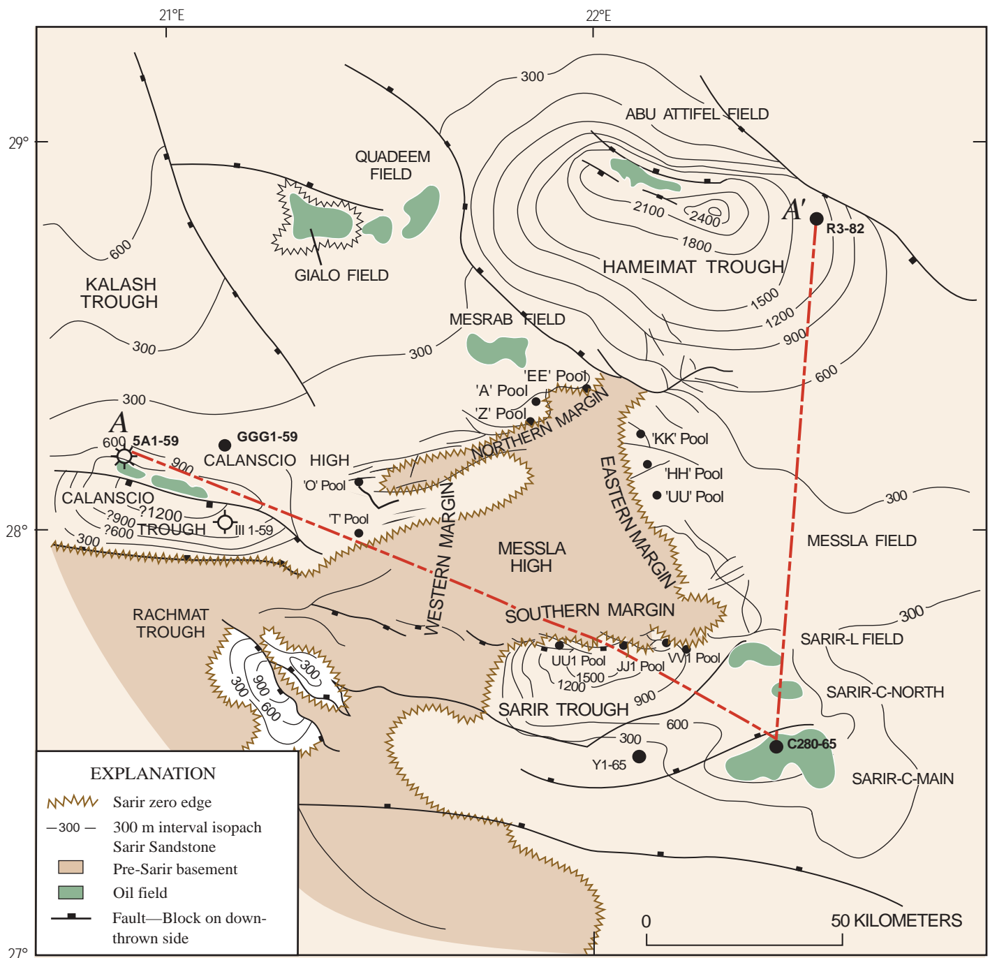
Figure 15. Tectonic elements and oil fields in eastern Sirte Basin. Sarir Sandstone isopachs are shown in main depocenters (modified from Ambrose, 2000). Cross section A–A' shown in figure 16.
