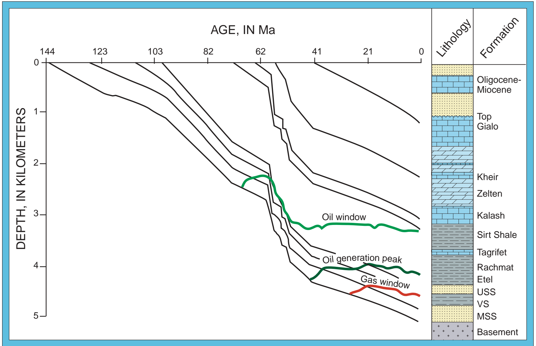
Figure 10. Burial history curve for deepest portion of Sirte Trough (the Hameimat Trough), southeastern Sirte Basin (modified from Bender and others, 1996). USS, upper Sarir Sandstone; VS, variegated shale; MSS, middle Sarir Sandstone.
