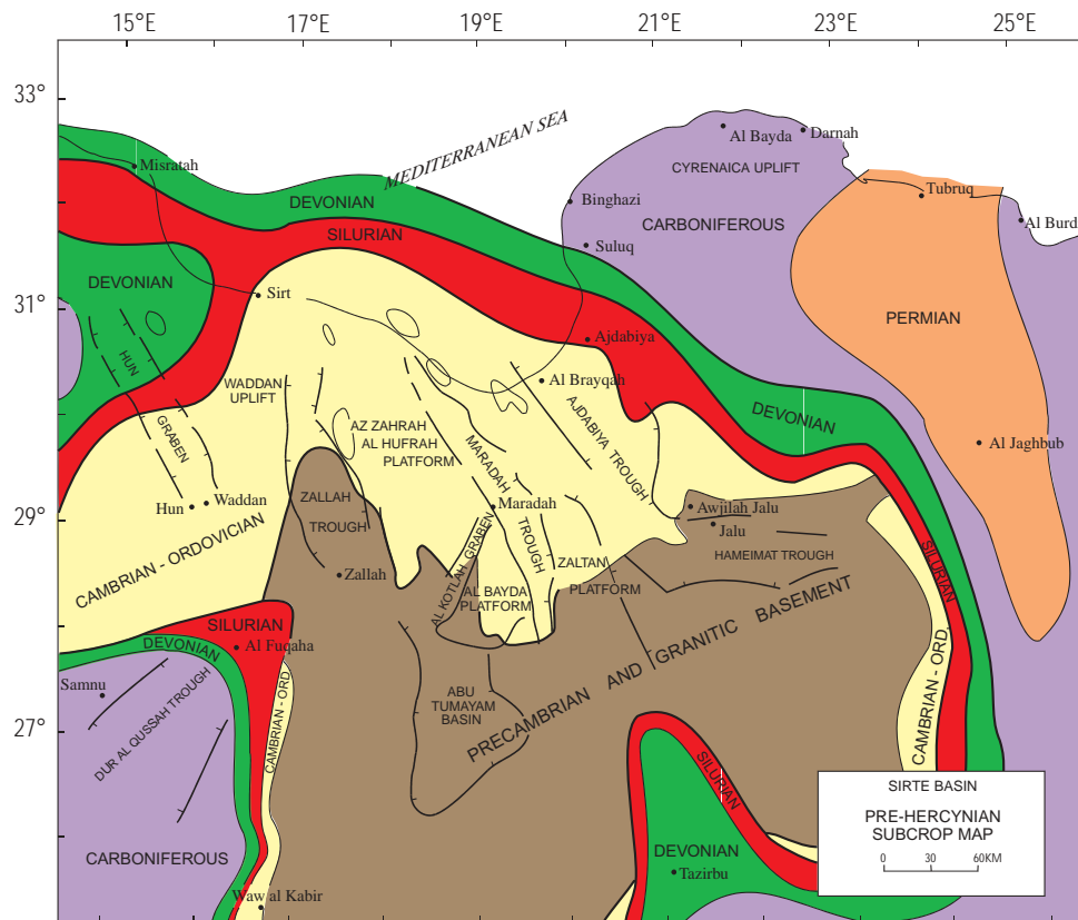
Figure 6. Pre-Hercynian subcrop map in Sirte Basin area (modified from Hallett and El Ghoul, 1996).
