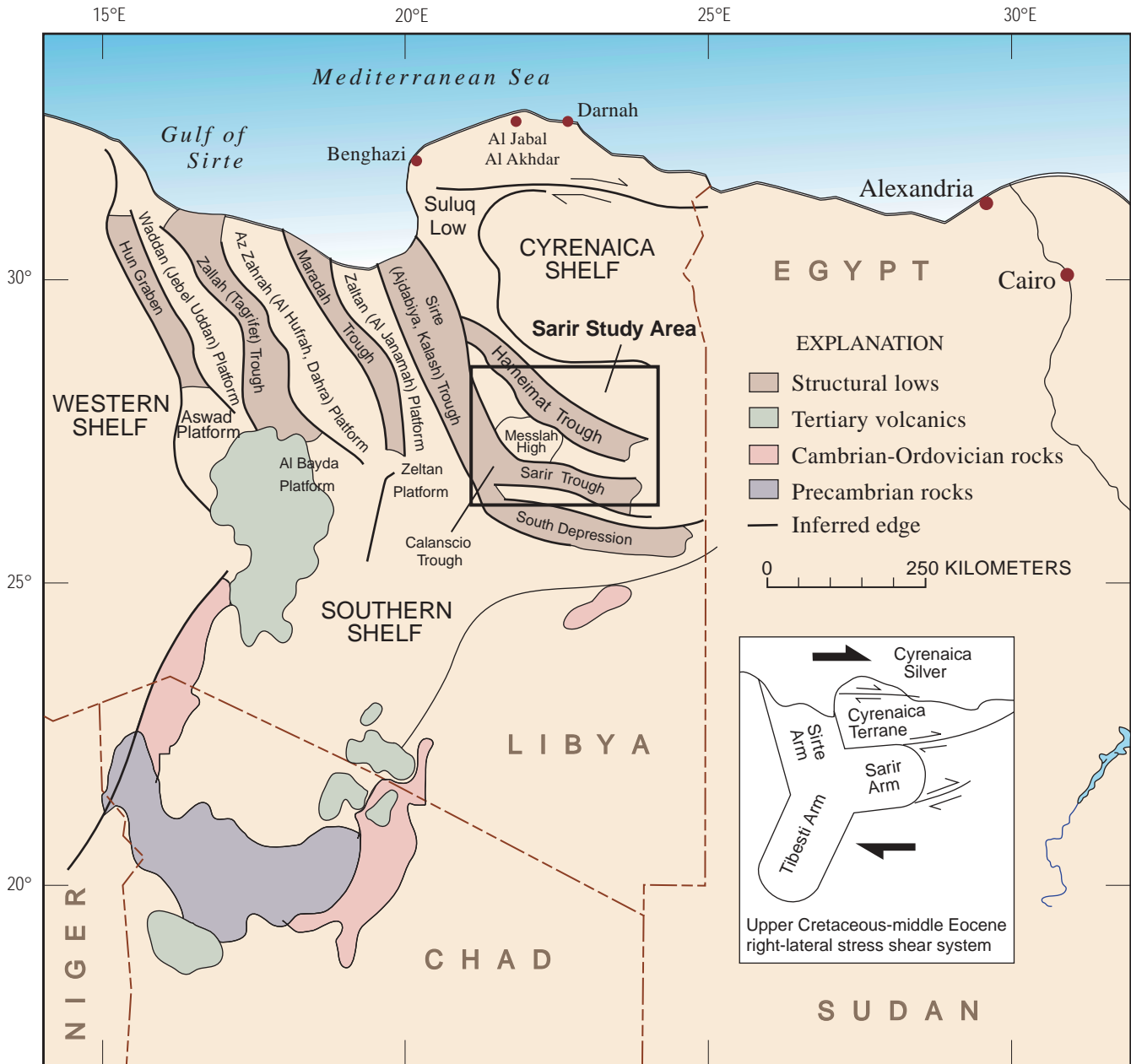
Figure 2. Structural elements of Sirte Basin. Troughs and grabens, platforms and horsts are synonymous terms. Individual horsts and grabens possess multiple names. For example, the Sirte (Sirt) Trough is also known as the Kalash or Ajdabiya Trough, as noted (modified from Ambrose, 2000). Barbs show direction of relative movement on faults.
