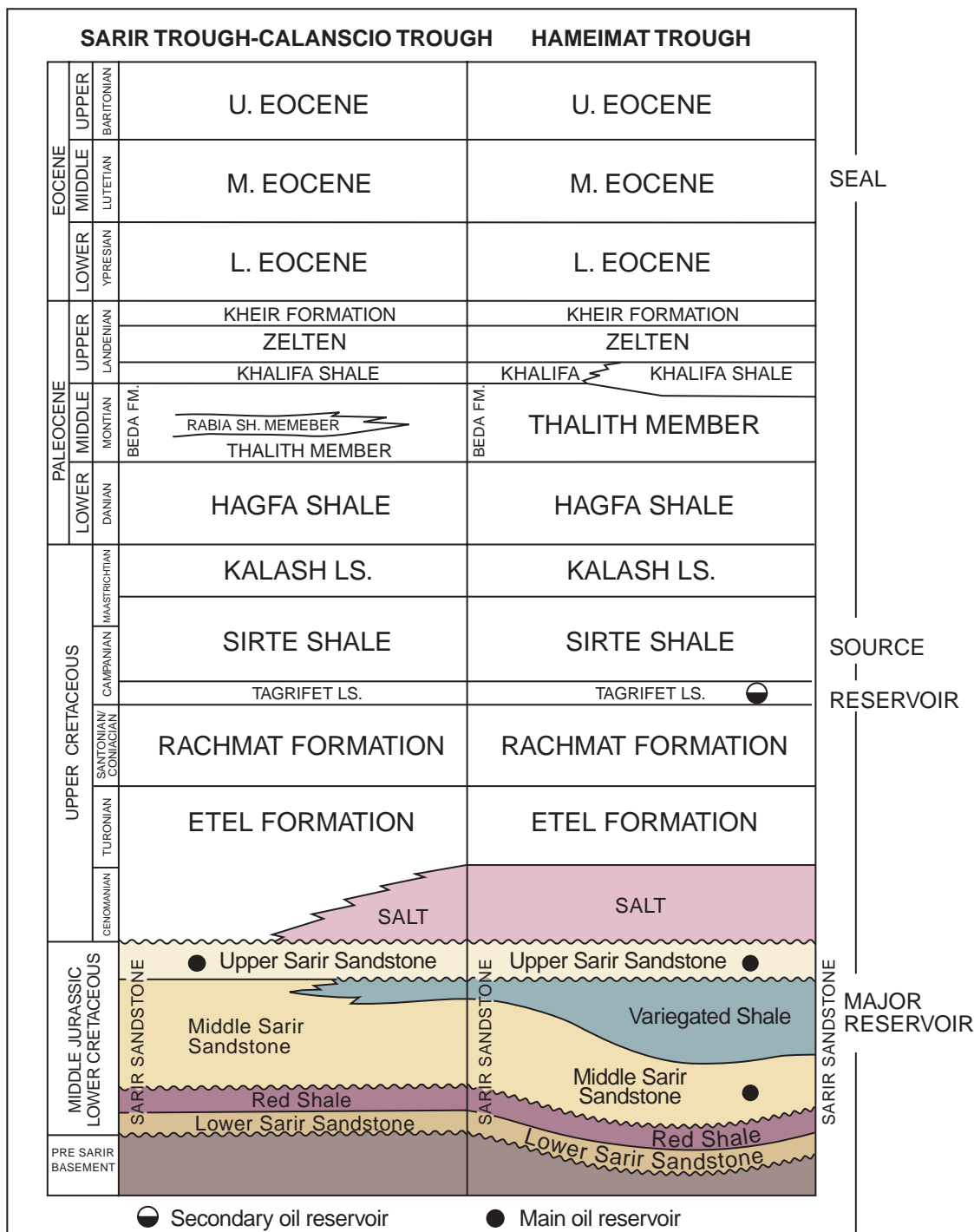
Figure 8. Stratigraphic section in eastern Sirte Basin (Sarir arm). The Sarir Sandstone is equivalent of the Nubian Sandstone of figure 7. Modified from Ambrose (2000).
