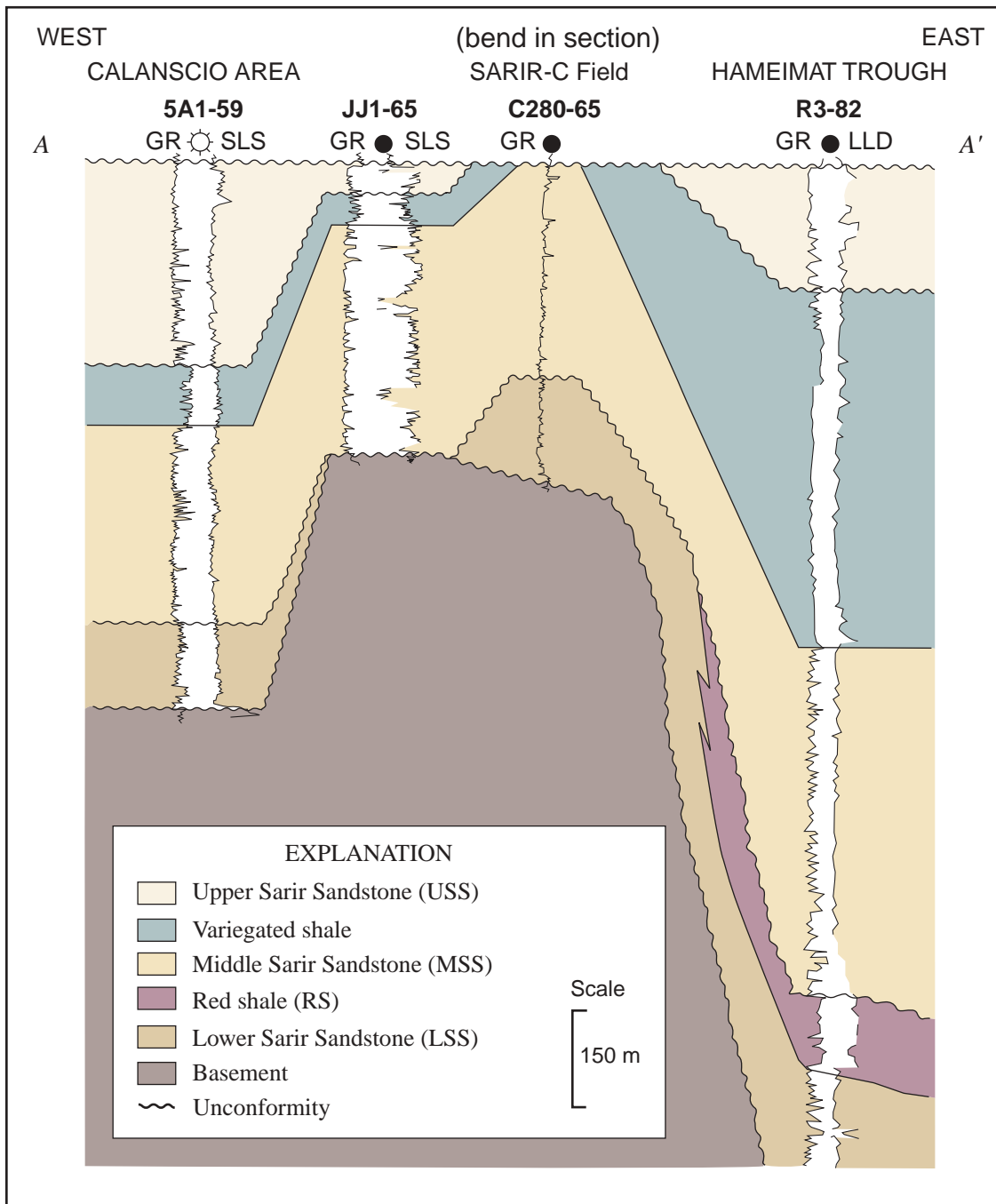
Figure 16. Stratigraphic cross section A–A' in Calanscio-Hameimat Trough (line of section shown in fig. 15). Note subdivisions (members) within the Sarir Sandstone and the combined structural-stratigraphic trap at Sarir-C field (modified from Ambrose, 2000).
