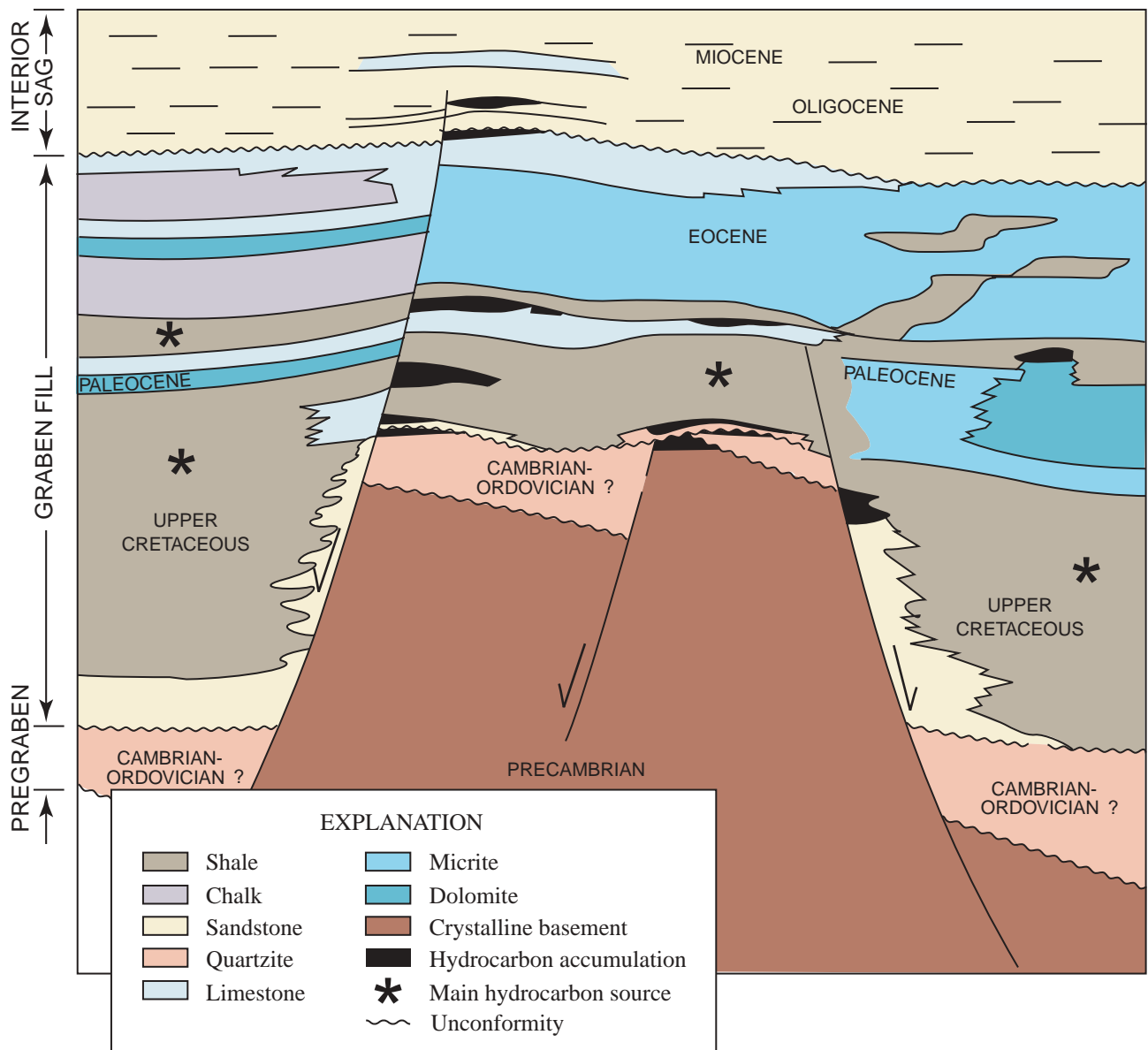
Figure 9. Schematic cross section showing general structural position, stratigraphic age, and lithology of most traps within the onshore Sirte Basin (modified from Harding, 1984). Note Upper Cretaceous source rocks charging multiple reservoirs on platforms (horsts). Bars show direction of relative movement on faults.
