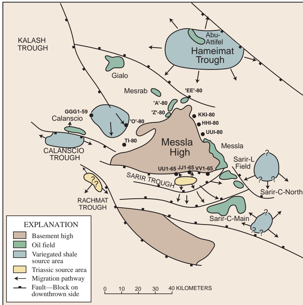
Figure 12. Postulated pre-Upper Cretaceous source areas and migration pathways of minor nonmarine source rocks in eastern Sirte Basin. Modified from Ambrose (2000).
