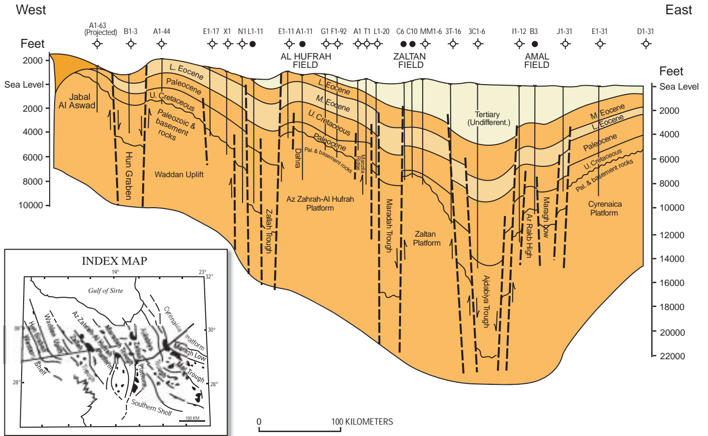
Figure 5. East-west onshore structural cross section across Sirte Basin (modified from Roohi, 1996a). Note name changes for troughs and platforms relative to figure 1 and nearly vertical displacement on faults (heavy dashed lines).
