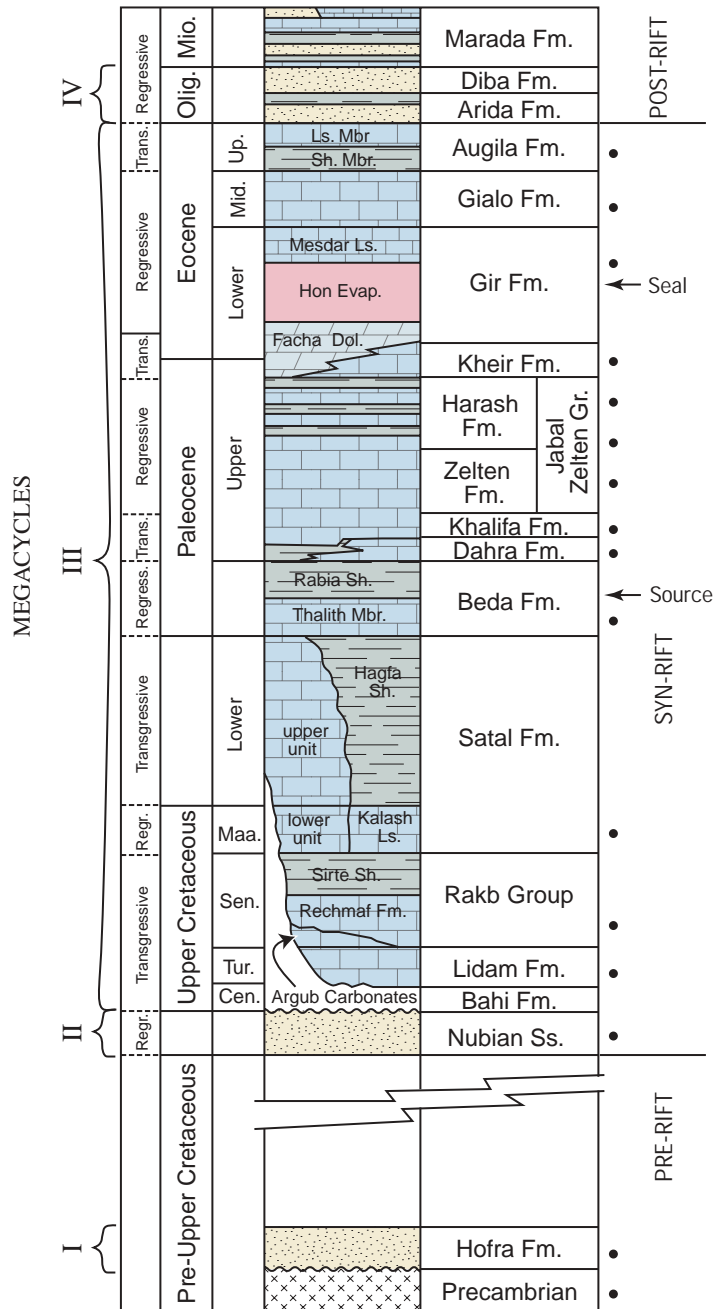
Figure 7. Stratigraphic section in central Sirte Basin (Sirte and Tibesti arms) (modified from Barr and Weeger, 1972; Montgomery, 1994). Primary hydrocarbon source and seal rock intervals are shown. Reservoirs are indicated by dots.
