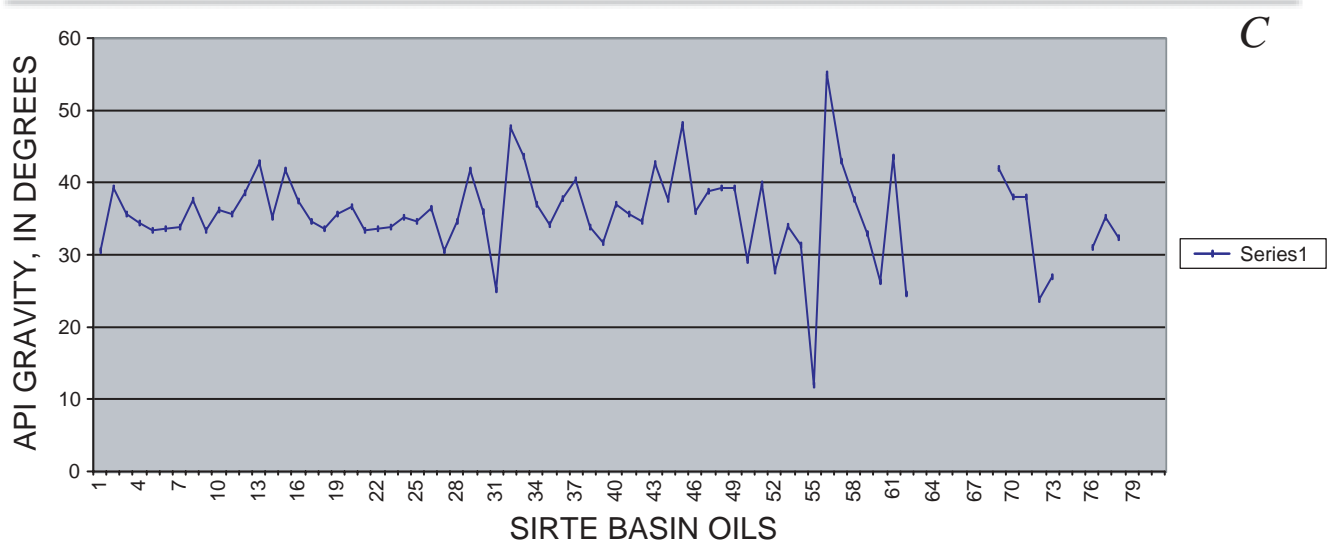
Figure 13. Oil geochemistry plots utilizing data from GeoMark (1998) for 81 oil samples from 55 fields in Sirte Basin. A, Pristane/phytane ratios; B, Sulfur percentages; C, API gravity.
