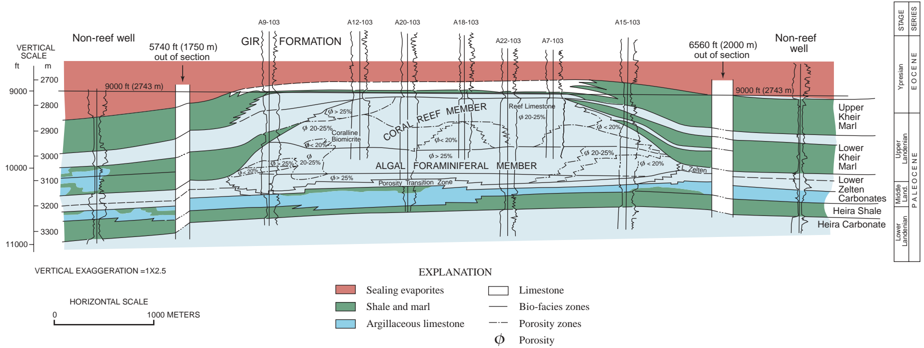
Figure 19. Stratigraphic cross section through Zelten Formation (Paleocene) bioherms, Idris "A" field, northeastern Sirte Basin, representing reservoirs in carbonate assessment unit (modified from Terry and Williams, 1969).
