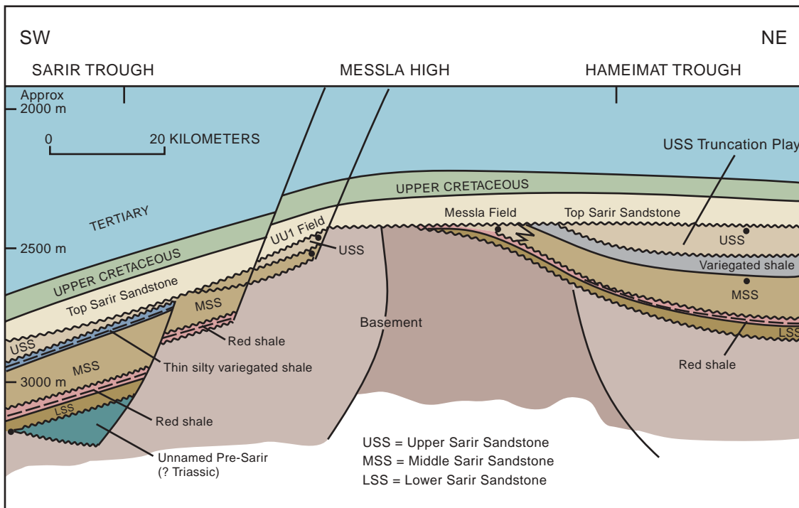
Figure 18. Schematic structural cross section from Sarir Trough across Messla High and into Hameimat Trough showing hydrocarbon habitat of the Sarir Sandstone (modified from Ambrose, 2000). Note truncation and stratigraphic trap potential in various members of the Sarir Sandstone. Scale is approximate.
