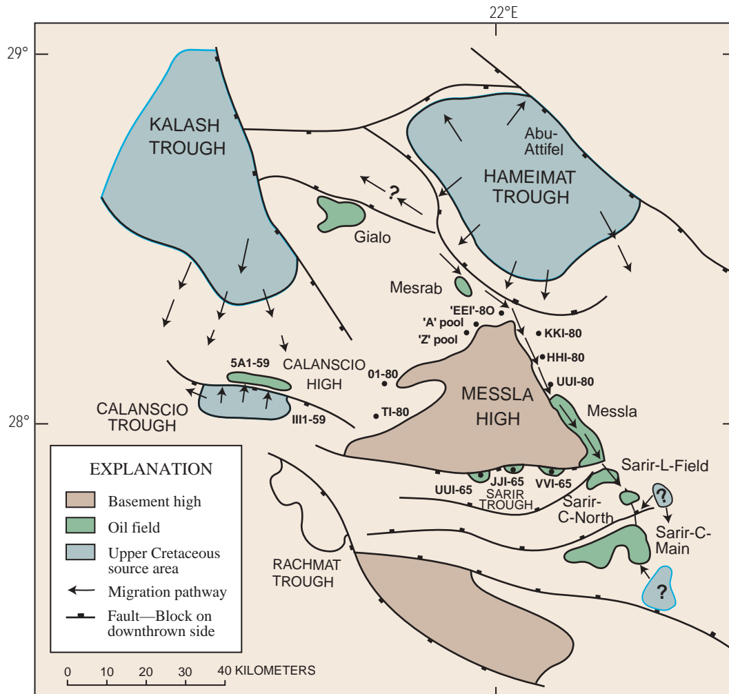
Figure 11. Postulated petroleum migration pathways for oil sourced from Upper Cretaceous shales, which also provide a regional seal in Sarir arm area of eastern Sirte Basin. Modified from Ambrose (2000).
