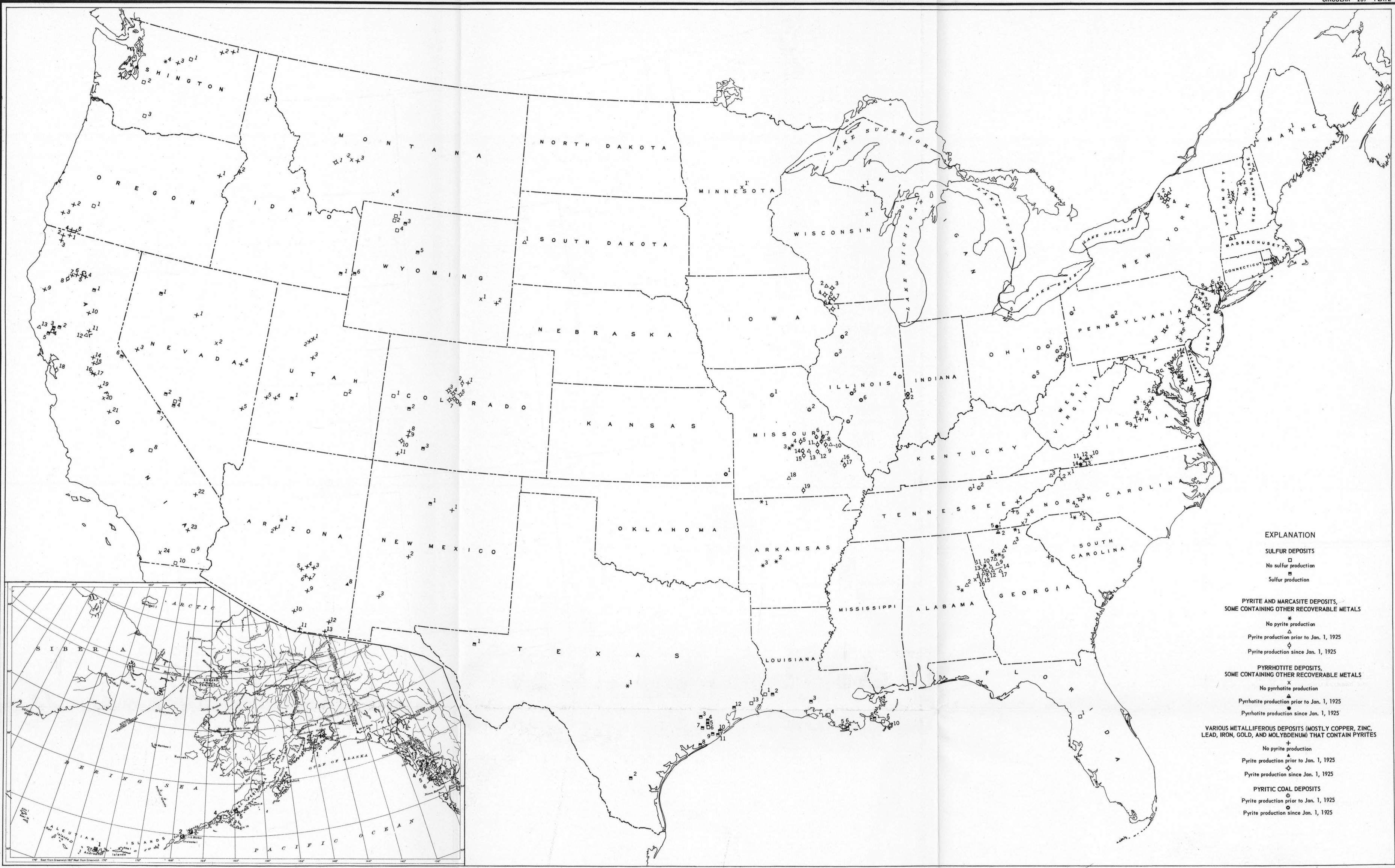
INDEX MAP OF SULFUR AND PYRITE DEPOSITS IN THE UNITED STATES AND ALASKA
