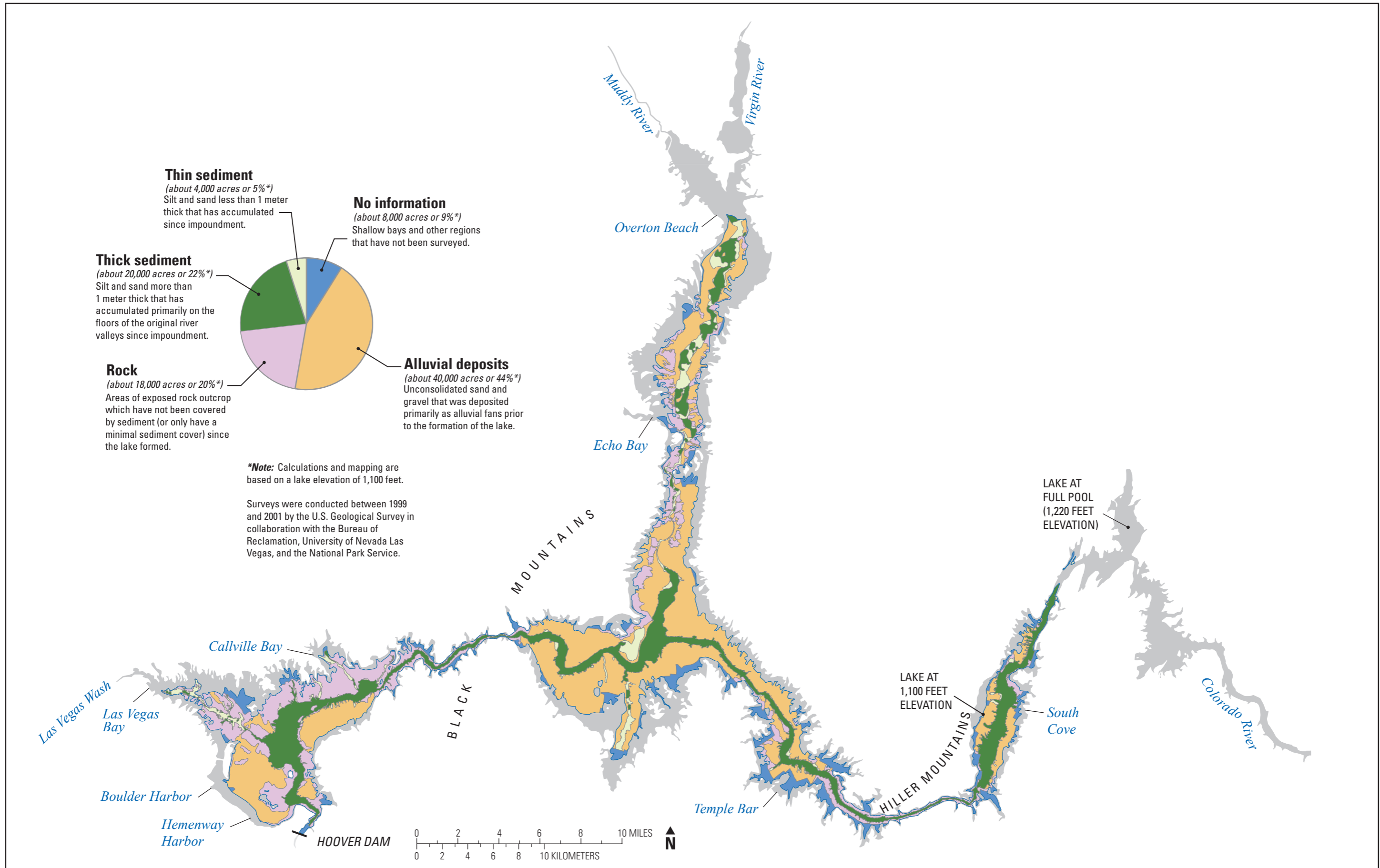
FIGURE 2.3—Interpreted lake-floor geology. Four units were mapped: outcrops of Tertiary and older rocks, Quaternary alluvial deposits, thick post-impoundment sediment deposits, and thin post-impoundment sediment deposits. These are represented in the map as rock, alluvial deposits, thick sediment, and thin sediment, respectively.
