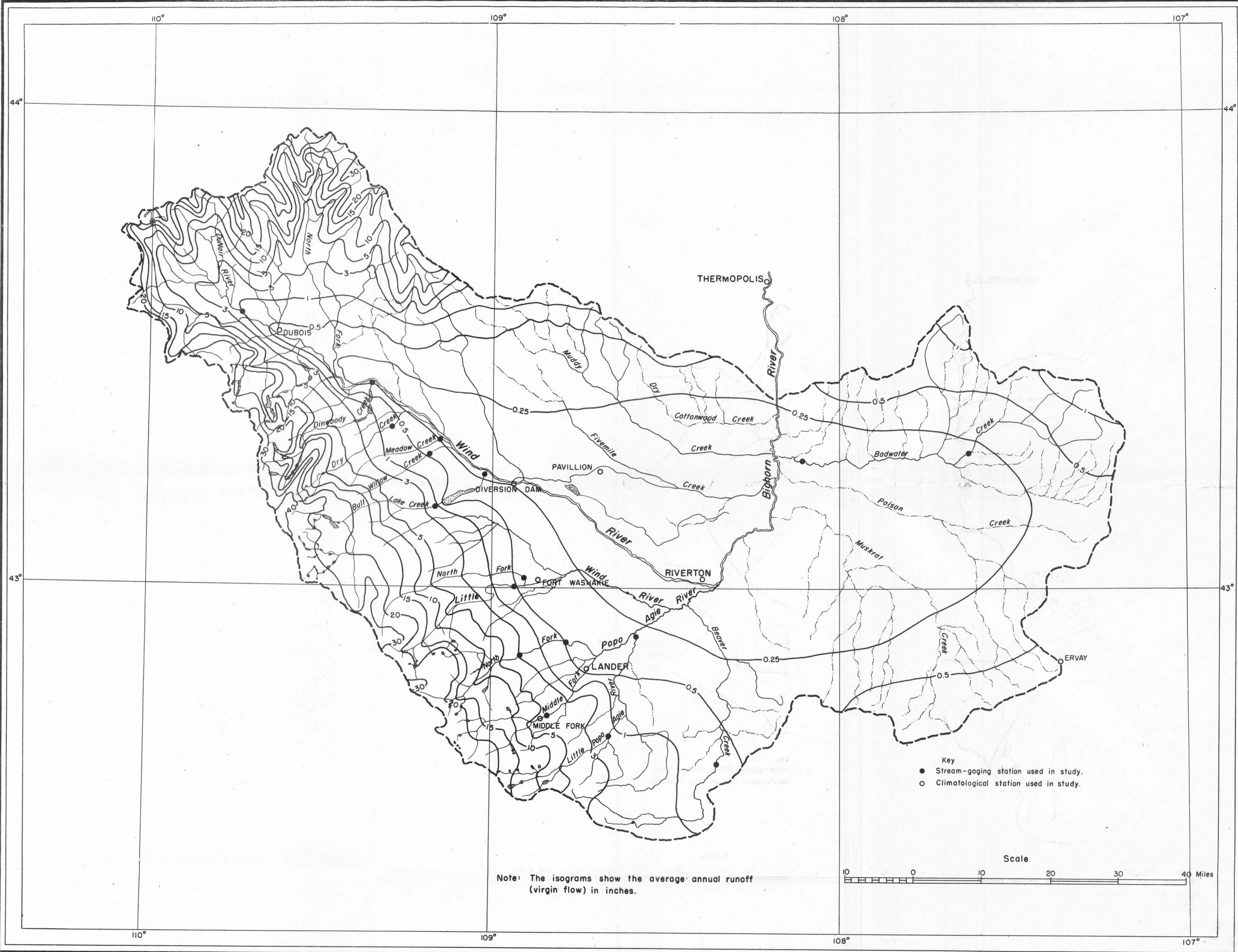
AVERAGE ANNUAL RUNOFF IN THE WIND RIVER BASIN
