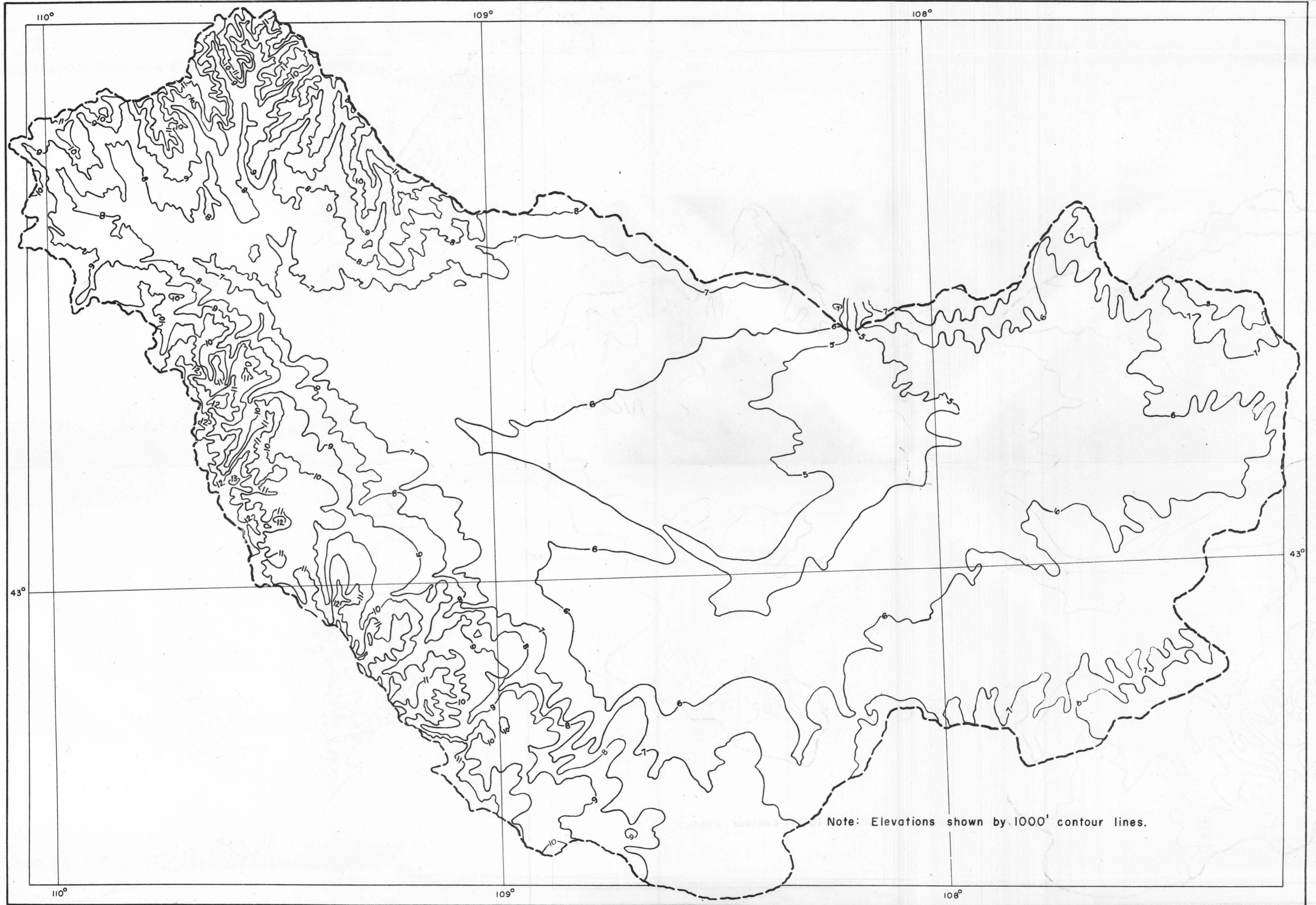
ALTITUDE VARIATION IN THE WIND RIVER BASIN
