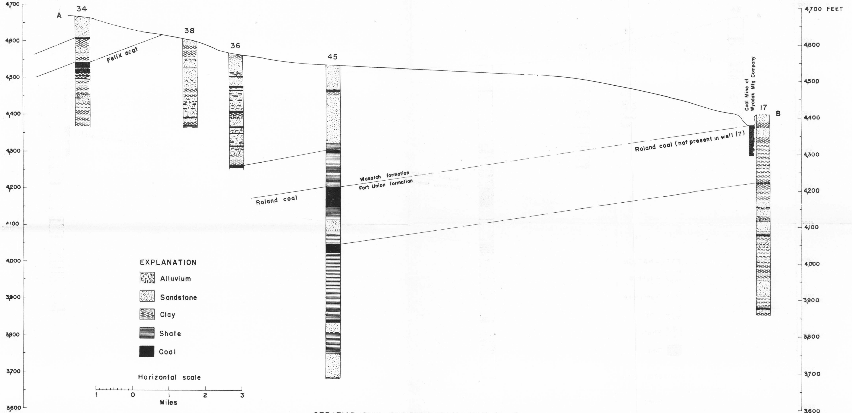
STRATIGRAPHIC SECTIONS ALONG LINE A — B
