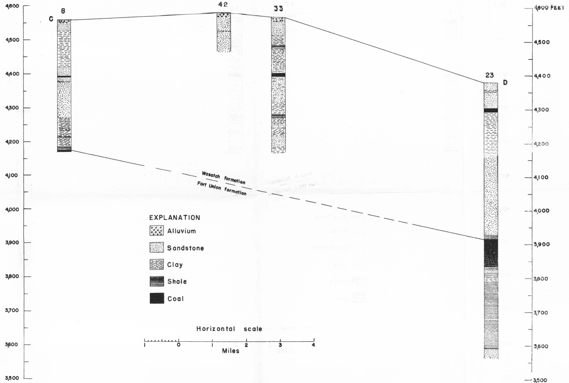
STRATIGRAPHIC SECTIONS ALONG LINE C-D
