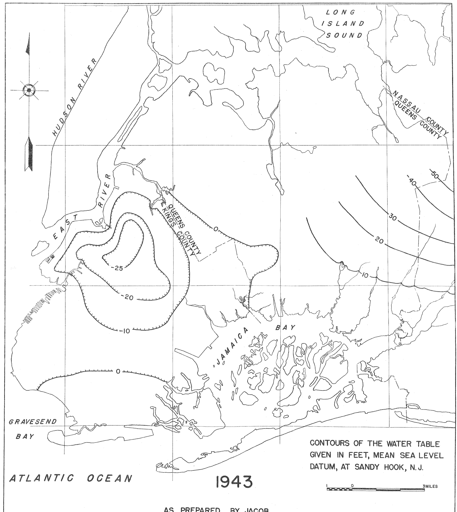
THE POSITION OF THE WATER TABLE IN KINGS AND QUEENS COUNTIES, N.Y. IN 1903, 1933, 1936, 1943
