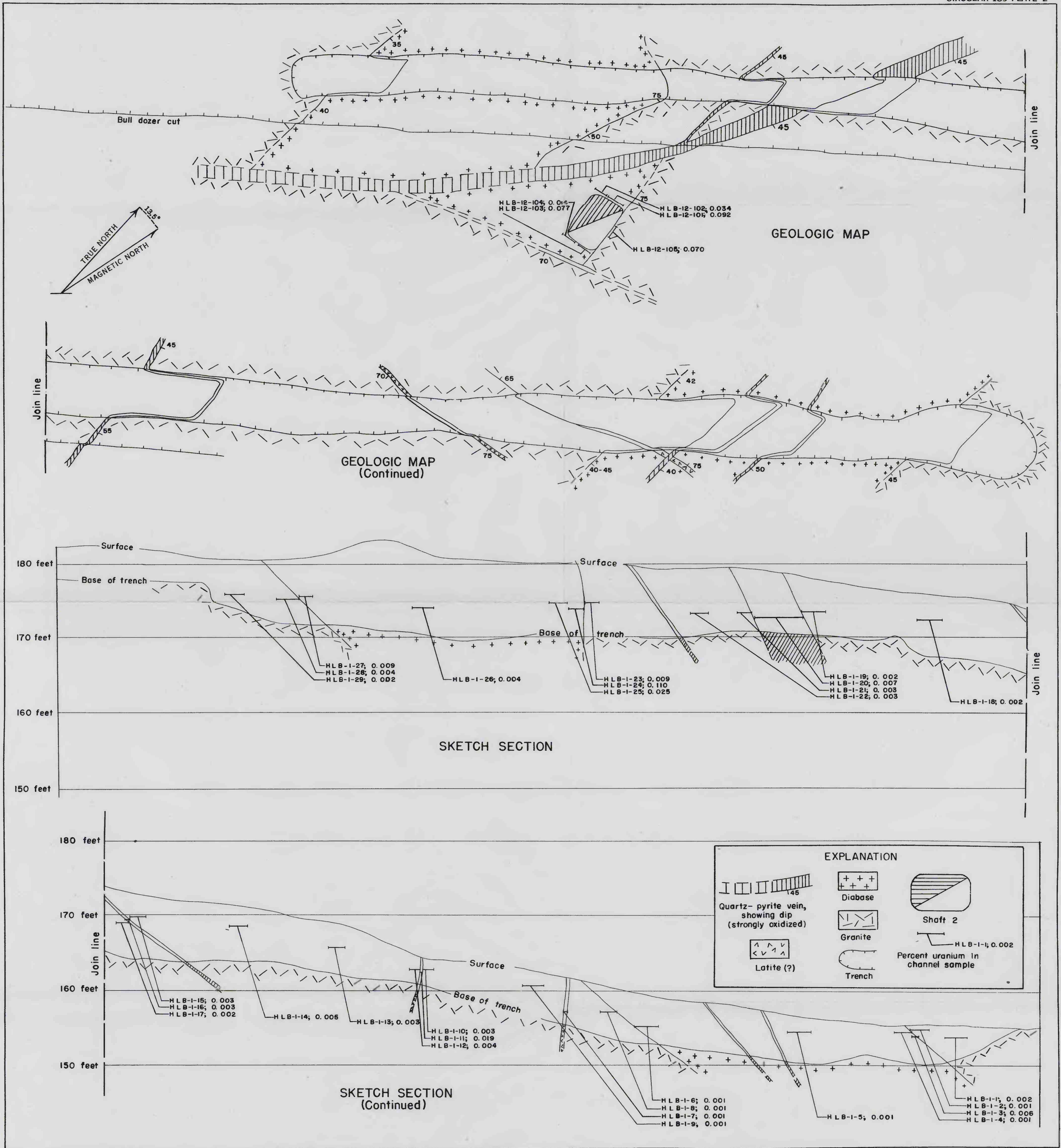
DETAILED GEOLOGIC MAP AND SKETCH SECTION, TRENCH I, MERRY WIDOW CLAIM, WHITE SIGNAL DISTRICT, GRANT COUNTY, NEW MEXICO
