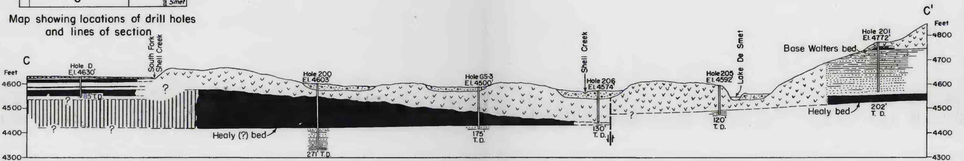
Section C-C'
