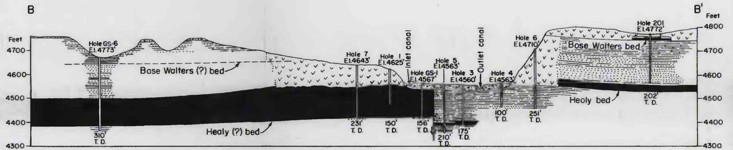
Section B-B'
