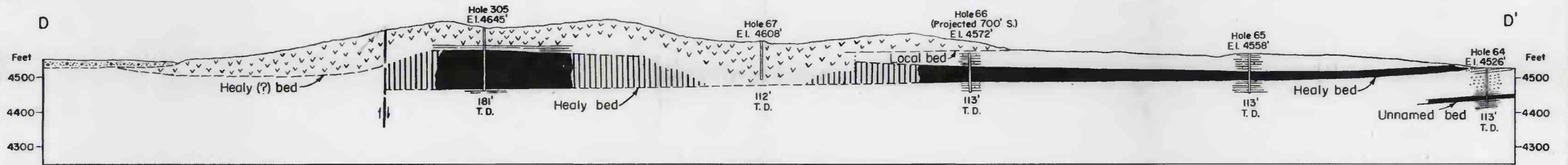
Section D-D'
