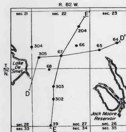
Map showing locations of drill holes and lines of section
