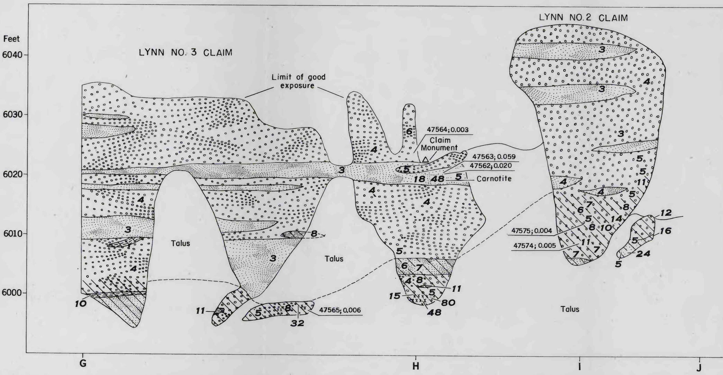
DIAGRAMMATIC SKETCHES OF THE URANIFEROUS DEPOSITS IN CLIFF FACE PROJECTED BETWEEN B, C, D, E, F, G, H, I, AND J
