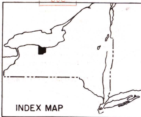
MAP OF ROCHESTER AREA, NEW YORK, SHOWING GAGING STATIONS AND BEDROCK CONTOURS
