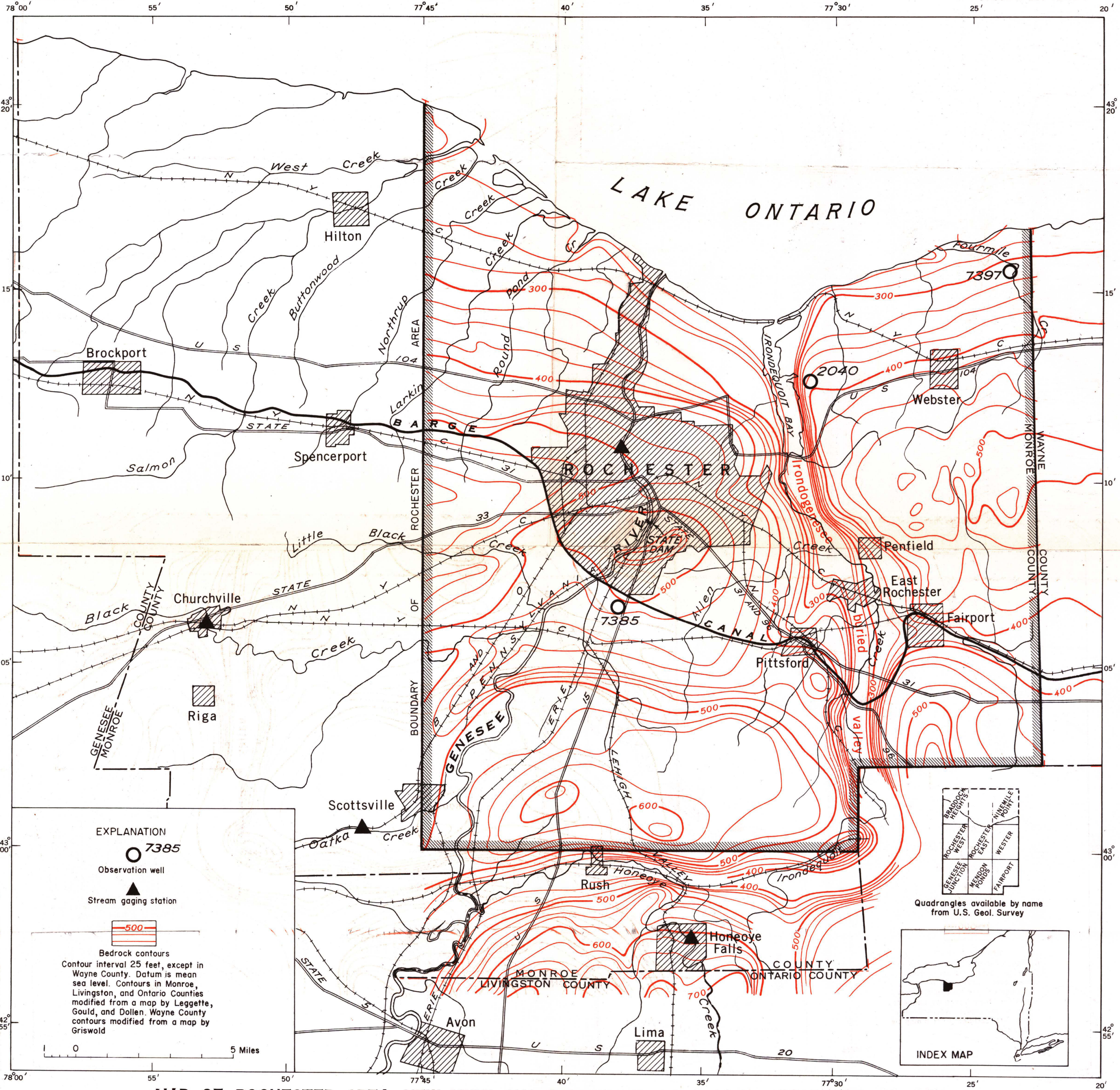
MAP OF ROCHESTER AREA, NEW YORK, SHOWING GAGING STATIONS AND BEDROCK CONTOURS
