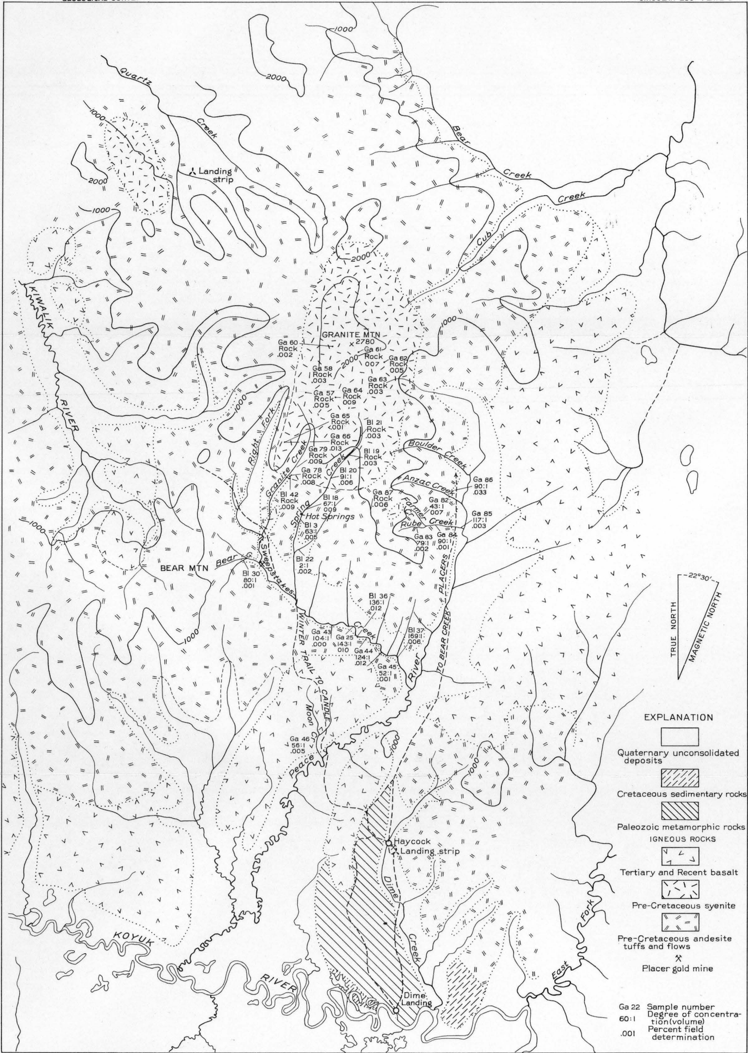
GEOLOGIC SKETCH MAP OF SWEEPSTAKES CREEK AND VICINITY, SEWARD PENINSULA, ALASKA
