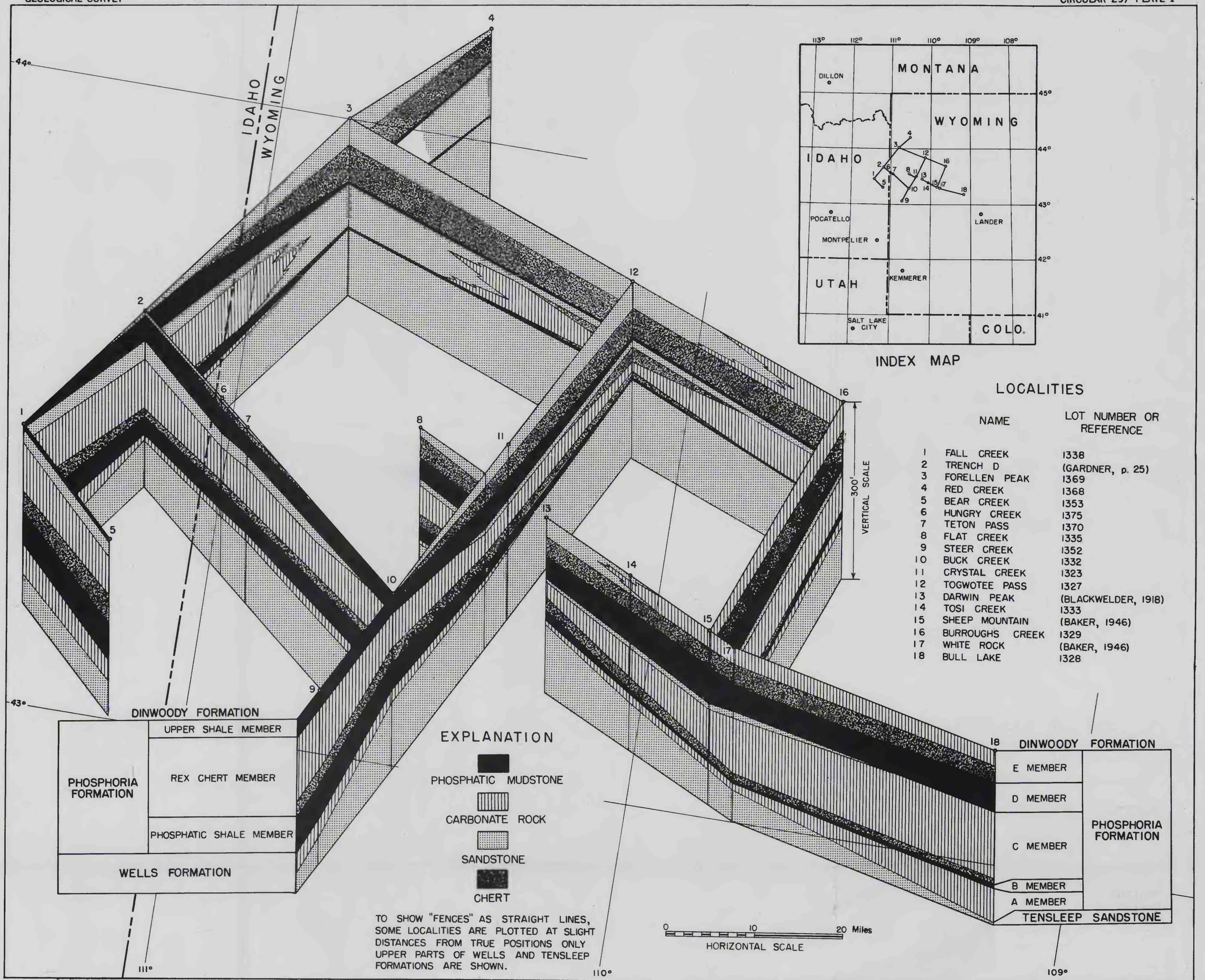
FENCE DIAGRAM SHOWING A LITHOLOGIC CORRELATION OF THE STRATA OF THE PHOSPHORIA FORMATION IN NORTHWESTERN WYOMING
