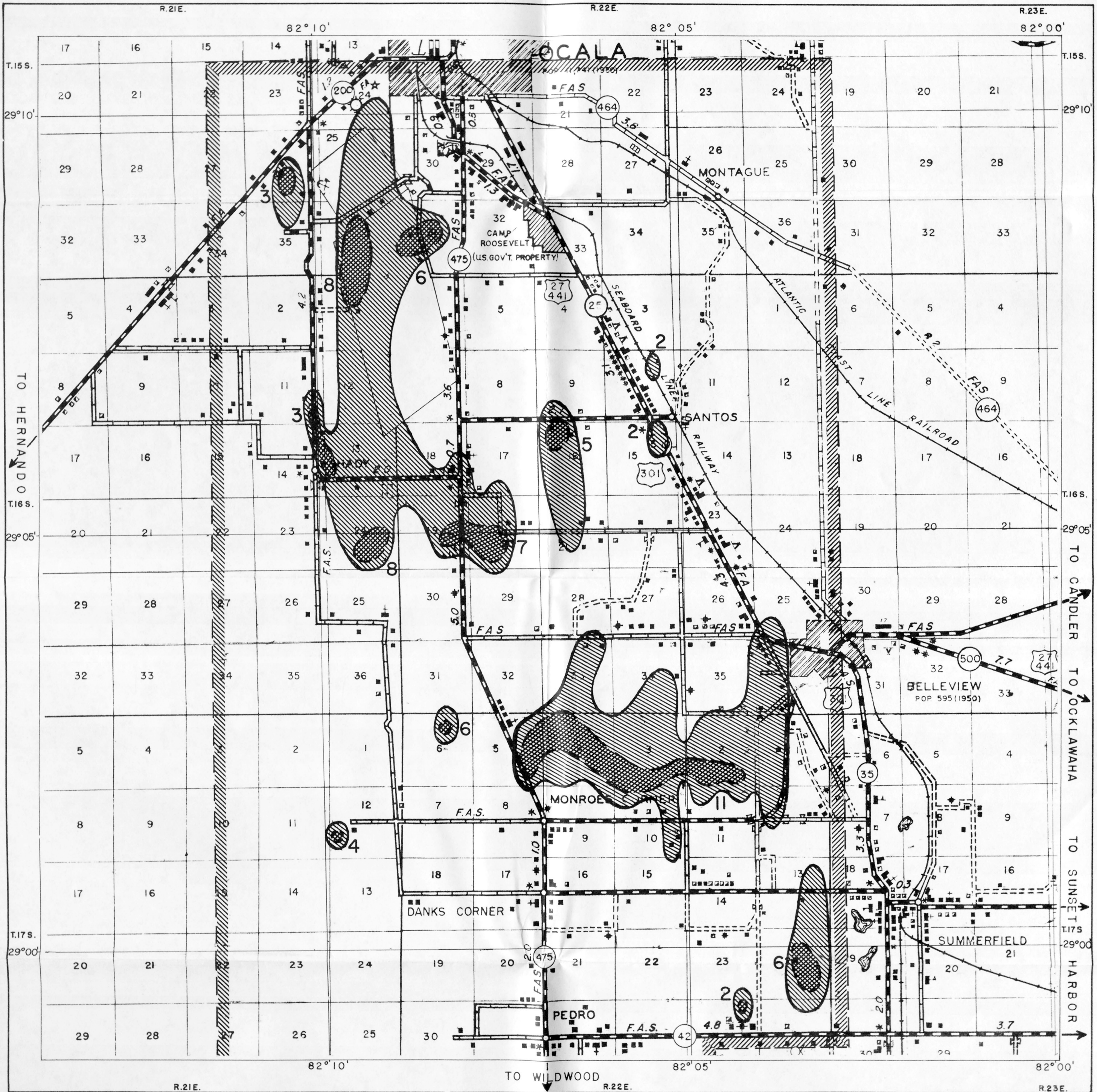
FIGURE 2 AIRBORNE RADIOACTIVITY SURVEY OF PART OF MARION COUNTY, FLORIDA
