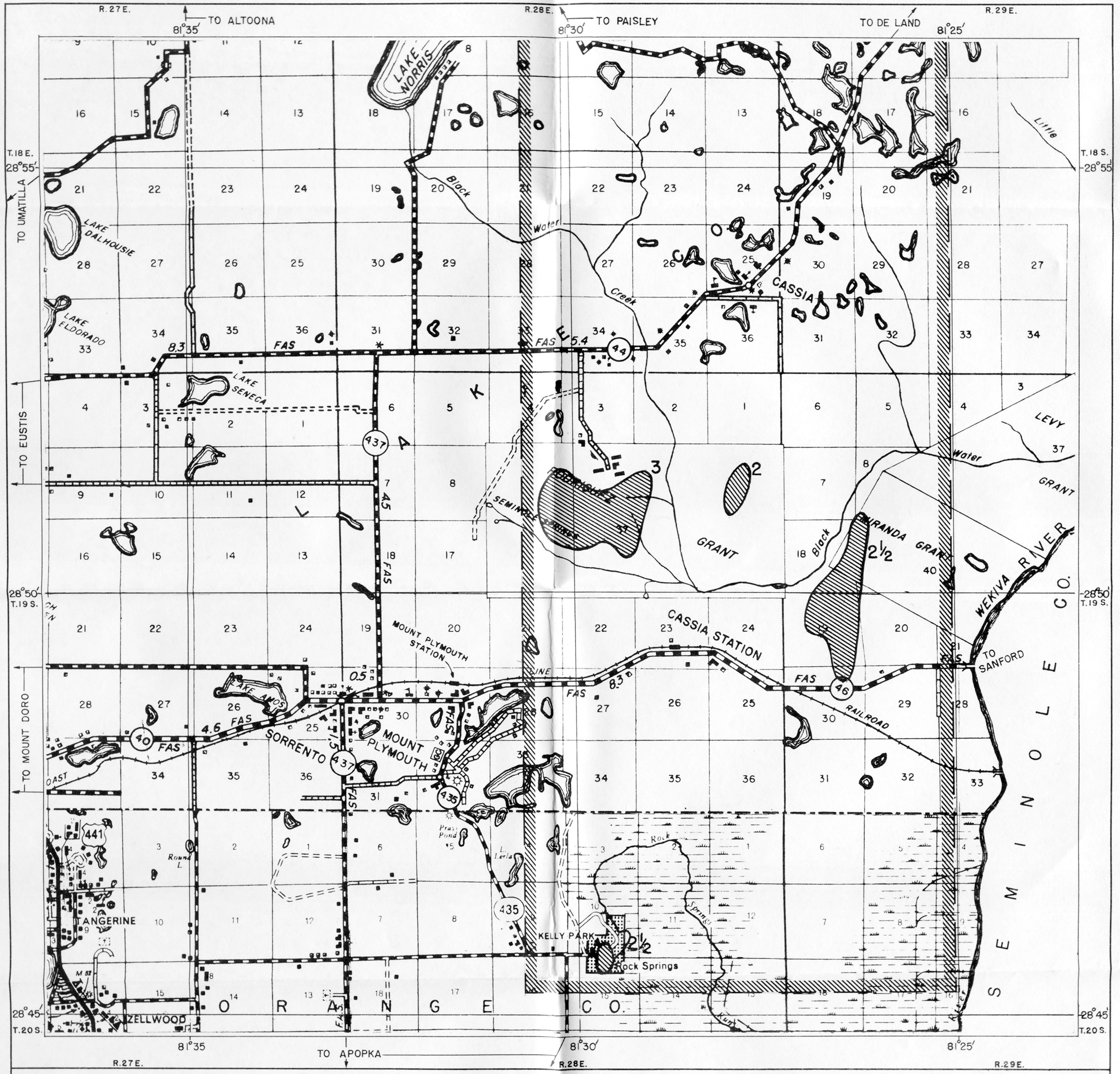
FIGURE 6 AIRBORNE RADIOACTIVITY SURVEY OF PARTS OF LAKE AND ORANGE COUNTIES, FLORIDA
