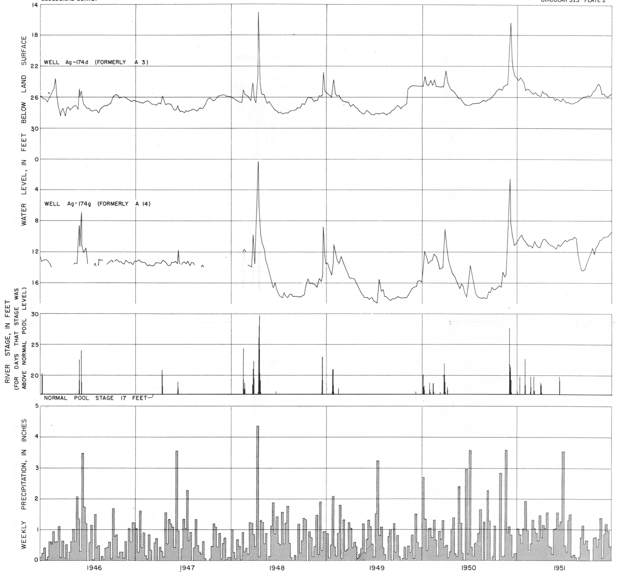
RELATIONS AMONG PRECIPITATION, RIVER STAGE, AND GROUND WATER LEVELS IN THE TRIANGLE AREA, 1946-51
