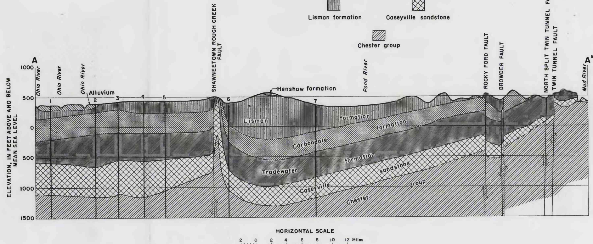
GENERALIZED GEOLOGIC CROSS SECTION OF THE WESTERN COAL FIELD, KENTUCKY
