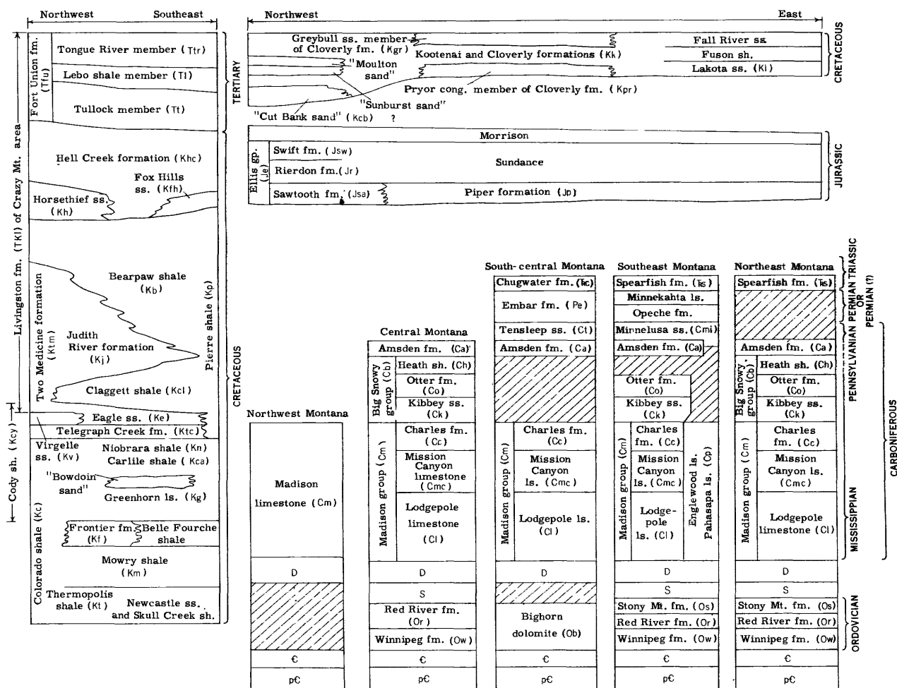
Figure 1.—Stratigraphic diagram and correlation chart for Montana with explanation of symbols used in table 2. (Nomenclature of upper Mississippian strata in central Montana has been revised and will differ from this in forthcoming publications. The Piper formation of Jurassic age rests on rocks of Mississippian to Triassic age in northeast Montana.)
