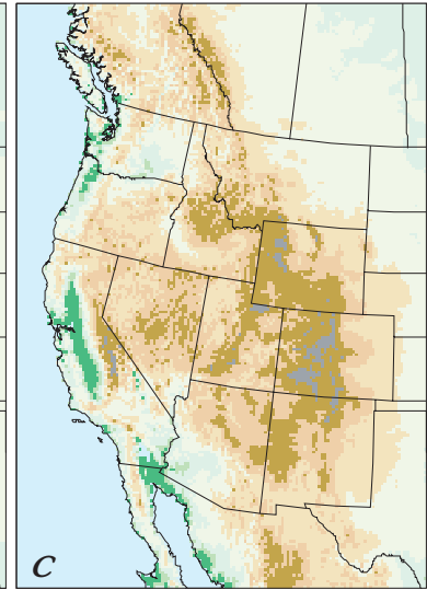
15-km LAND GRID POINT ELEVATIONS (m)
