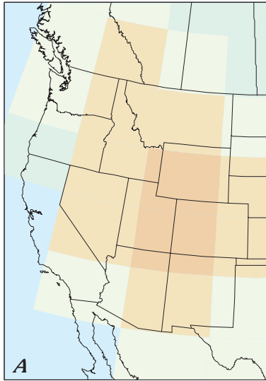
GENESIS LAND GRIDBOXES AND ELEVATIONS (m)
