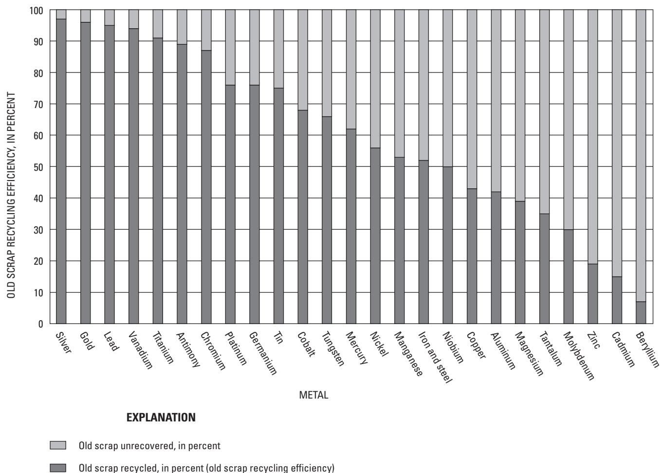
Figure 4. Bar graph showing old scrap recycling efficiency for metals studied for chapters A–Z of U.S. Geological Survey Circular 1196 (table 1). Each bar has data for a single base year, which is 1998, 2000, or 2004. The old scrap recycling efficiency values and base years from the chapters are summarized in table 2 of this chapter AA; a recycling efficiency value is not available for one metal (selenium). The old scrap available to be recycled (100 percent) is shown as old scrap recycled, in percent (old scrap recycling efficiency), plus old scrap unrecovered, in percent.
