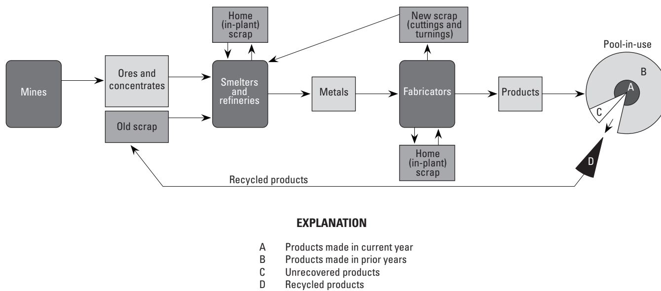
Figure 1. Generalized metals recycling flow chart. Flow charts for all of the metals in the study follow this general outline.
