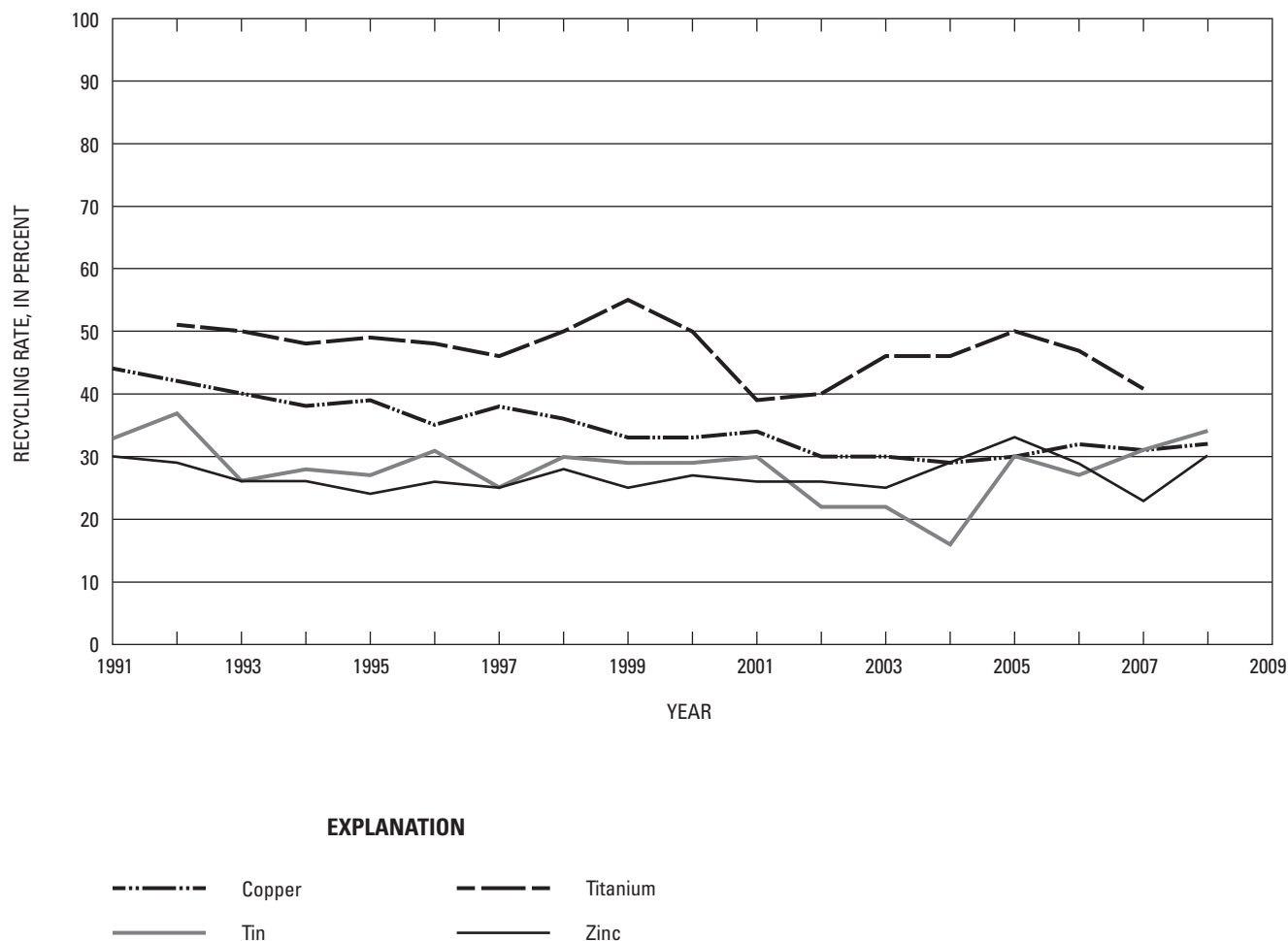
Figure 7. Graph showing declining or stagnant recycling rates for four metals in the United States in 1991 through 2008. Data sources: U.S. Geological Survey (1997–2006) and Papp (2007–2010).
