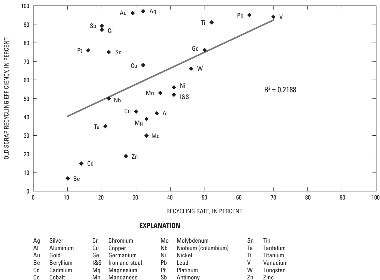
Figure 5. Scatter diagram of old scrap recycling efficiency versus recycling rate for 24 metals and base years of 1998, 2000, and 2004; see figures 3 and 4. The plot suggests a weak correlation. R^2 , or the square of the correlation coefficient, is a measure of how well the data fit a pattern or trend, in this case, a straight-line regression analysis, where 1 is the highest value possible and would represent the best fit. The value of R^2 for these data is 0.2188.
