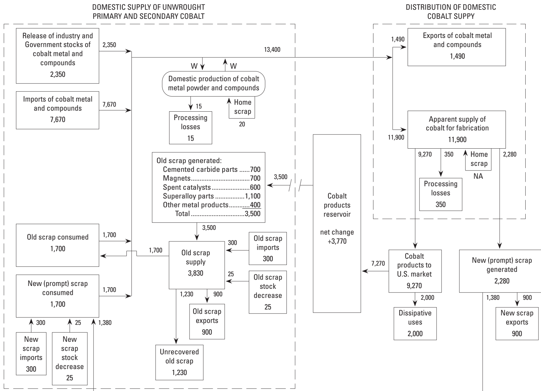
Figure 2. Example of a typical detailed flow chart showing the materials flow of cobalt in the United States in 1998. For some metals, detailed information like that shown for cobalt is not available. Values are in metric tons of contained cobalt, are rounded to no more than three significant digits, and may not add to totals shown. NA, not available; W, withheld to avoid disclosing company proprietary data. Source: Shedd (2006, fig. 1).
