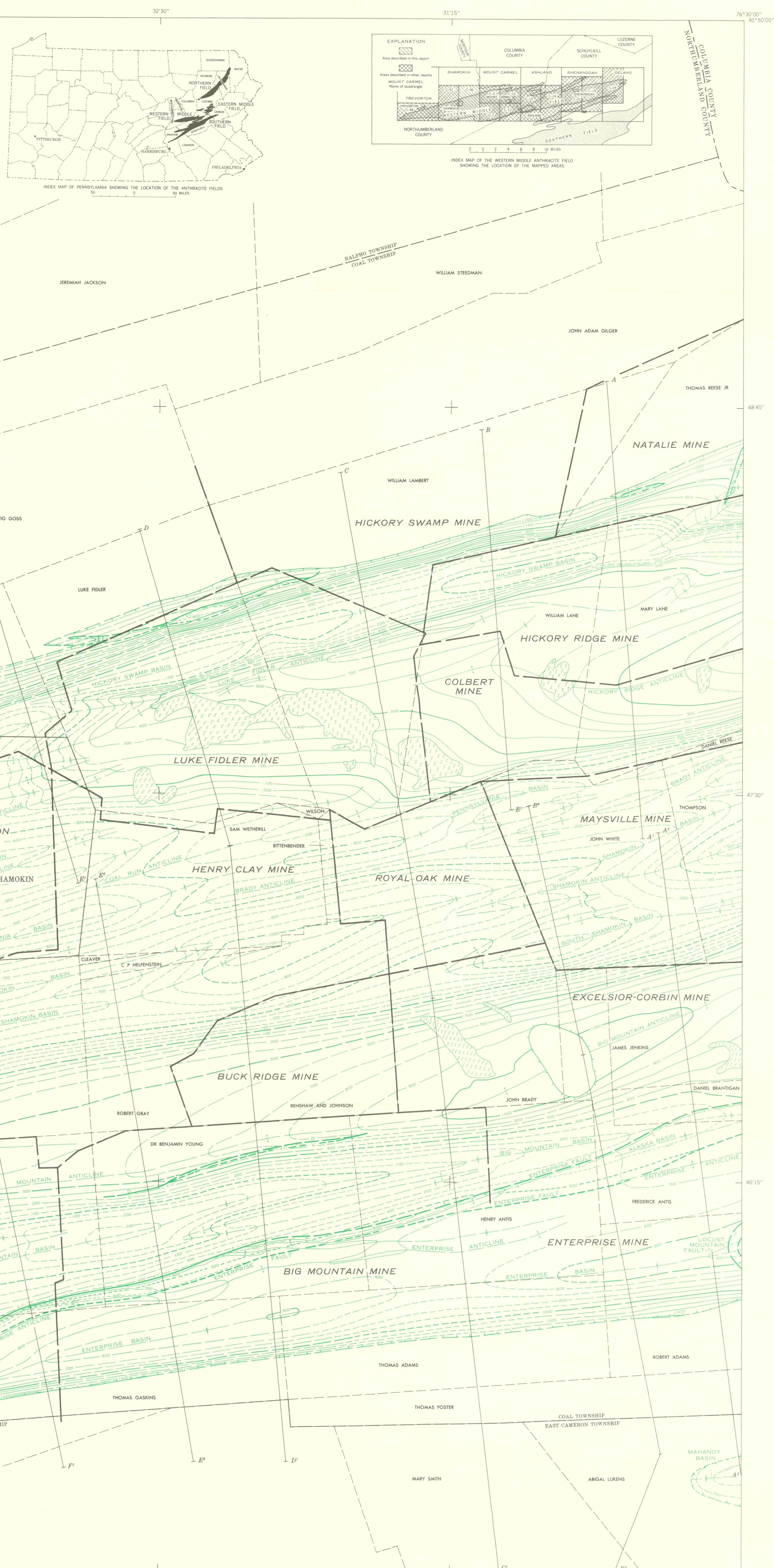
STRUCTURE CONTOUR MAP OF THE BUCK MOUNTAIN COAL BED
