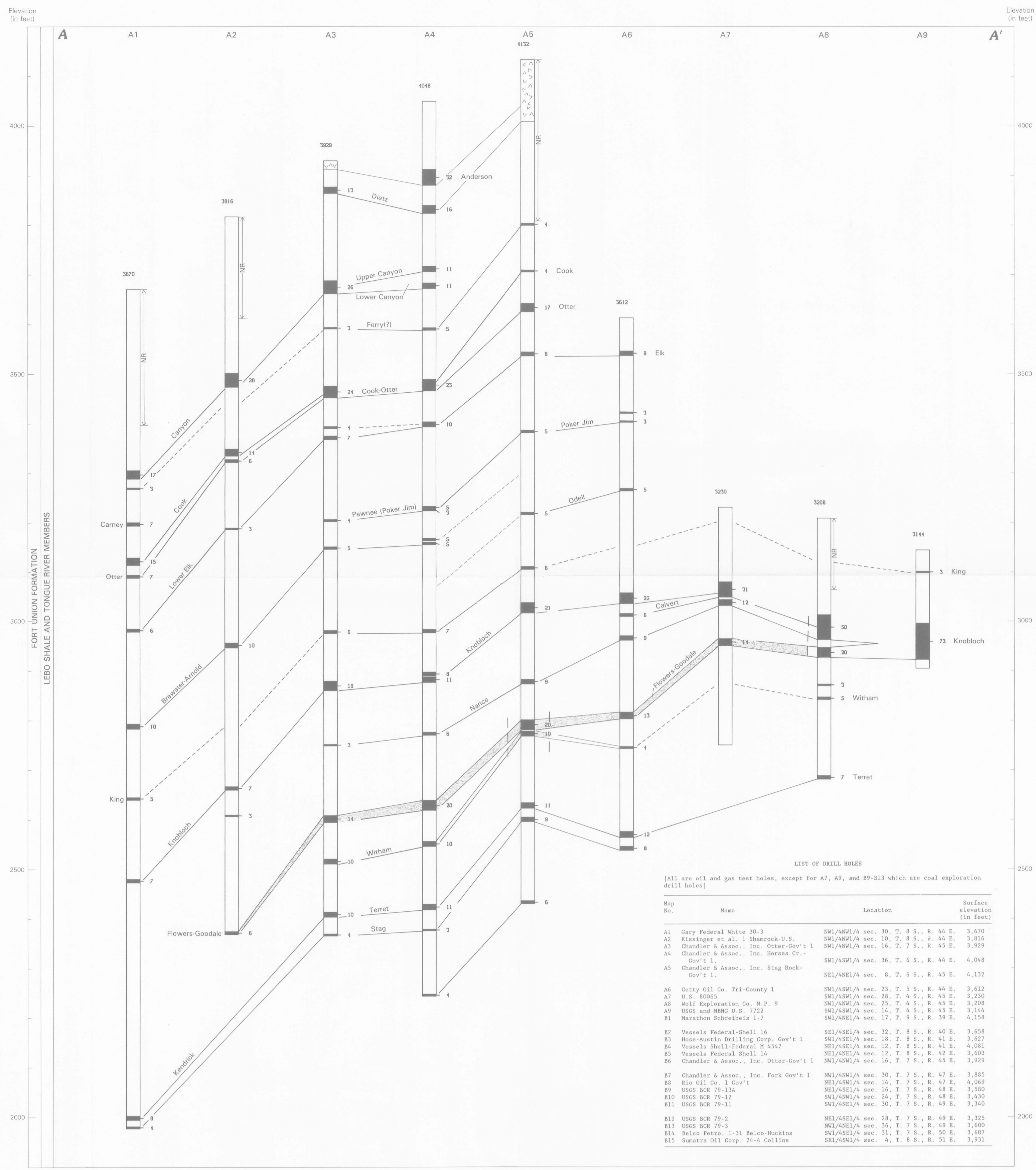
CORRELATION DIAGRAM OF THE FLOWERS-GOODALE COAL RESOURCE UNIT AND ASSOCIATED COAL BEDS ALONG A-A'
