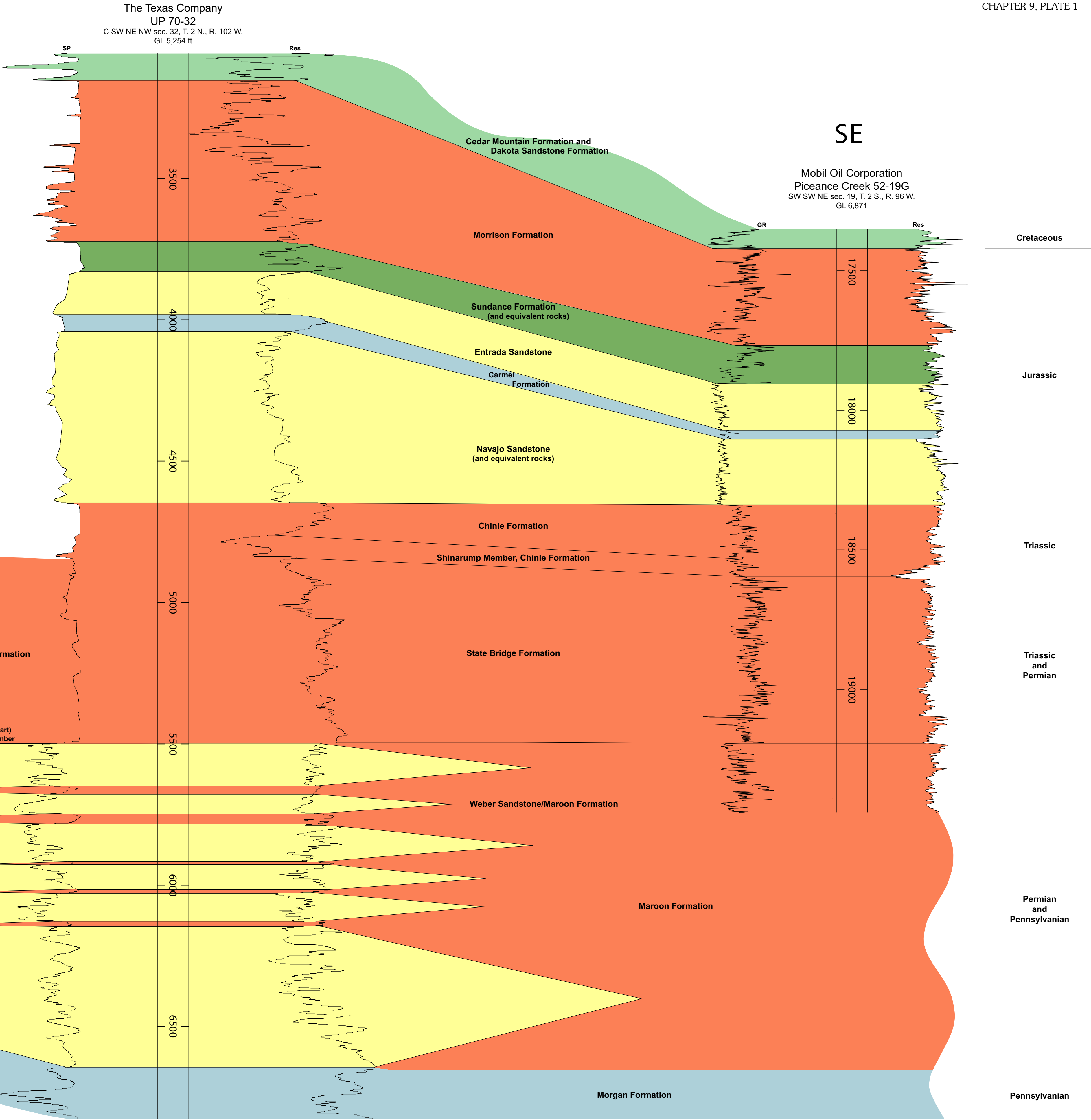
SUBSURFACE STRATIGRAPHIC CROSS SECTION SHOWING THE WEBER SANDSTONE–MAROON FORMATION FACIES TRANSITION, NORTHEAST UTAH TO NORTHWESTERN COLORADO
