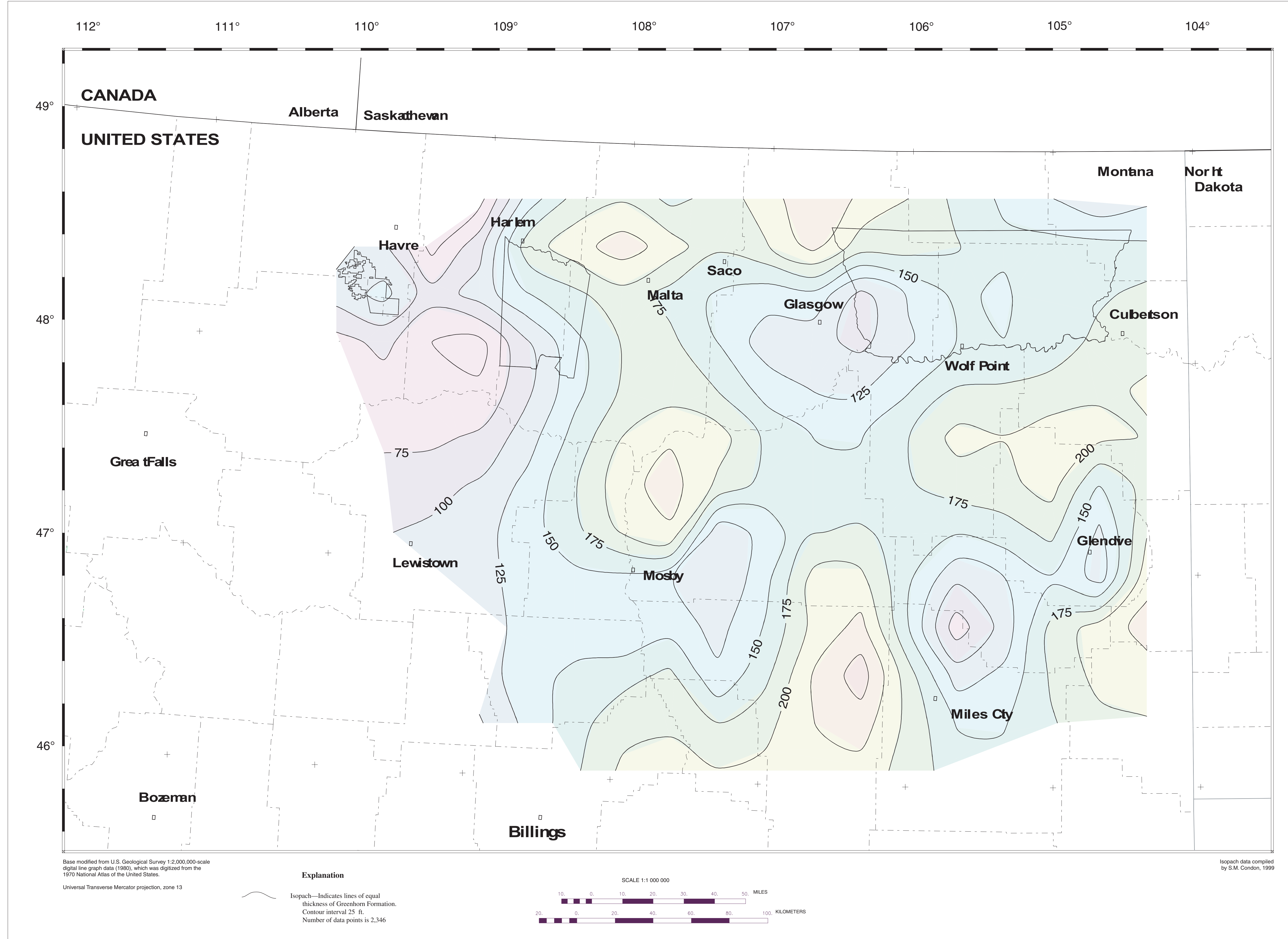
ISOPACH MAP OF THE GREENHORN FORMATION STRATIGRAPHIC FRAMEWORK OF LOWER AND UPPER CRETACEOUS ROCKS IN CENTRAL AND EASTERN MONTANA By Steven M. Condon 2000
