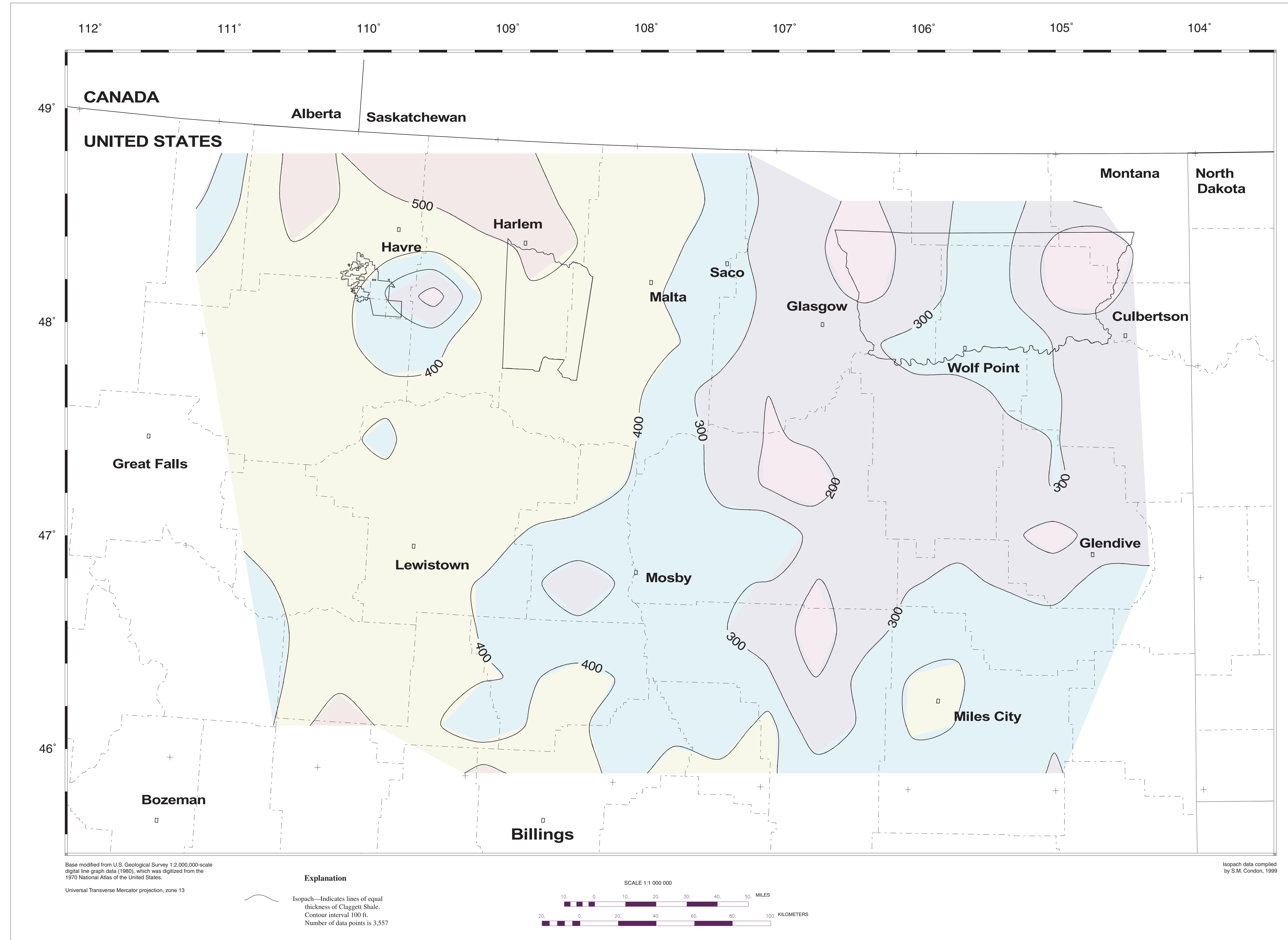
ISOPACH MAP OF THE CLAGGETT SHALE STRATIGRAPHIC FRAMEWORK OF LOWER AND UPPER CRETACEOUS ROCKS IN CENTRAL AND EASTERN MONTANA By Steven M. Condon 2000
