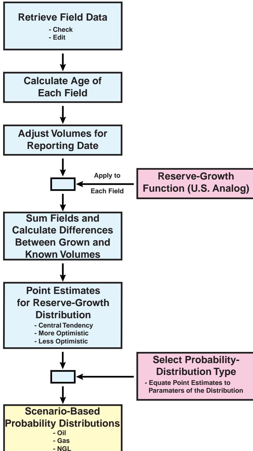
Figure RG-3. Simplified flow diagram emphasizing the basic steps used to obtain a forecast of world potential reserve growth for the USGS World Petroleum Assessment 2000.
