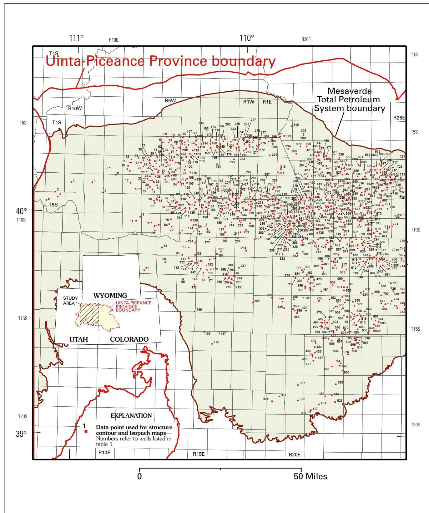
Figure 1. Study area and approximate locations of wells examined in this report. Due to the proprietary nature of exact locations, wells are plotted in the center of the quarter sections in which they were drilled. Location of study area shown on insert map.
