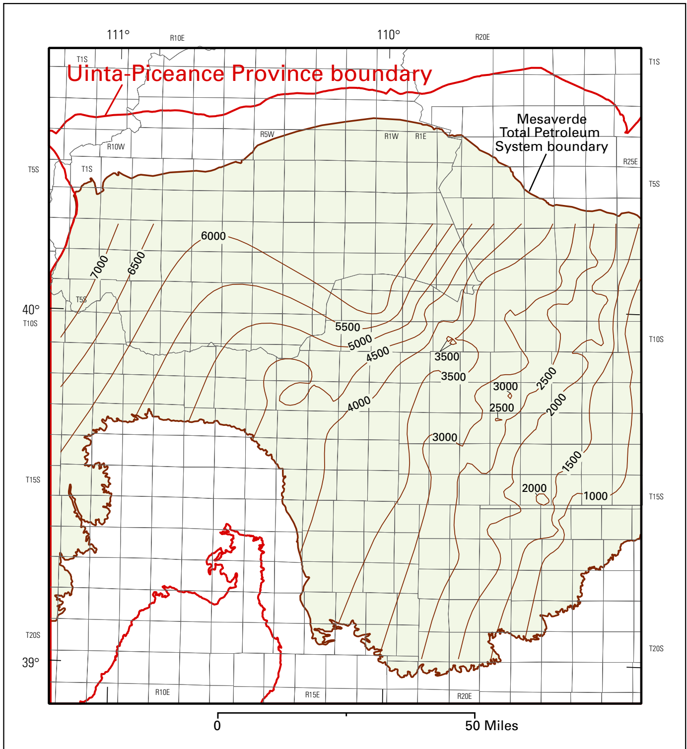
Figure 8. Isopach map of the interval from the top of the Upper Cretaceous Mesaverde Group to the base of the Long Point Bed of the Eocene Green River Formation. Contour interval 500 ft.
