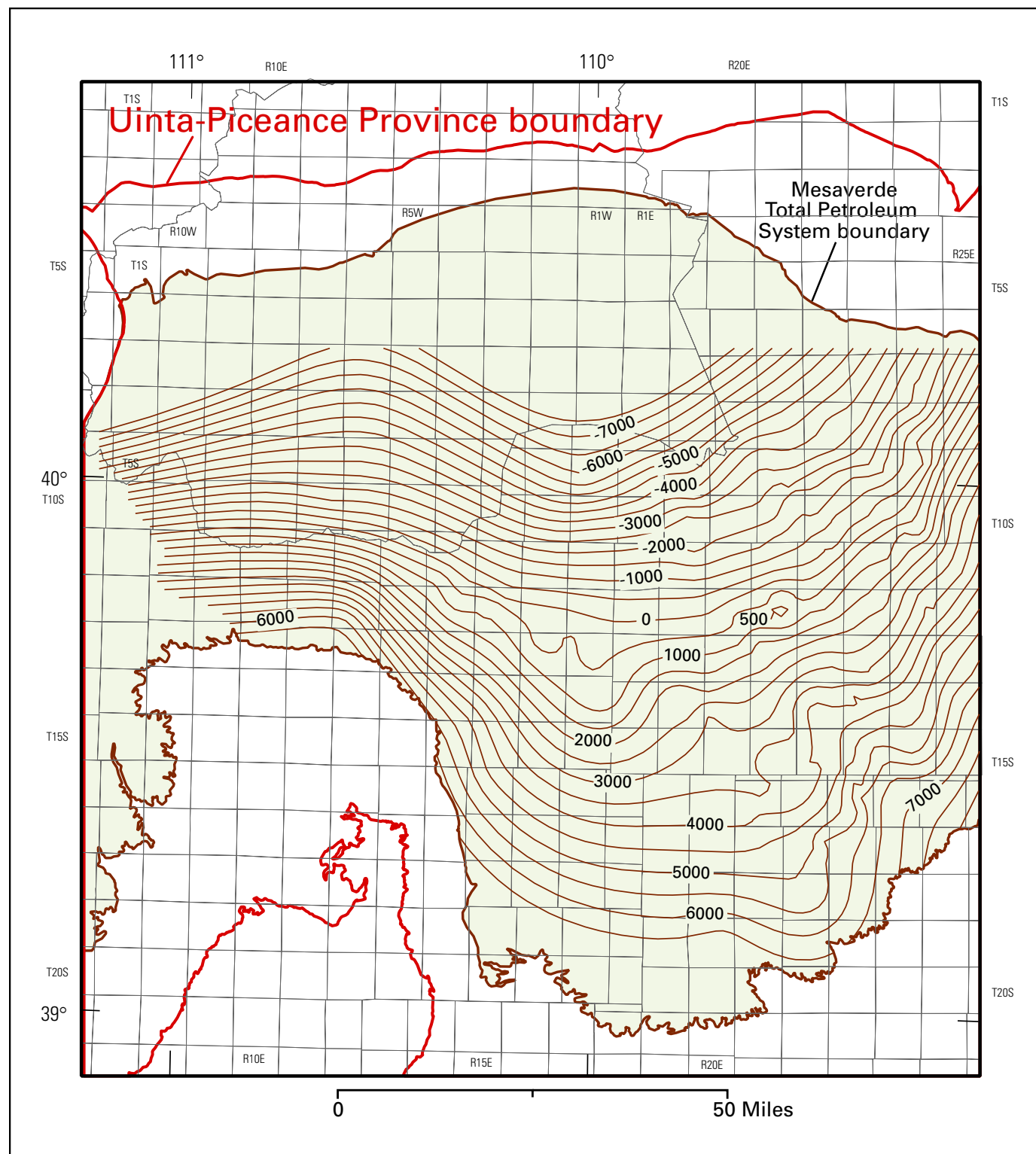
Figure 4. Structure contour map on the top of the Upper Cretaceous Mesaverde Group. Contour interval 500 ft.
