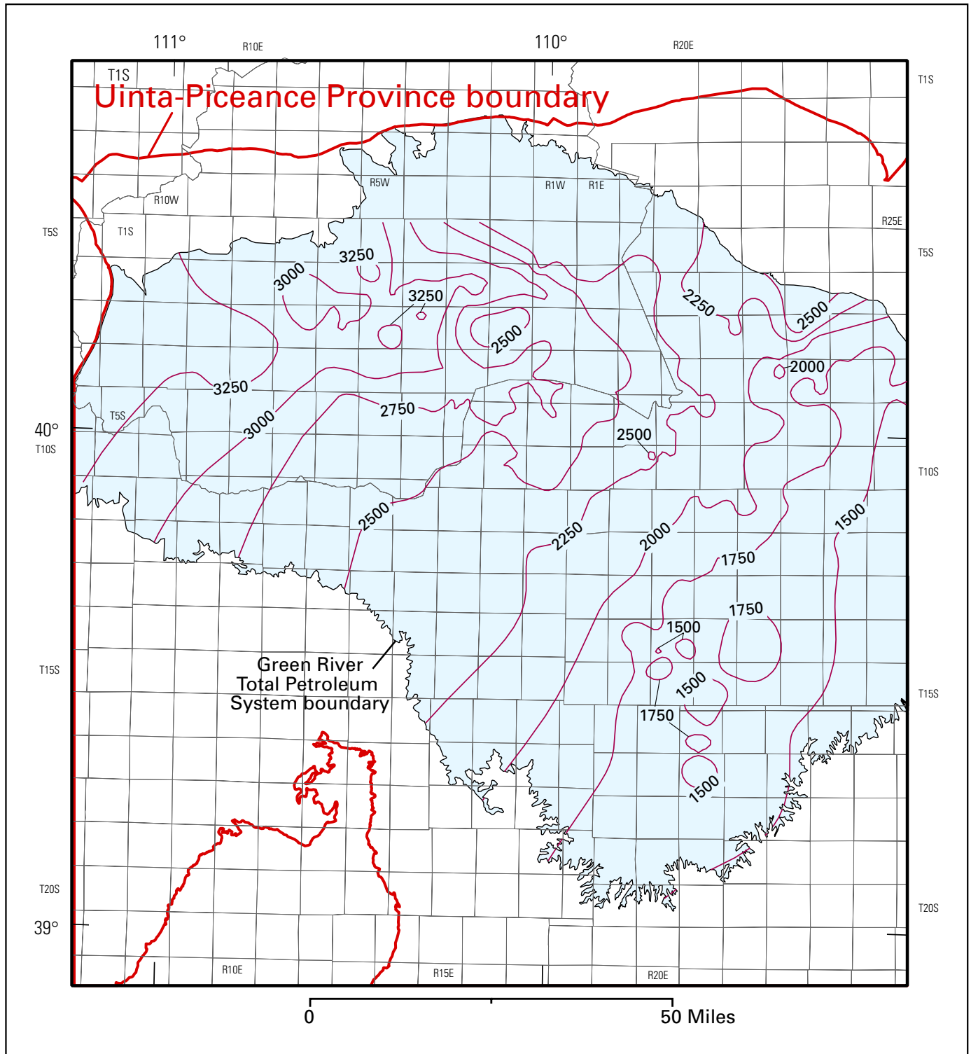
Figure 9. Isopach map of the interval from the base of the Long Point Bed of the Eocene Green River Formation to the top of the Mahogany oil-shale bed of the Eocene Green River Formation. Contour interval 250 ft.
