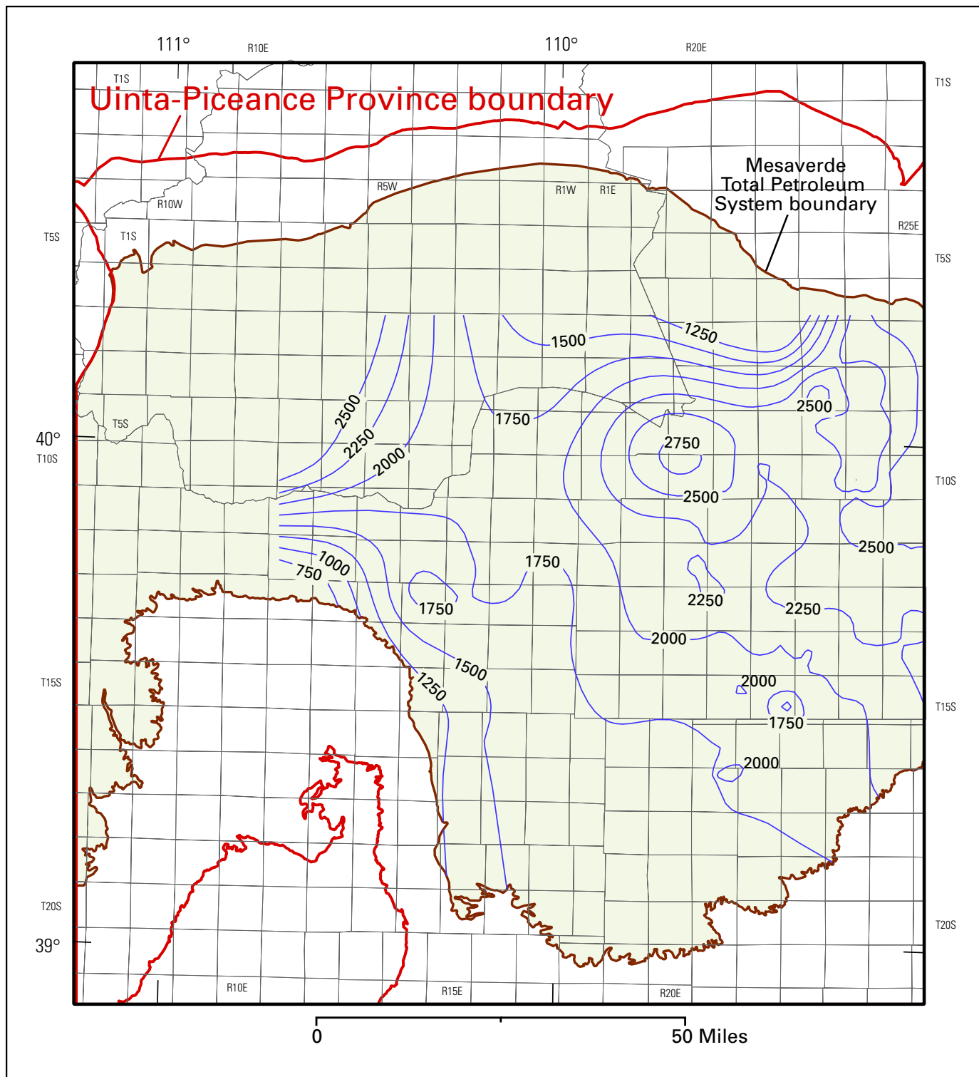
Figure 7. Isopach map of the interval from the top of the lower tongue of the Upper Cretaceous Castlegate Sandstone to the top of the Upper Cretaceous Mesaverde Group. Contour interval 250 ft.
