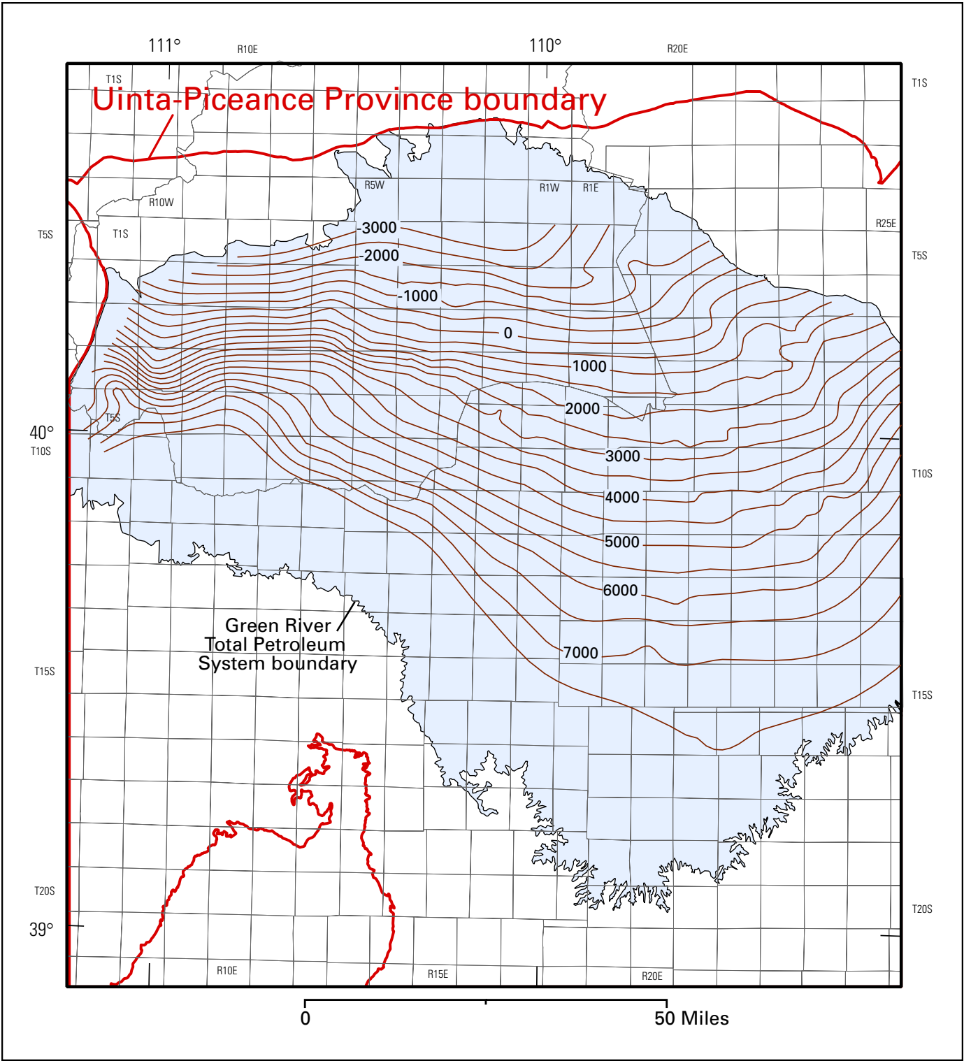
Figure 6. Structure contour map on the top of the Mahogany oil-shale bed of the Eocene Green River Formation. Contour interval 500 ft.
