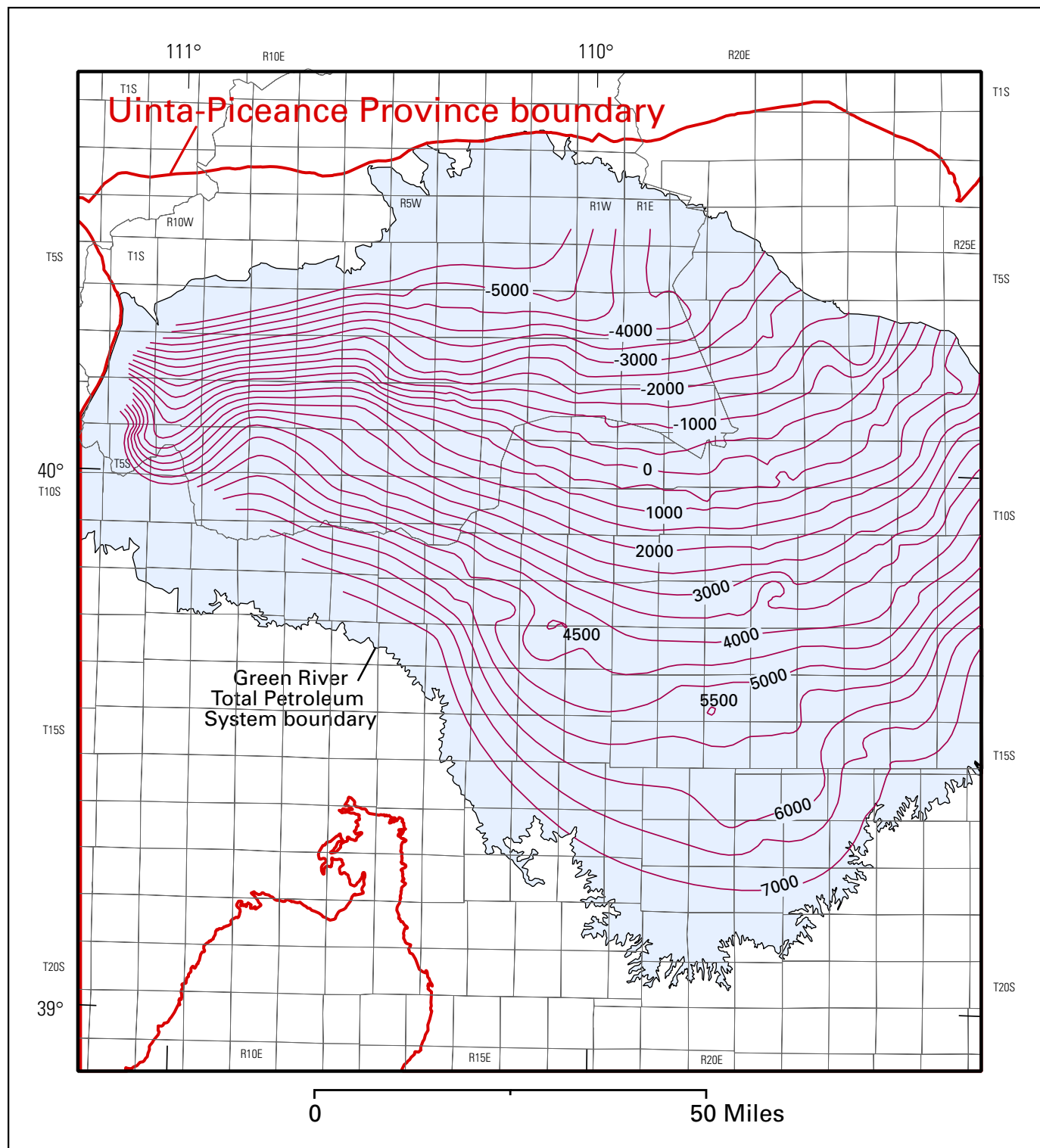
Figure 5. Structure contour map on the base of the Long Point Bed of the Eocene Green River Formation. Contour interval 500 ft.
