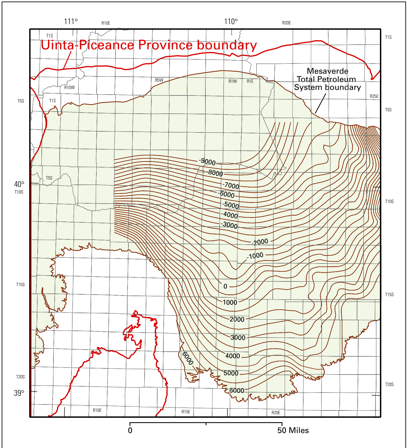
Figure 3. Structure contour map on the top of the lower tongue of the Upper Cretaceous Castlegate Sandstone. Contour interval 500 ft.
