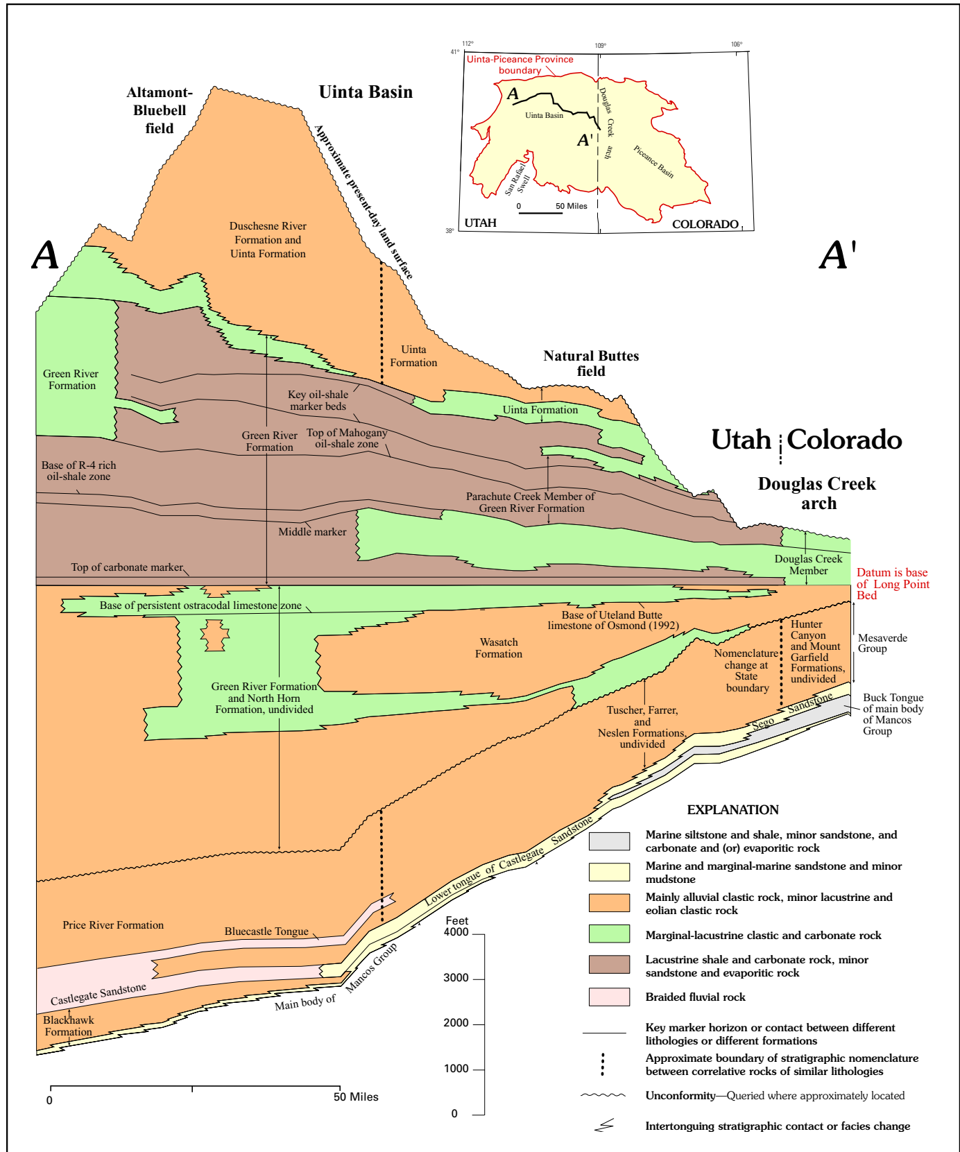
Figure 2. Generalized stratigraphic cross section showing Upper Cretaceous and lower Tertiary rocks in the Uinta Basin, Utah. Modified from Johnson and Johnson (1991). Location of cross section shown on inset map.
