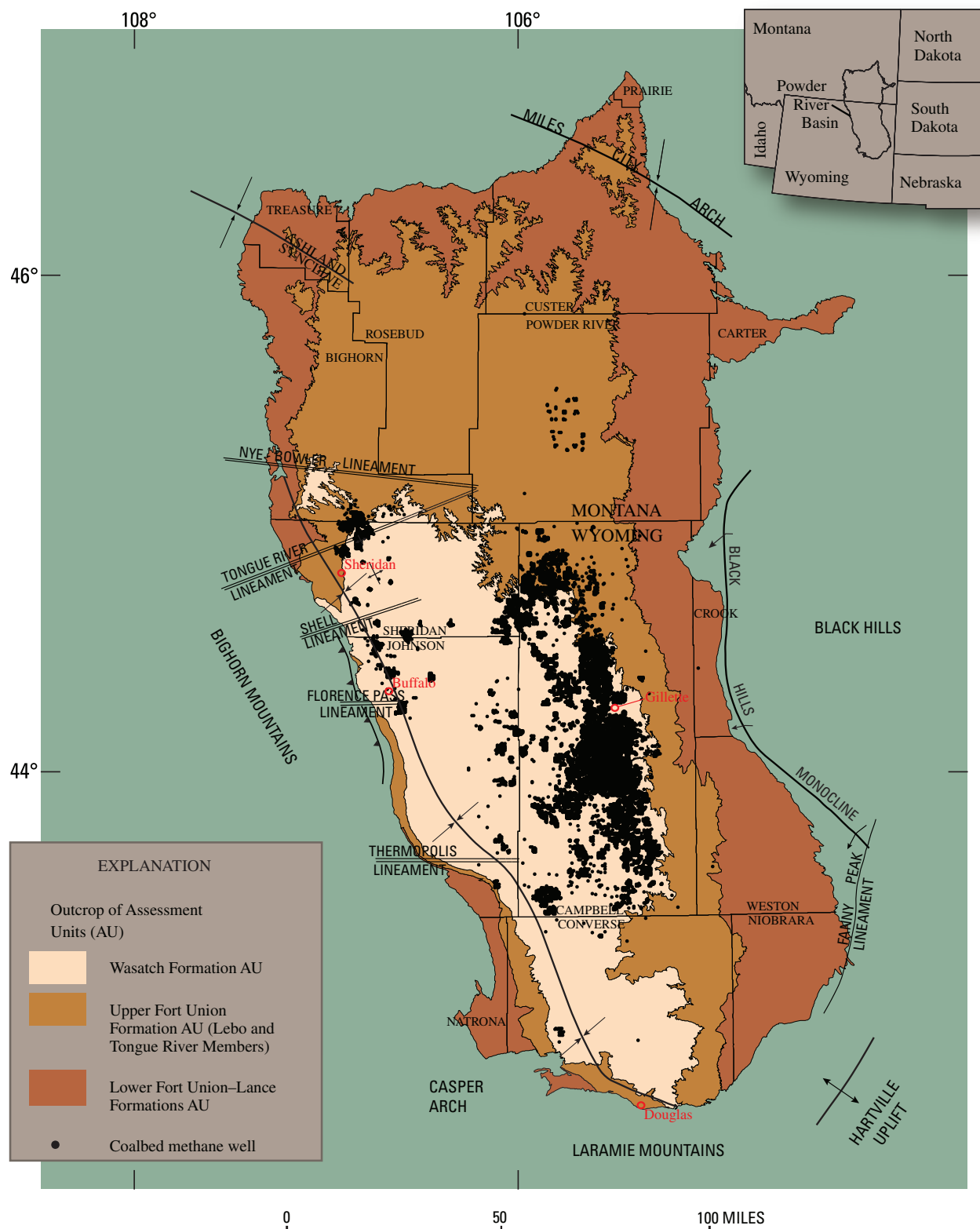
Figure 8. Map showing the assessment units of the Tertiary-Upper Cretaceous Coalbed Methane Total Petroleum System, major structural elements, and distribution of coalbed methane wells in the Powder River Basin and adjoining areas in Wyoming and Montana.
