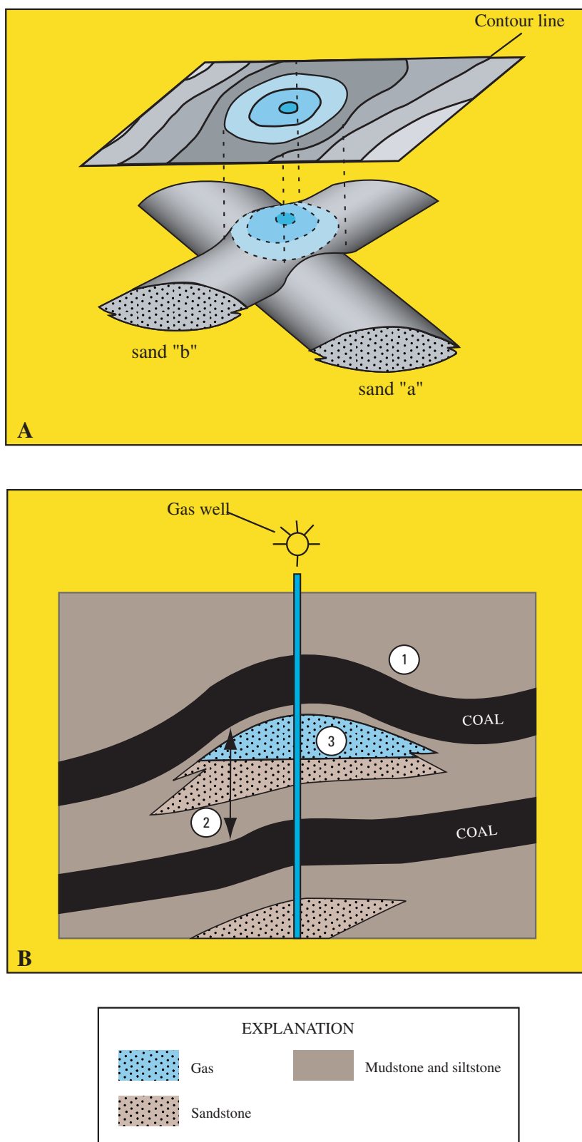
Figure 20. Diagrams A and B showing sandstone reservoirs "a" and "b" and compaction structure above the sandstone reservoirs in the Eastern Basin Margin Upper Fort Union Sandstone Assessment Unit. Diagram A shows enhancement of closure on a compactional trap in stacked sandstone reservoirs. Not shown between the sandstone reservoirs is interbedded coal and fine-grained sediments. Diagram B shows (1) a compaction model with a structural closure, (2) increased noncoal interval (arrow) below the upper coalbed, and (3) gas-saturated top of the sandstone. Modified from Oldham (1997).
