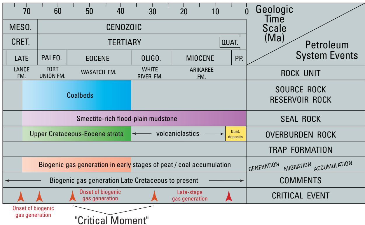
Figure 40. Events chart showing timing of elements and processes related to coalbed methane generation and accumulation in the Wasatch Formation, Upper Fort Union Formation, and Lower Fort Union-Lance Formations Assessment Units of the Powder River Basin, Wyoming and Montana. PP. = Pliocene-Pleistocene; FM. = Formation; Ma = million years. Arrows show onset of gas generation.
