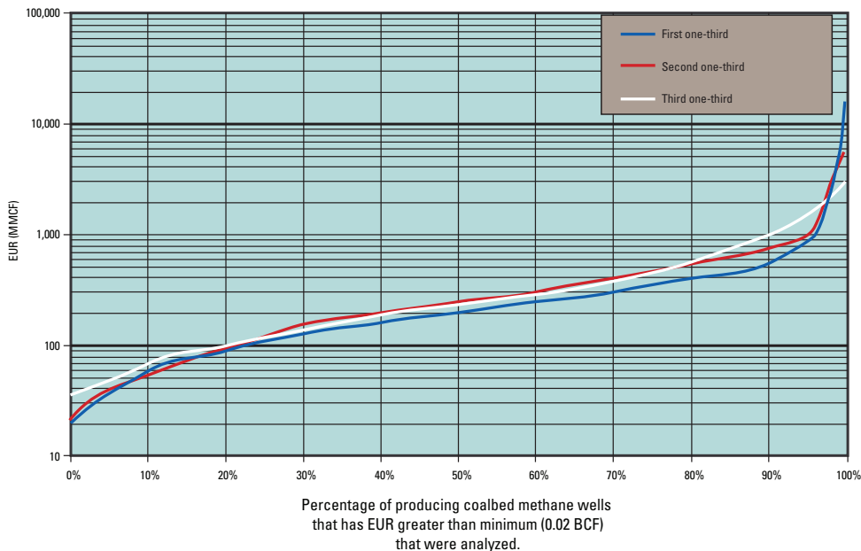
Figure 29. Estimated ultimate recovery distributions for coalbed methane wells in the first, second, and third one-thirds analyzed in the Upper Fort Union Formation Assessment Unit in the Powder River Basin, Wyoming (EUR, estimated ultimate recovery; MMCF, million cubic feet; BCF, billion cubic feet).
